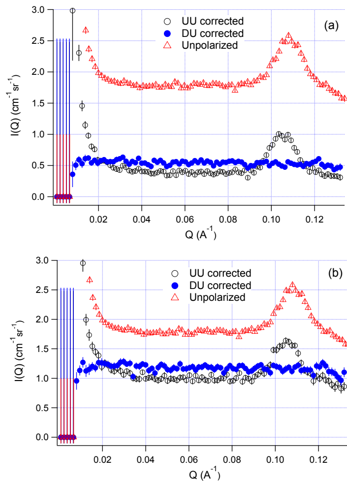
Figure 3. Color online. Polarization efficiency corrected, radially averaged data on an absolute scale ( \text{cm}^{-1}\text{sr}^{-1} ) for a sample of 0.5 mm-thick silver behenate back filled with 1 mm-thick light water for (a) the elastic data only and (b) both elastic and inelastic data. Non spin-flip data \sigma^{\text{uu}} are shown in black open circles; spin-flip data \sigma^{\text{du}} are shown in blue solid circles. Unpolarized data (red open triangles) are also shown for comparison. All uncertainties given in the paper represent one standard deviation.
