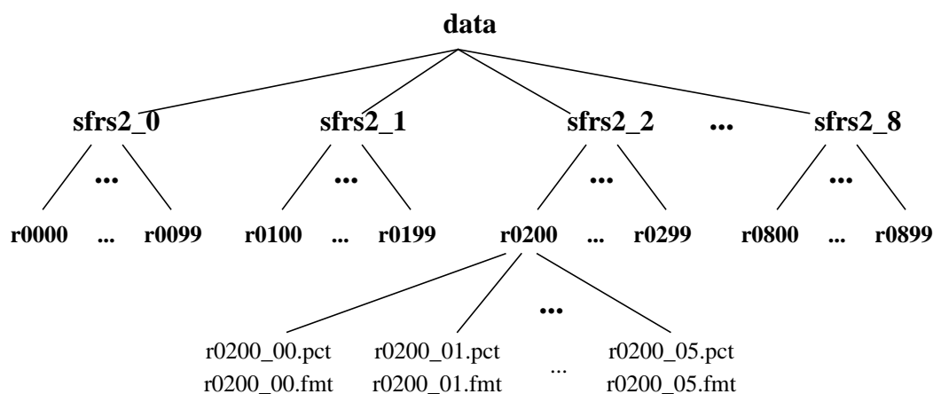
FIGURE 14. The file organization of the form images and format files contained in NIST Special Database 6 .
