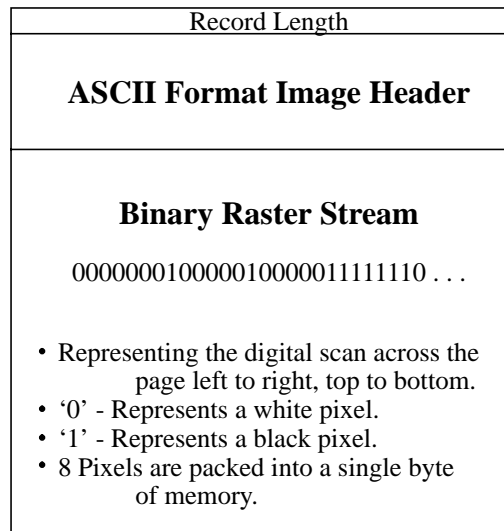
FIGURE 5. An illustration of the IHead raster file format.
