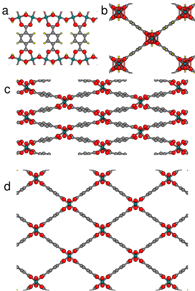
FIG. 1. Structure of MIL-53(Cr). Cr atoms green, O red, C gray, and H yellow. (a) bdc linkers joining zigzag Cr-OH-Cr-... chains. (b) Each zigzag chain is coordinated with four neighboring chains; each Cr is octahedrally coordinated with six O. (c) Narrow pore ( np ) phase showing bdc rotations. (d) Large pore ( lp ) phase. In (c) and (d), the H are not shown.
