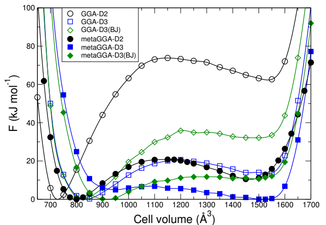
FIG. 4. Calculated Helmholtz free energy for MIL-53(Cr) at 293 K as a function of volume for different density functionals. Each curve is scaled so that its minimum is zero. The effect of atmospheric pressure of about 0.1 MPa is negligible on this scale.
