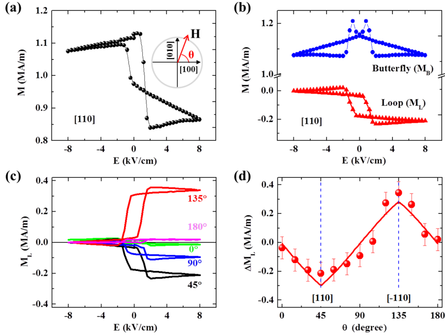
Figure 1. Macroscopic magnetization controlled by electric field. (a) M - E curves measured at 300 K along the [110] direction with a 1 mT external magnetic field. A simplified version of the crystal axes, magnetic field ( H ), and the angle \theta is shown in the inset. (b) The looplike ( M_L , red triangles) and butterfly-like ( M_B , blue circles) electric-field-controlled magnetization ( M - E ) hysteresis curves obtained from panel a. (c) Angle dependence of M_L - E curves obtained with steps of 45^\circ at 300 K. (d) Angle dependence of the nonvolatile manipulation magnitude \Delta M_L and the fitting curve (red line, Supporting Information S7). The error bars in panel d are the standard error derived from multiple measurements, which includes error in the sample alignment for each measurement. Error bars in panels a-c are smaller than the point markers.
