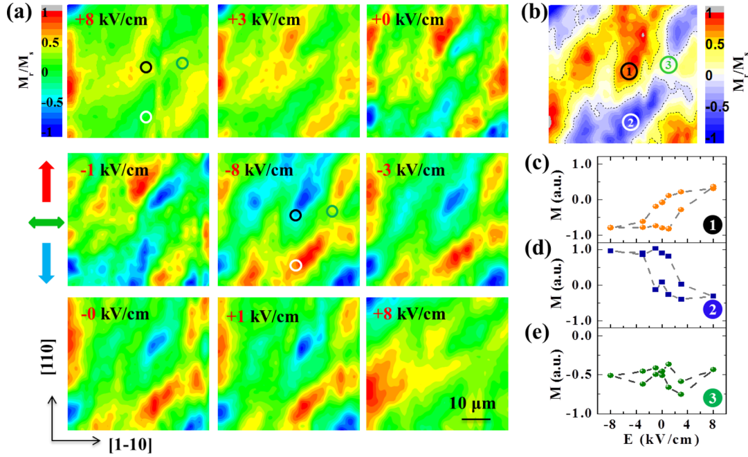
Figure 2. Electric field control of magnetism with SKM. (a) Scanning MOKE maps of M_t/M_s in a 50 \times 50 \mu\text{m}^2 area under different static electric fields. The in-plane longitudinal MOKE was aligned to the [110] direction of PMN-PT substrates. The colored arrows at the left represent the different magnetic moment orientations. (b) The difference of SKM images under \pm 8 \text{ kV cm}^{-1} ( M_{+8} - M_{-8} ) deduced from panel a. The dotted lines are a guide for the eye to distinguish three types of contrasts. (c-e) The local static electric-field-controlled magnetization ( M-E ) curves for the different regions numbered in panel b. The uncertainty in the measurement is smaller than the point size.
