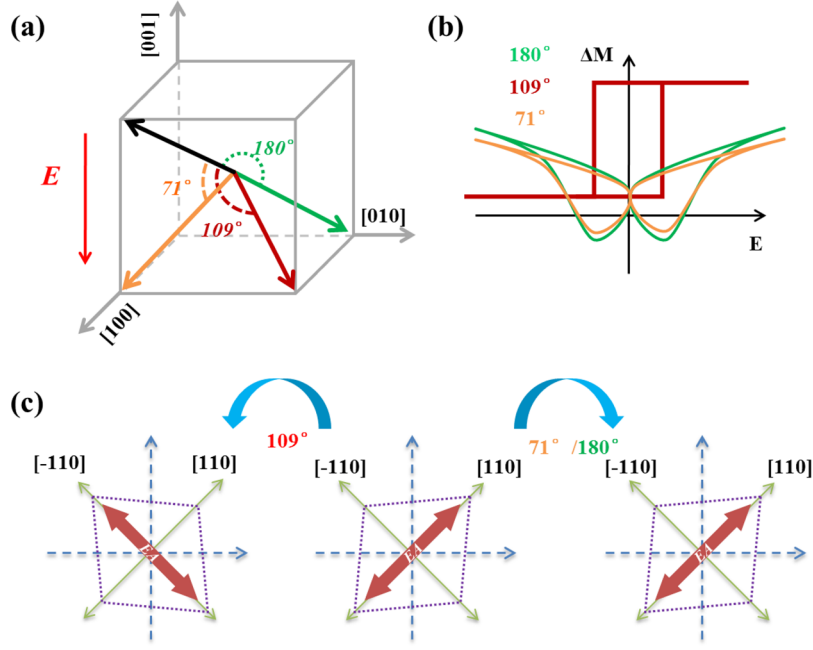
Figure 4. Schematic of the FE-domain-switching-controlled magnetism. Schematic of (a) three FE domain switching processes of PMN-PT and (b) picture of the related M - E curves. (c) The top view looking down [001] of distortions and related in-plane magnetic easy axes (EA, red arrows) for the different FE domain switching processes, starting from a FE polarization along the [111] direction.
