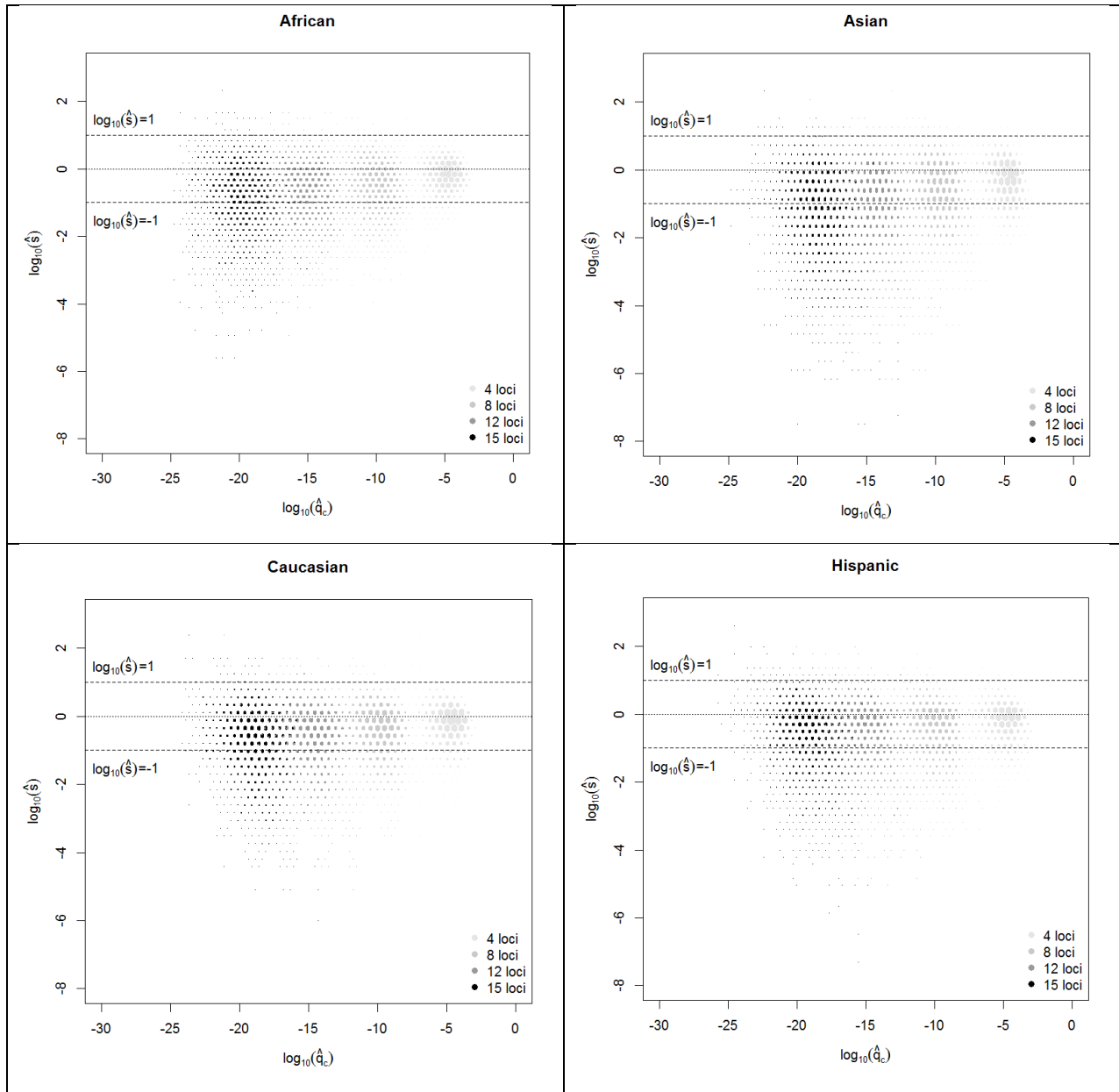
Fig. 1: Results of Experiment 1a. Each database within a cluster serves as the cognate database to simulate 400 profiles. Ratio \hat{s} is obtained for each non-cognate database within the cluster. The graphs show the plots of the log of \hat{s} in function of the log of \hat{q}_c for the African, Asian, Caucasian and Hispanic clusters.
