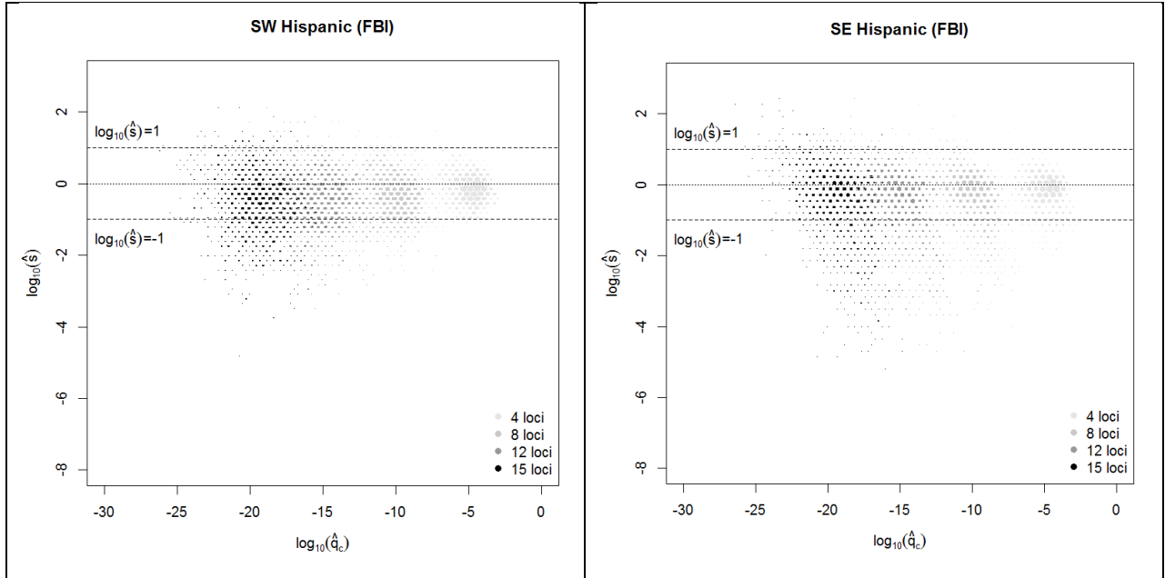
Fig. 2: A selection of results of Experiment 1b. Each database within a cluster, with the exception of the FBI and NIST databases, serves as the cognate database to simulate 400 profiles. Ratio \hat{s} is obtained for the cluster's FBI and NIST databases, respectively. The graphs show the plots of the log of \hat{s} in function of the log of \hat{q}_c for the African, Asian, Caucasian and Hispanic clusters (note that the FBI has two Hispanic databases: one for Southwest (SW) Hispanics and one for Southeast (SE) Hispanics). Additional results are presented in Supplementary Fig. 1.
