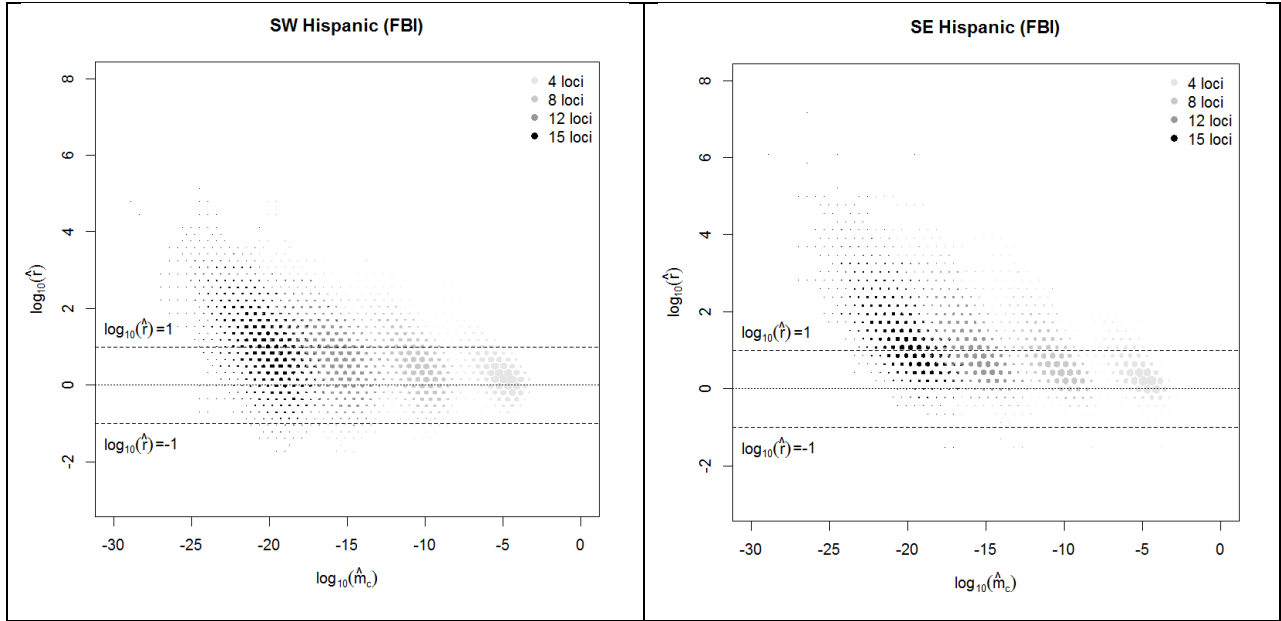
Fig. 4: A selection of results of Experiment 2. The cognate databases are all the databases within a cluster, with the exception of that ethnic group's FBI and NIST databases. Their match probabilities, \hat{m}_c , are obtained using the product rule. The non-cognate database is the cluster's FBI or NIST database. The match probability, \hat{m}_{\bar{c}} , is obtained using NRC II recommendation 4.2. The graphs show the plots of the log of \hat{r} in function of the log of \hat{m}_c for the African, Asian, Caucasian and Hispanic clusters (note that the FBI has two Hispanic databases: one for Southwest (SW) Hispanics and one for Southeast (SE) Hispanics). Additional results are presented in Supplementary Fig. 2.
