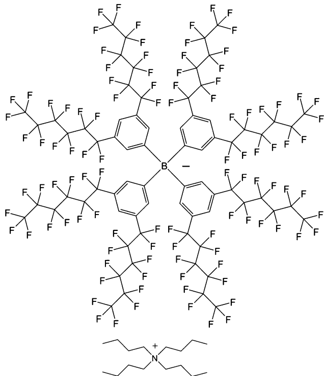
Fig. 1 Tetra- n -butylammonium tetrakis[3,5-bis(perfluorohexyl)phenyl]borate.
