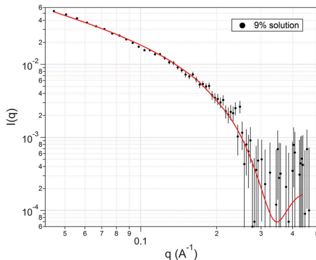
Fig. 2 The SANS scattering curve for the 9% solution and the best fitting curve of the core-shell model. The uncertainties ( \pm\sigma ) are for the counting statistics only.
