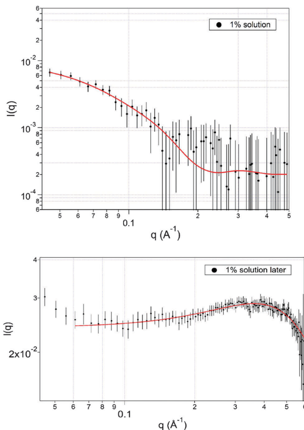
Fig. 4 The SANS scattering curves of the 1% TBA-borate solution a few days after mixing (top) and after more than a month of equilibration (bottom). The uncertainties ( \pm\sigma ) are for the counting statistics only.
