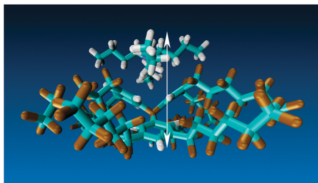
Fig. 5 Image of a solitary ion pair from the eight-pair model. The arrow length is 9.9 \text{\AA} . Note the pairings of the sidechains from different rings.
