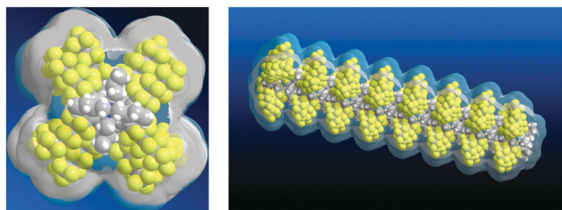
Fig. 3 The molecular structure of a model eight ion pairs in length of the TBA-borate complex shown end on (left) and lengthwise, both showing the limits of solvent accessibility (grey cloud) for a static structure. Even for the static structure, the solvent can penetrate only slightly past the outer edge. That, together with flexibility at the ends of the chains, reduces the apparent diameter for the scattering.
