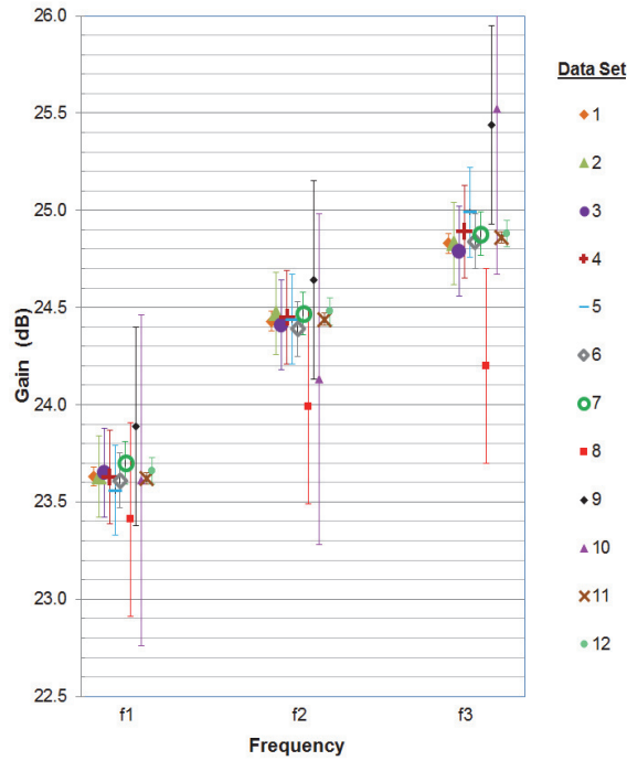
Fig. 1. On-axis gain value.
