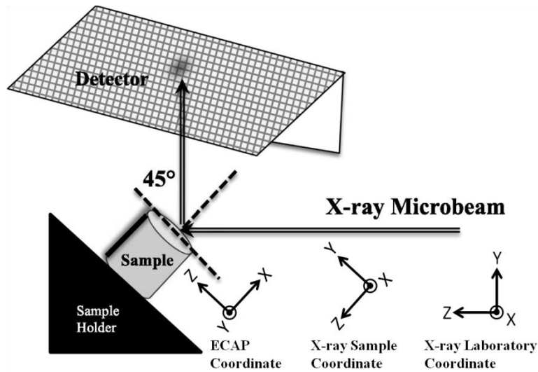
Figure 1. The X-ray microbeam procedure [7] and the various coordinate systems. The ECAP, X-ray Laboratory, and X-ray Sample coordinate systems are shown in relation to the ECAP sample. The x-direction points out of the page for the X-ray sample and laboratory coordinate systems; the y-direction points out of the page for the ECAP coordinate system. Note that the ECAP coordinate system uses a "left-handed" convention while the X-ray Laboratory and Sample coordinate system use a "right-handed" convention.
