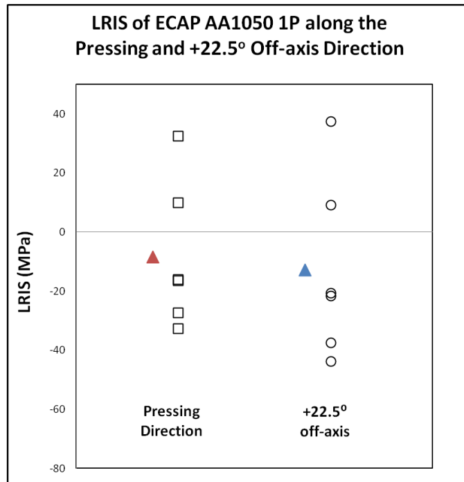
Figure 6. Long range internal stresses along the pressing and +22.5^\circ off-axis directions of ECAP AA1050 sample after 1 pass. Average values are plotted as solid triangles to the left of the elastic strain values.
