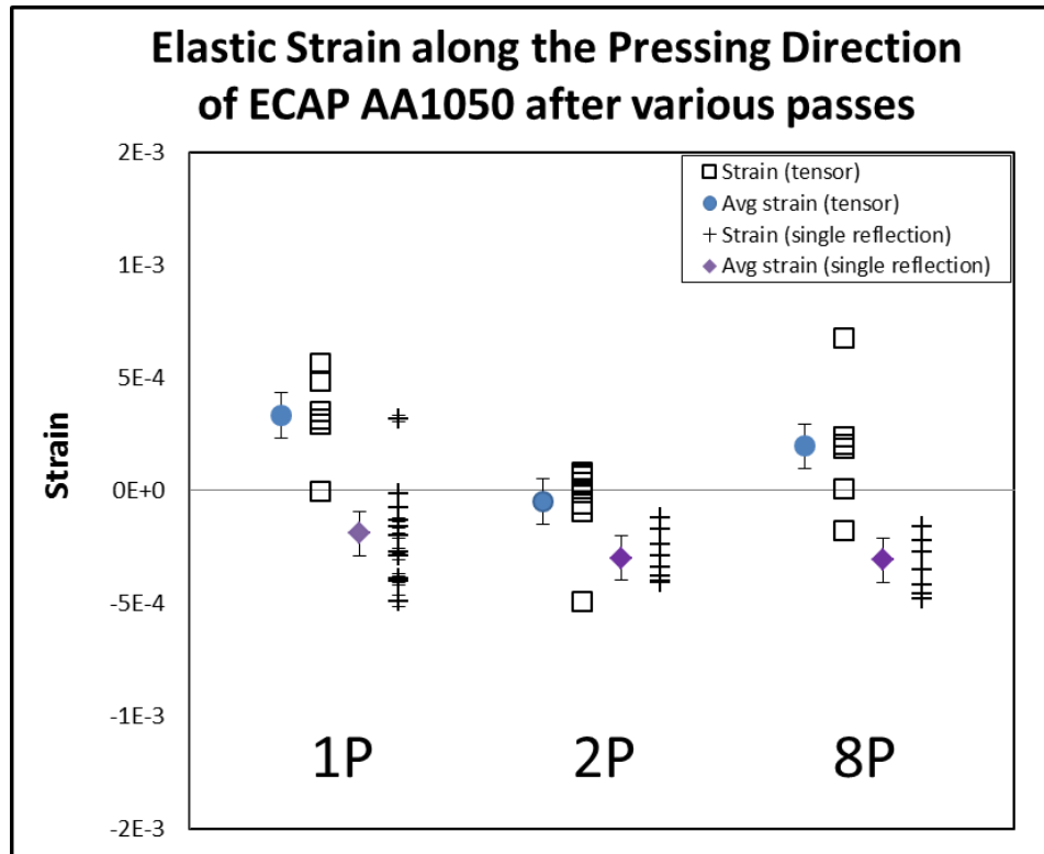
Figure 7. Elastic strain along the pressing direction for ECAP AA1050 grain/subgrain interiors calculated by tensor analysis and single reflection measurements after 1, 2, and 8 passes. Average elastic strains are plotted to the left of the strain values as solid dots for the tensor calculated values and solid diamonds for the single reflection values from previous works [8].
