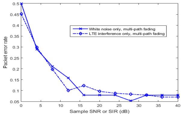
Fig 3. Packet error rate vs. SNR of the IEEE 802.11a signal, affected by white noise and LTE interferences, respectively.
