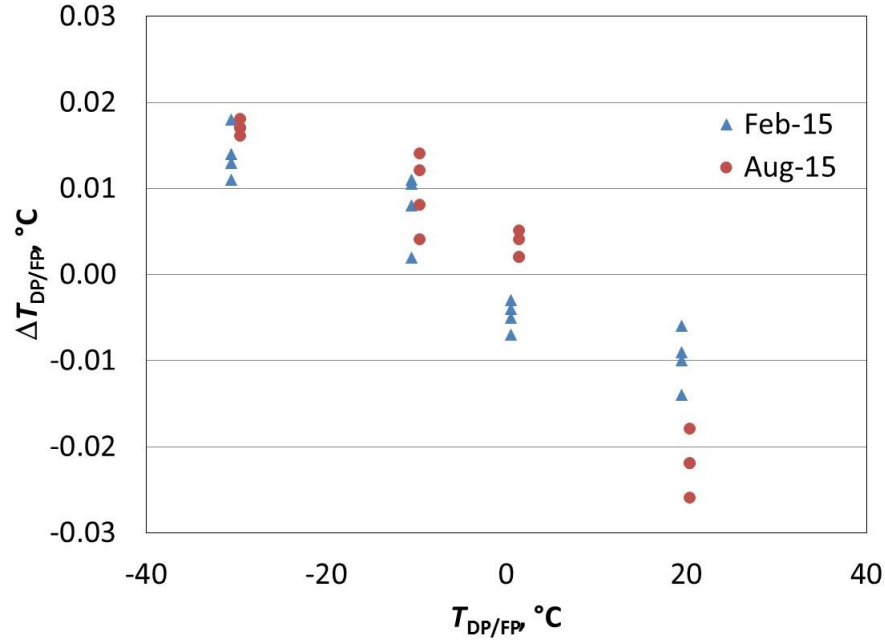
Figure 3. Difference between the LACOMET generator/hygrometer comparisons performed in February 2015 and in August 2015. The values of T_{DP/FP} have been slightly offset to aid the viewer.
