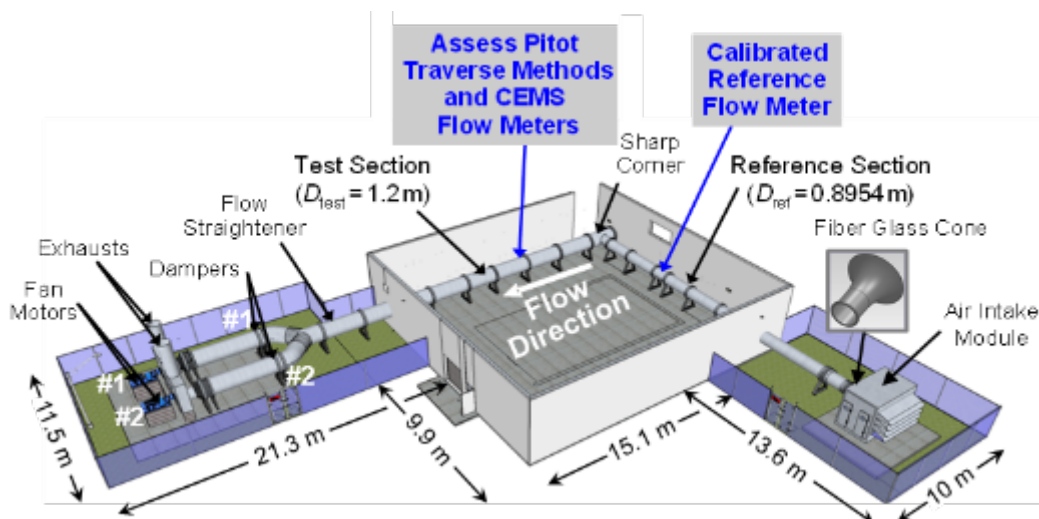
Figure 7. Schematic of NIST Scale-Model Smokestack Simulator (SMSS). A calibrated flow meter in the reference section is used to assess both the EPA RATA and a CEMS flow meter installed in the 1.2 m diameter test section. The sharp corner introduces swirling, asymmetric flow in the test section that is similar to the complex flow conditions in an industrial-scale smokestack. ( http://www.nist.gov/pml/div685/grp02/scale-model-smokestack.cfm )
