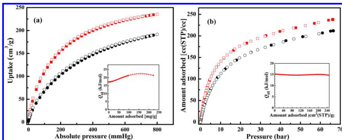
Figure 3. Gas sorption isotherms of ZJU-70a for (a) C_2H_2 at 273 and 298 K and (b) high-pressure CH_4 at 273 and 298 K. Inset: Isosteric heats of adsorption of C_2H_2 and CH_4 calculated using the virial method. Solid symbols: adsorption, open symbols: desorption.
