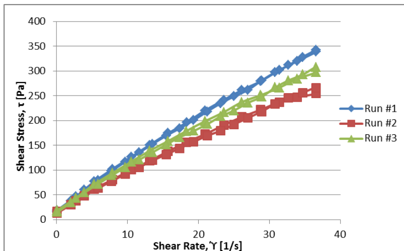
Figure B-30: 7 Day values for Mix J (NIST Code: SR-97)
