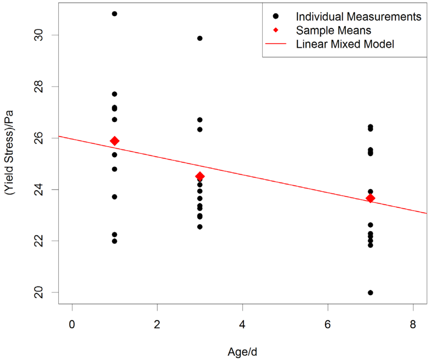
Figure A-4: Yield Stress versus Age with Linear Mixed Model.
