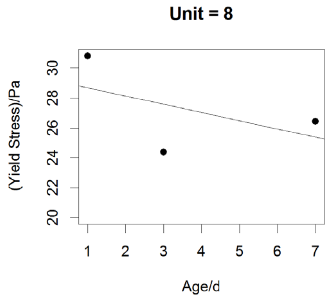
Figure A-2: Yield Stress by unit - Units 5 through 8.
