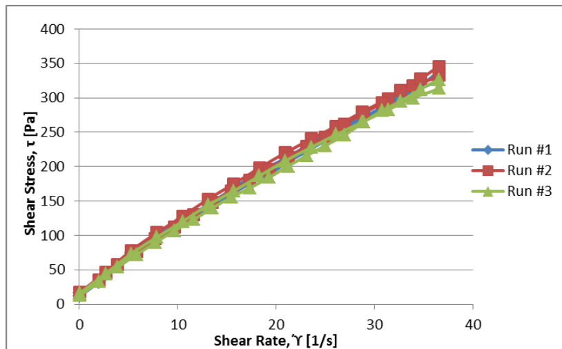
Figure B-21: 7 Day values for Mix G (NIST Code: SR-79)
