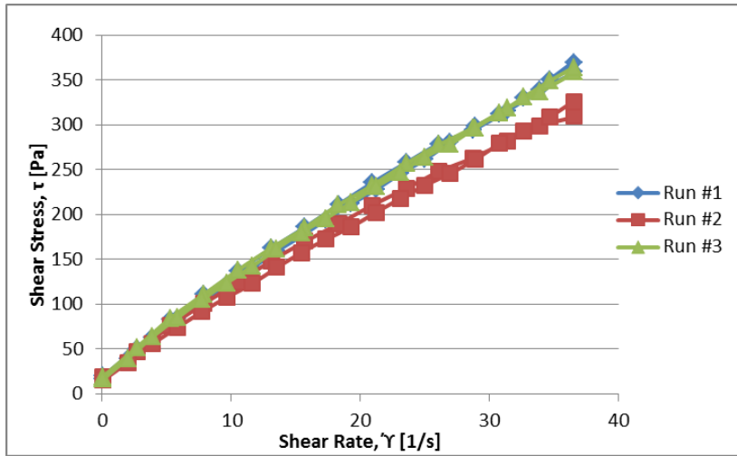
Figure B-19: 1 Day values for Mix G (NIST Code: SR-79)
