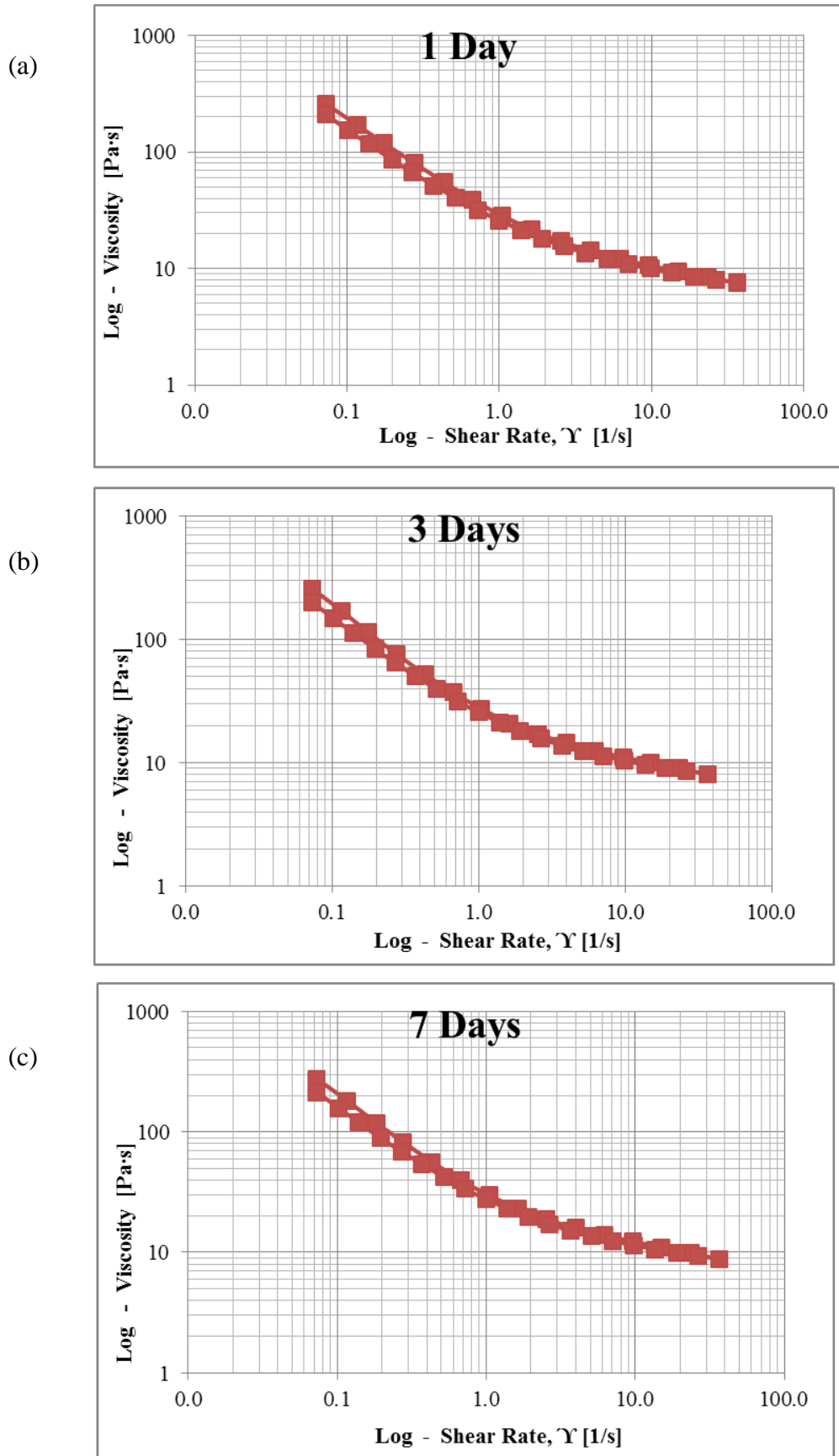
Figure C-2: Viscosity curves for Mix H at (a) 1, (b) 3 and (c) 7 days.
