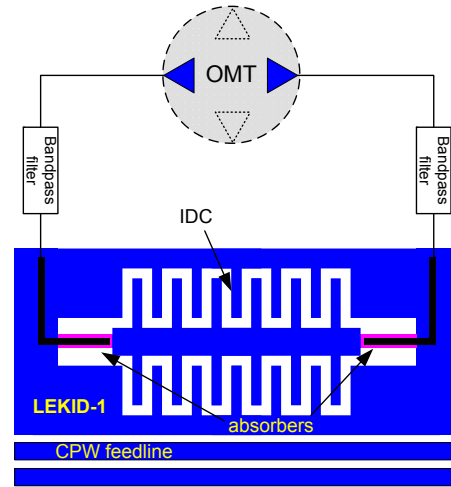
Fig. 3. Concept of an MKID-based dual-polarization pixel coupled via a planar ortho-mode transducer (OMT). Components of the second polarization channel are omitted for simplicity. Radiation is coupled via feedhorn and waveguide directly to the OMT. A Nb ground plane is depicted in blue. Nb microstrip (black) on top of TiN/Ti/TiN (red) forms a lossy transmission line that absorbs the radiation from the OMT. The large IDC capacitively couples the MKID to the coplanar waveguide (CPW) feedline.
