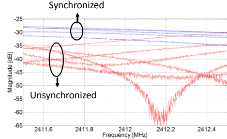
Fig. 5. Instantaneous channel magnitudes of unsynchronized (lower, red) and synchronized (upper, blue) cases. In this measurement setup, the small reverberation chamber was loaded with two absorbers with a horn transmit antenna and a patch receive antenna.
