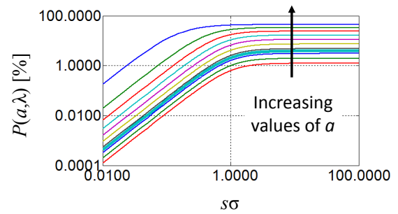
Fig. 2. The probability from (3) that r_2 is a times larger than r_1 plotted for different a values (after [13]).
