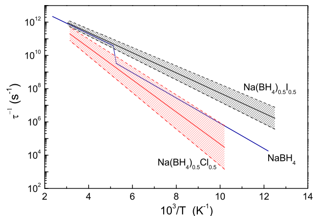
Fig. 2. Temperature dependences of the most probable H jump rates resulting from the fits for \text{Na}(\text{BH}_4)_{0.5}\text{Cl}_{0.5} , \text{Na}(\text{BH}_4)_{0.5}\text{I}_{0.5} , and \text{NaBH}_4 [25]. For the solid solutions, the shaded areas correspond to H jump rates described by the activation energies between \bar{E}_a - \Delta E_a and \bar{E}_a + \Delta E_a . For pure \text{NaBH}_4 , no signs of a distribution of H jump rates have been found [25].
