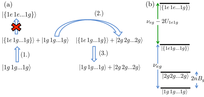
FIG. 4. (a) System prepared in |1g 1g \dots 1g\rangle . Spatially inhomogeneous pulse (1) results in equal superposition of this state and \{|1e 1g \dots 1g\rangle\} , containing one e atom. An interaction blockade prevents coupling to states with two e atoms. Pulse (2) flips the spins of the all- g state. The initial pulse is reversed in pulse (3), resulting in the GHZ state. (b) Relevant energy levels of the Hamiltonian with e and g states and the magnetic field. Note that pulses (1) and (3), which involve states |1g 1g \dots 1g\rangle and \{|1e 1g \dots 1g\rangle\} , do not couple to state \{|1e 1e \dots 1g\rangle\} since there is a blockade of 2U_{1e1g} . Similarly, during pulse (2), blockade prevents excitation of \{|1e 1g \dots 1g\rangle\} .
