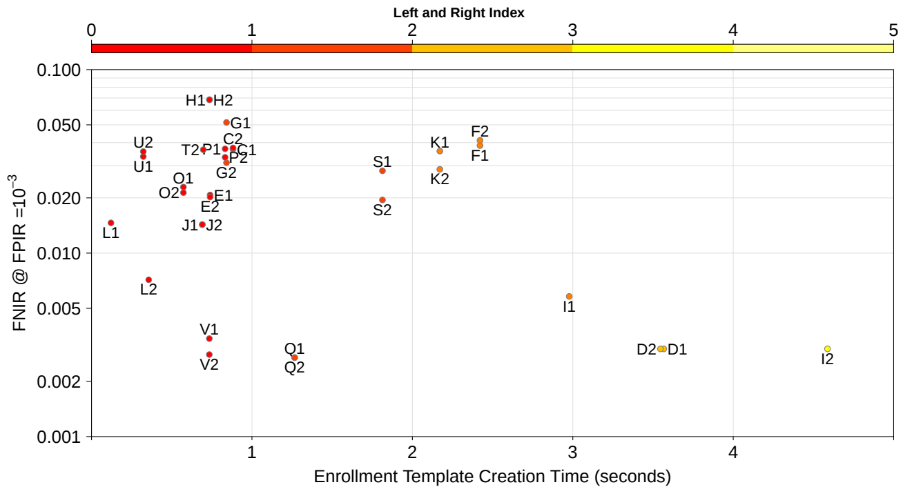
Figure 68: Scatter plot of FNIR @ FPIR = 10 -3 searching 30 000 subjects against 1 600 000 subjects and enrollment template creation time for Class A — Left and Right Index. The color of the data point is used to show the search template creation time. The color scale for search template creation time is at the top of the plot and the units are in seconds. The template creation time data is from Table 74 in Appendix H.
