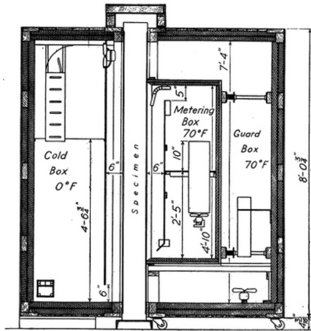
Figure 6 Cross-section of NBS hot box test apparatus 1937 – 1964 (Whittemore et al., 1943)
