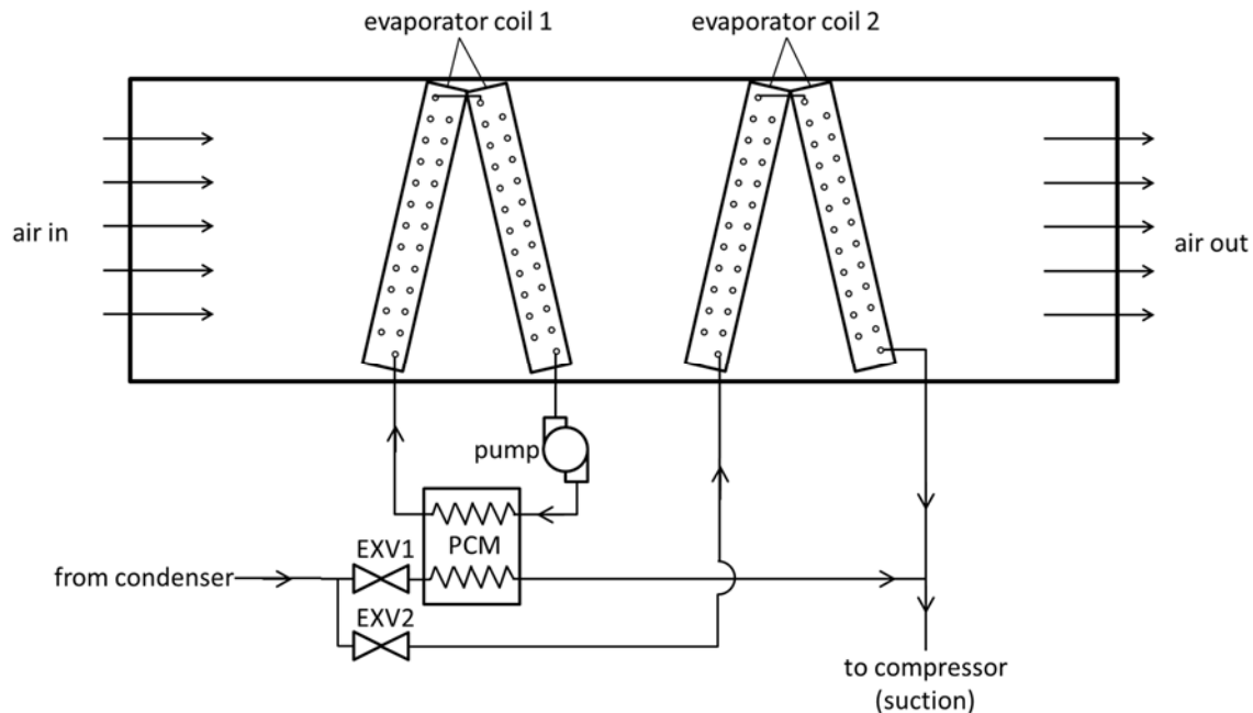
Figure 11 External PCM evaporator where the PCM is pumped through the first evaporator coil
