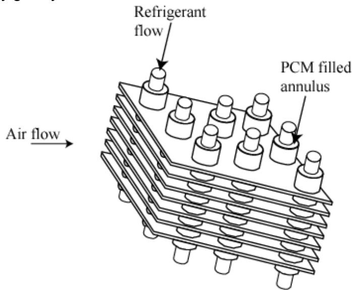
Figure 8 Proposed PCM evaporator for investigation
