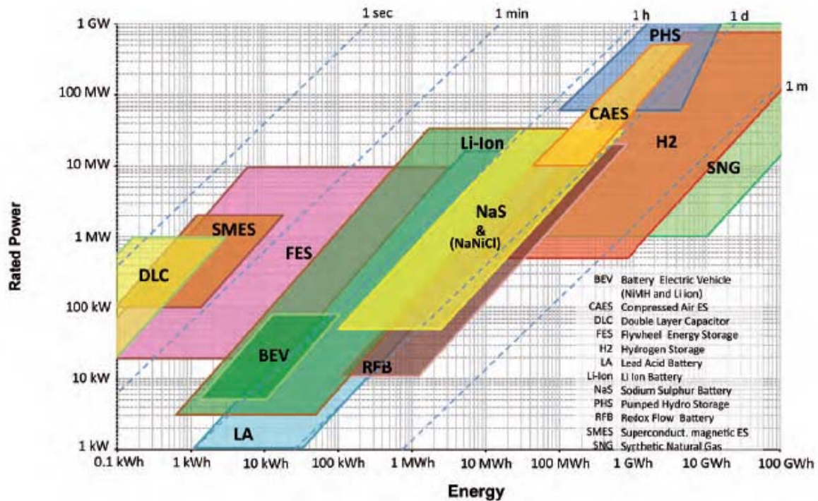
Figure 2 Fraunhofer ISE comparison of rated power, energy content and discharge time of different EES technologies (IEC, 2011)
