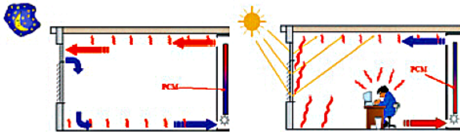
Figure 4 Passive cooling with external PCM wall (IRENA, 2013)
