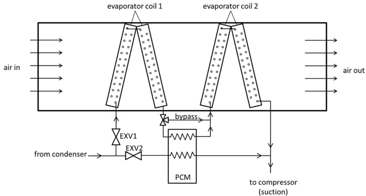
Figure 10 External PCM evaporator where PCM re-condenses refrigerant before the refrigerant enters the second evaporator coil
