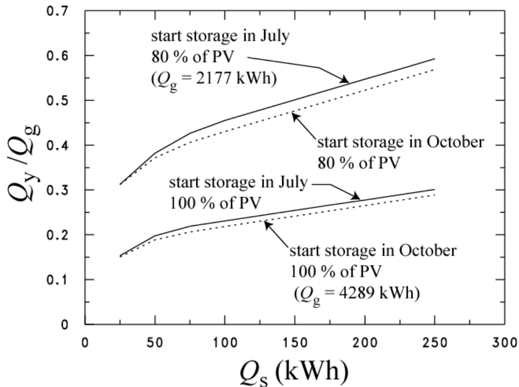
Figure 14 Fraction of excess electricity stored as a function of the size of the storage system
