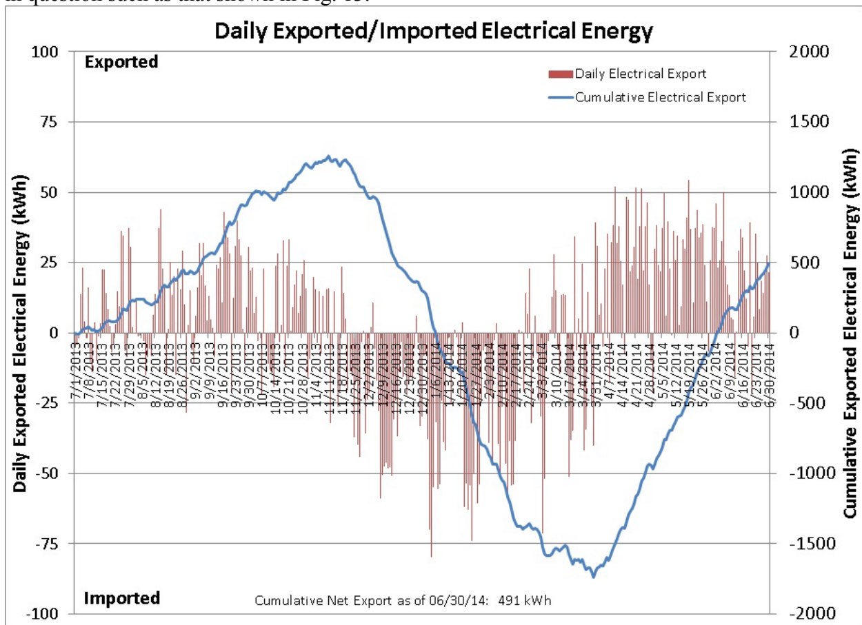
Figure 13 Net zero house electricity net generation and usage (Fanney et al., 2014)
