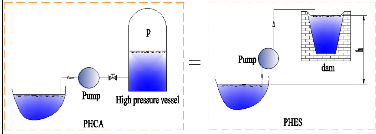
Figure 3 Comparison of PHCA to equivalent PHES system (Wang et al., 2013)
