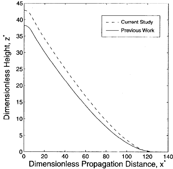
Figure 10. Dimensionless height as a function of dimensionless propagation distance for U_w = 3 . The dashed line indicates current study ( C_d = 0.45 , D_o^* = 3.9 , \Phi = 200 ); the solid line illustrates previous work 6,13 ( C_d(\text{Re}) , d_o^* = 10000 , \rho^* = 1/7600 , B = 1.2 , \text{Pr} = 0.7 ).
