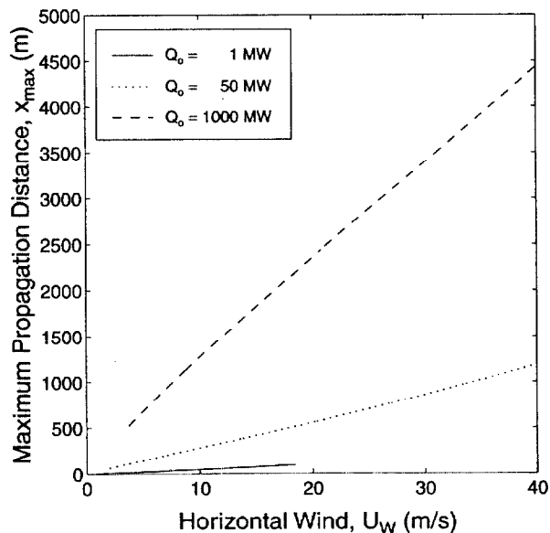
Figure 13. Maximum propagation distance as a function of horizontal wind for as noted. Due to range of dimensionless horizontal wind studied, 0.3 < U_w^* < 6 , minimum velocity increases with Q_o ( U_w = fn(Q_o) )
