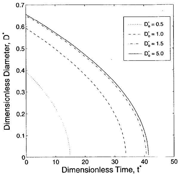
Figure 2. Dimensionless diameter as a function of dimensionless time; \Phi = 200 and D_o^* as noted.
