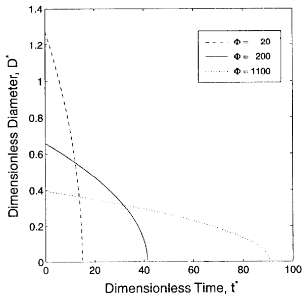
Figure 3. Dimensionless diameter as a function of dimensionless time; D_o^* = 5 and \Phi as noted.
