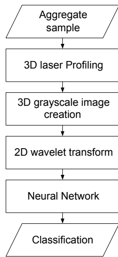
Figure 2. Artificial intelligence based aggregate classification system.
