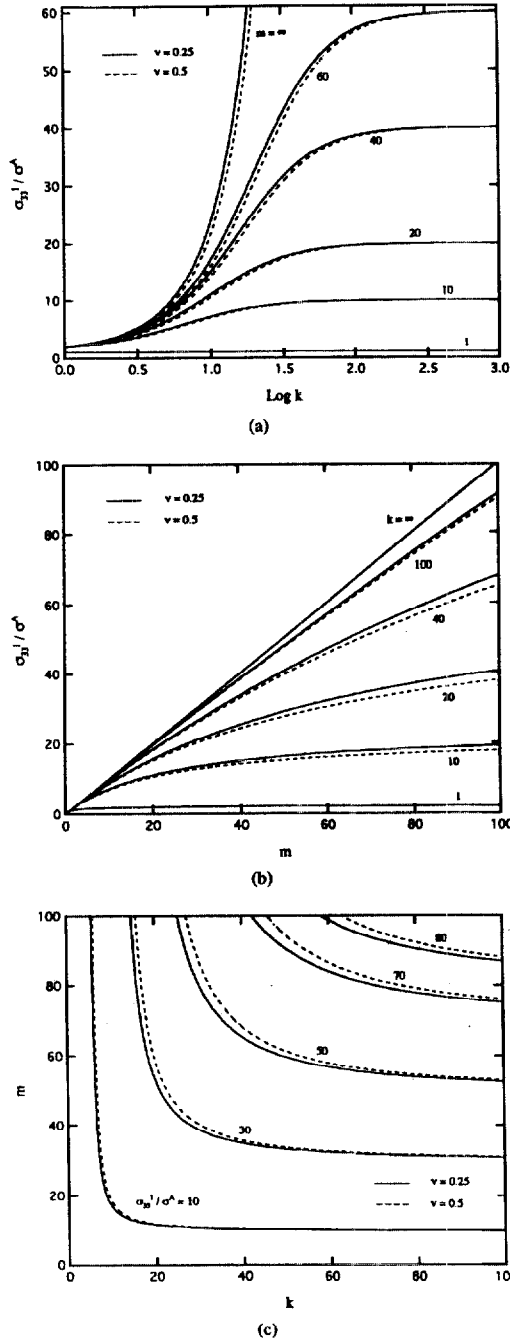
Figure 1 (a) \sigma_{33}^I/\sigma^A as a function of k ; (b) \sigma_{33}^I/\sigma^A as a function of m ; and (c) m as a function of k . Solid and dashed lines represent \nu = \nu^* = 0.25 and 0.5 , respectively.
