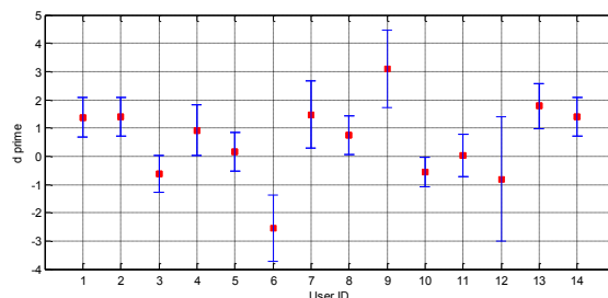
Figure 3: d' calculation for Phase 1. The red squares indicate the average value for d' , and the blue lines indicate the standard deviation of the values.
