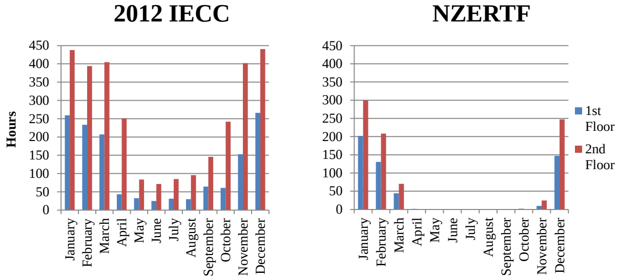
Figure 2-4 Simple ASHRAE 55-2010 Not Comfortable for 2012 IECC and NZERTF Designs - Hours
