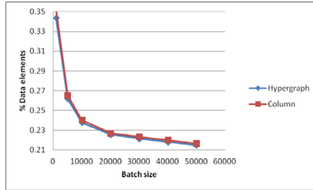
Figure 7. Data Element Reduction as Batch Size Increases
