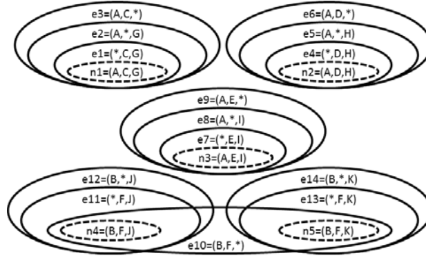
Figure 1. Hypergraph for Alert Aggregation Example
