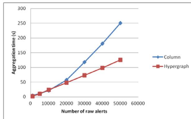
Figure 9. Aggregation of Snort Alerts at Hamming distance 2
