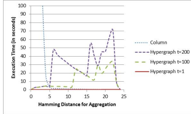
Figure 10. Mean Execution Time to Aggregate EVTX Alerts
