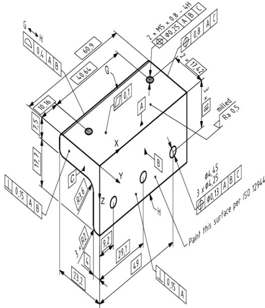
Fig. 1. An example of standardized presentation of product manufacturing information (PMI) on a 3D model [4].
