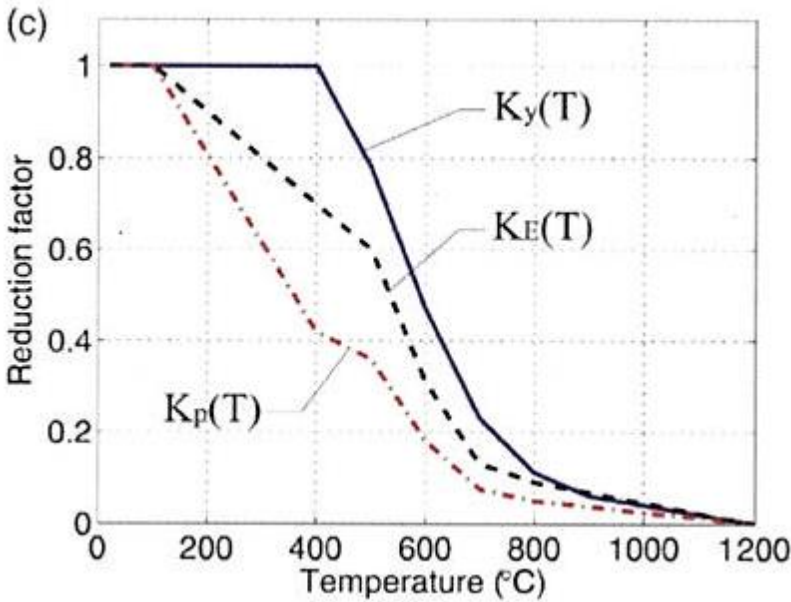
Figure 4.1 Reduction factors for the stress-strain relationship of carbon steel at elevated temperatures (EN 1993-1-2:2010, also Phan et al. 2010 NIST TN 1681)
