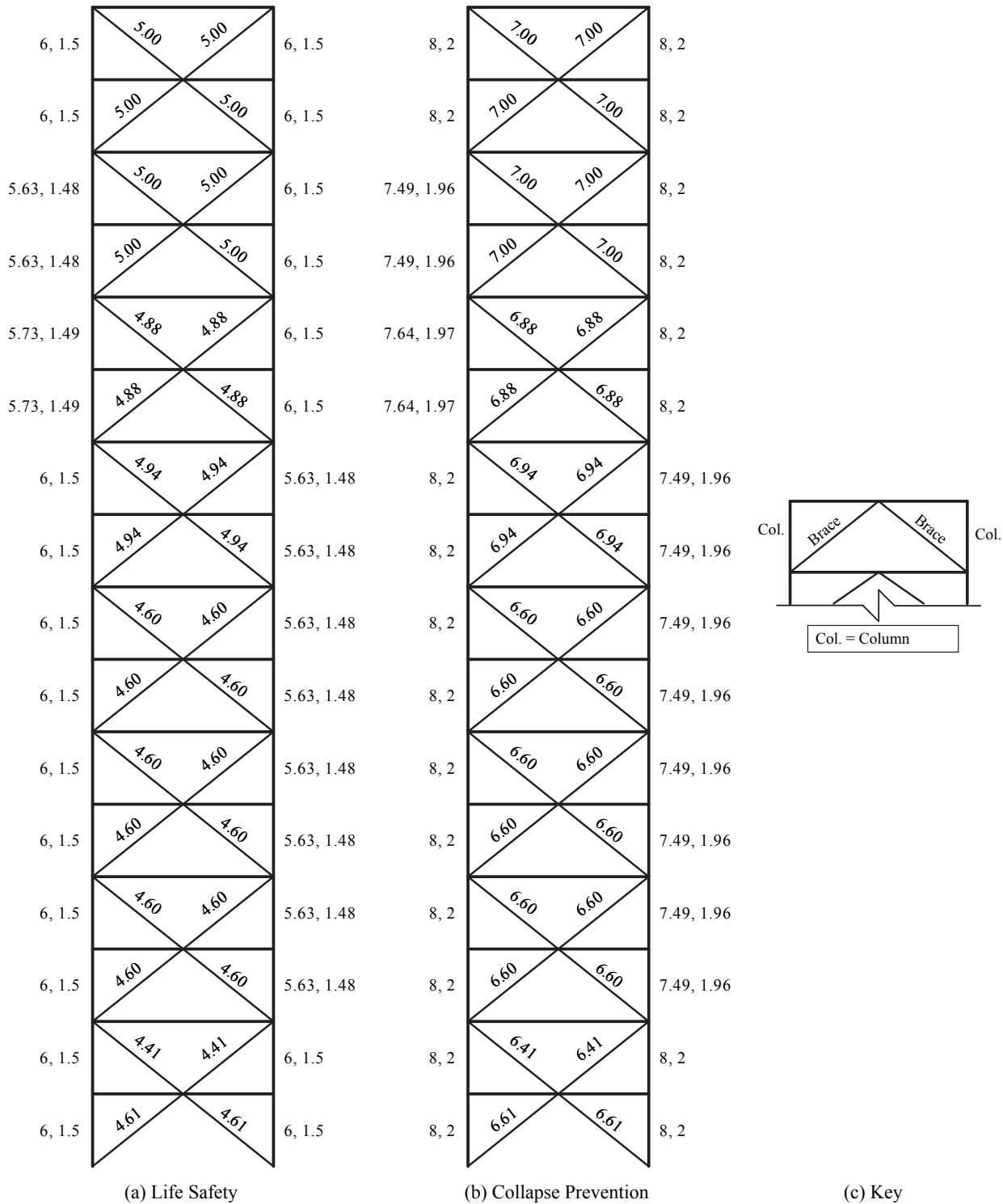
Figure 3-11. Frame Capacity Schematic ( m -factor), LS and CP, 16-Story SCBF ELF
