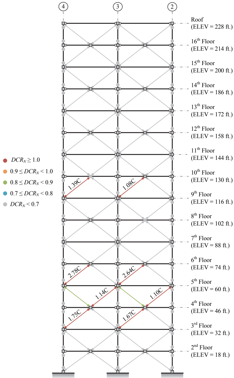
Figure 3-101. NSP Assessment Results, 16-Story SCBF ELF, BSE-2 CP (+push to left)
