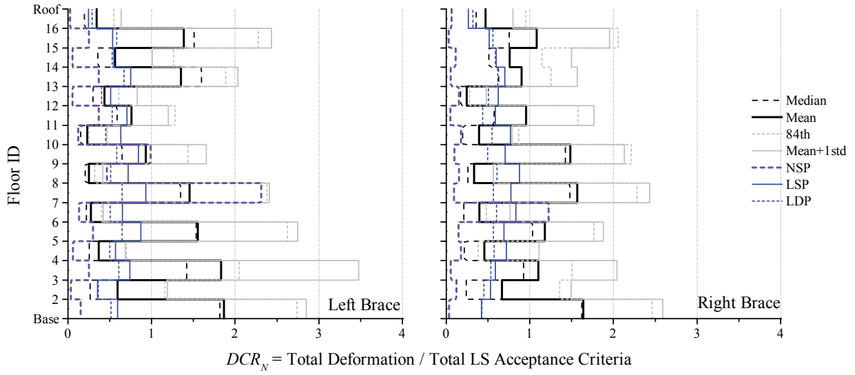
Figure 3-104. NDP Assessment Results, Brace Struts, 16-Story SCBF RSA, BSE-1 LS
