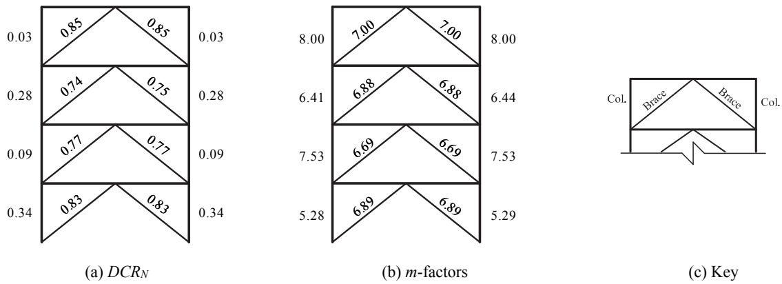
Figure 3-34. LDP Assessment Results, 4-Story SCBF RSA, BSE-2 CP
