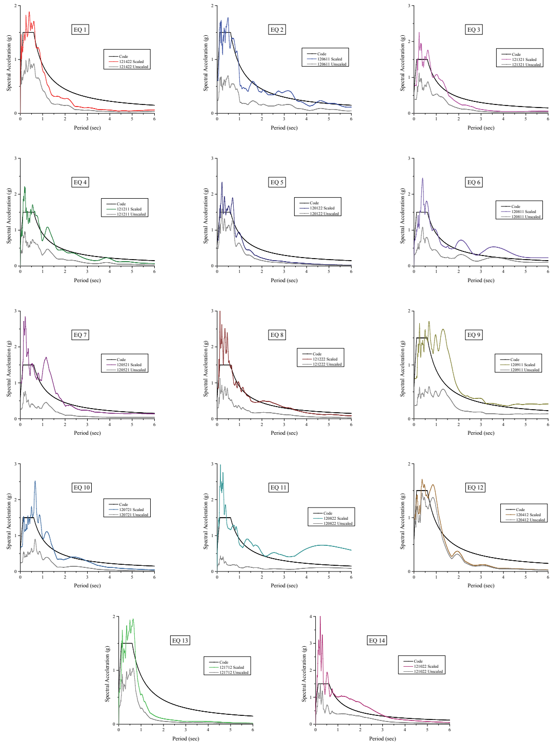
Figure A-2. Acceleration Response Spectra: Original and Scaled for Each Selected Record for N-S Direction of MC4
