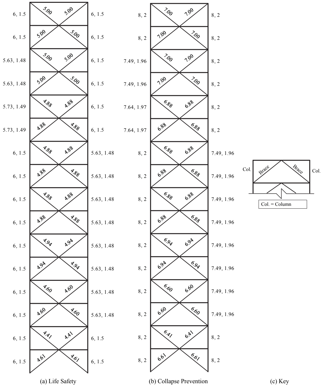
Figure 3-12. Frame Capacity Schematic ( m -factor), LS and CP, 16-Story SCBF RSA
