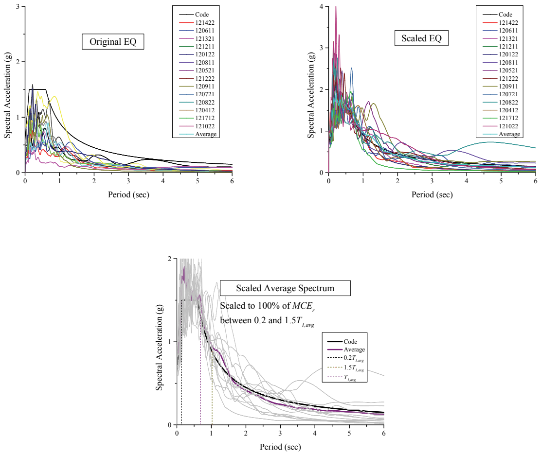
Figure A-1. Acceleration Response Spectra: Original, Scaled, and Scaled Average Spectrum for N-S Direction of MC4
