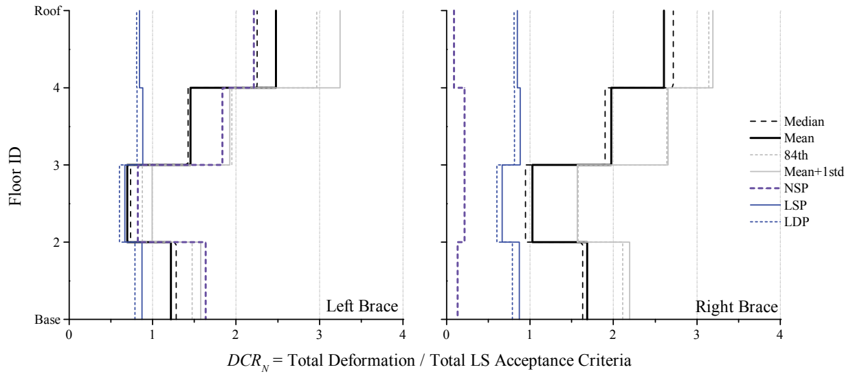
Figure 3-47. NDP Assessment Results, Brace Struts, 4-Story SCBF ELF, BSE-2 CP
