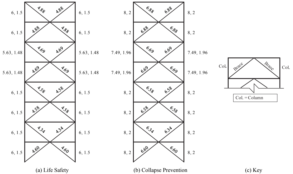
Figure 3-10. Frame Capacity Schematic ( m -factor), LS and CP, 8-Story SCBF RSA
