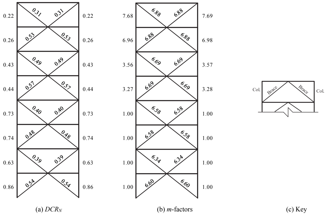
Figure 3-63. LDP Assessment Results, 8-Story SCBF RSA, BSE-2 CP
