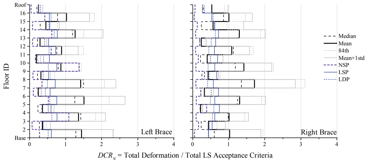
Figure 3-103. NDP Assessment Results, Brace Struts, 16-Story SCBF ELF, BSE-1 LS
