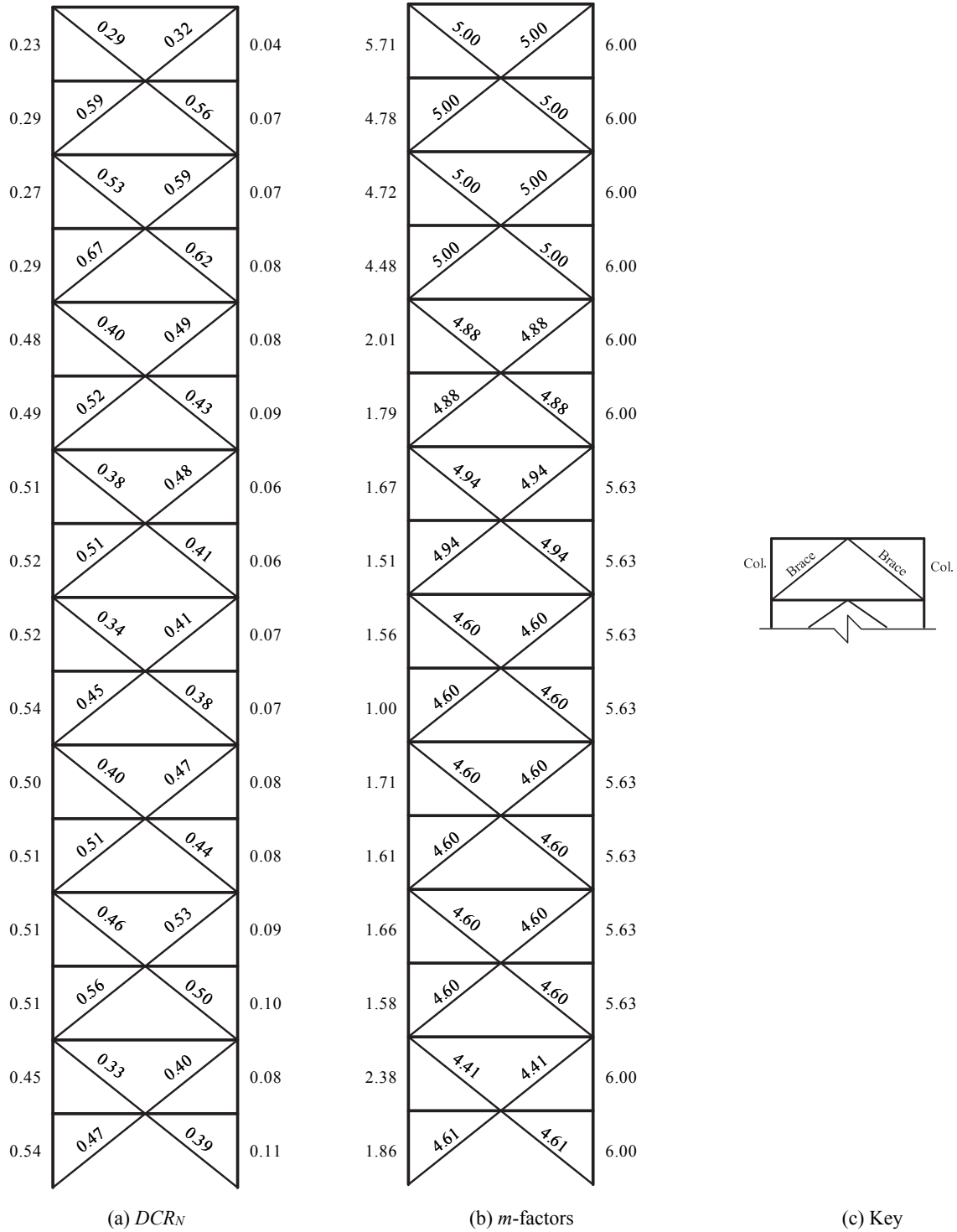
Figure 3-88. LDP Assessment Results, 16-Story SCBF ELF, BSE-1 LS
