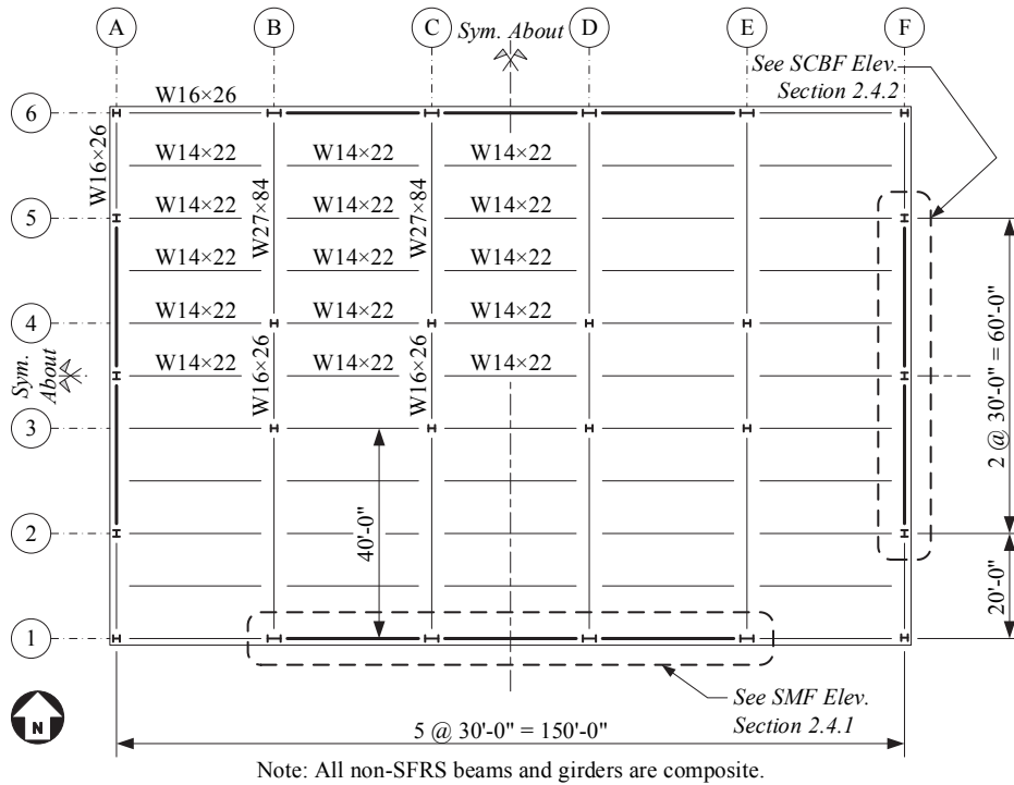
Figure 2-5. Typical Floor Framing Plan, MC16
