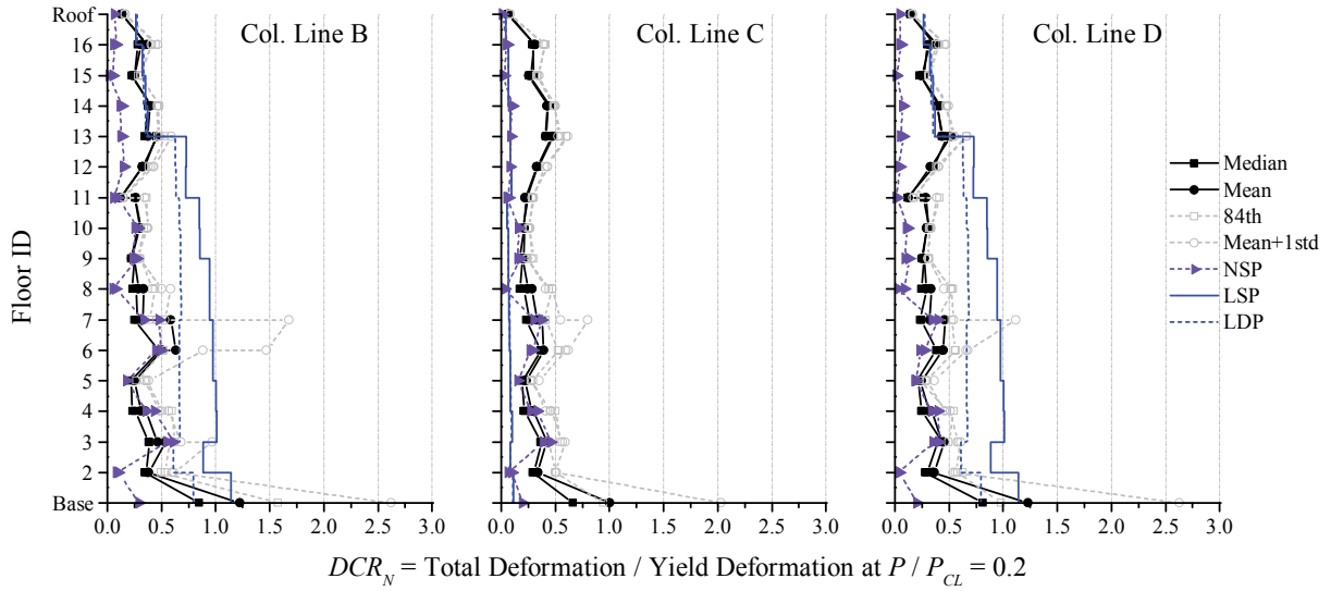
Figure 3-107. NDP Assessment Results, Column Hinges, 16-Story SCBF ELF, BSE-2 Yield
