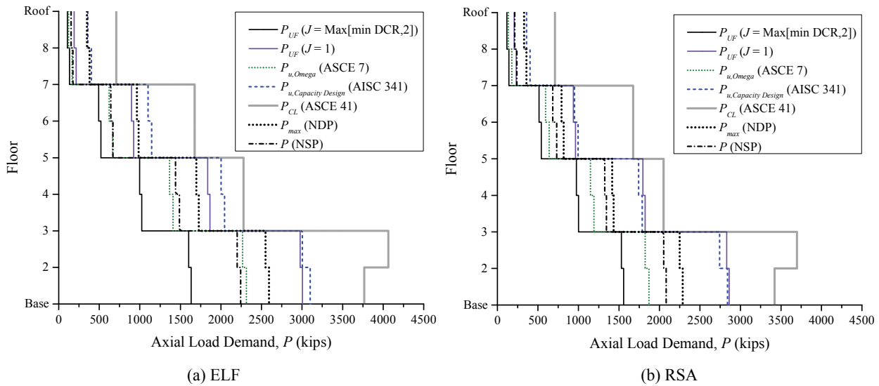
Figure 3-61. LDP Assessment Results, Compression in Ext. Columns, 8-Story SCBF, BSE-1
