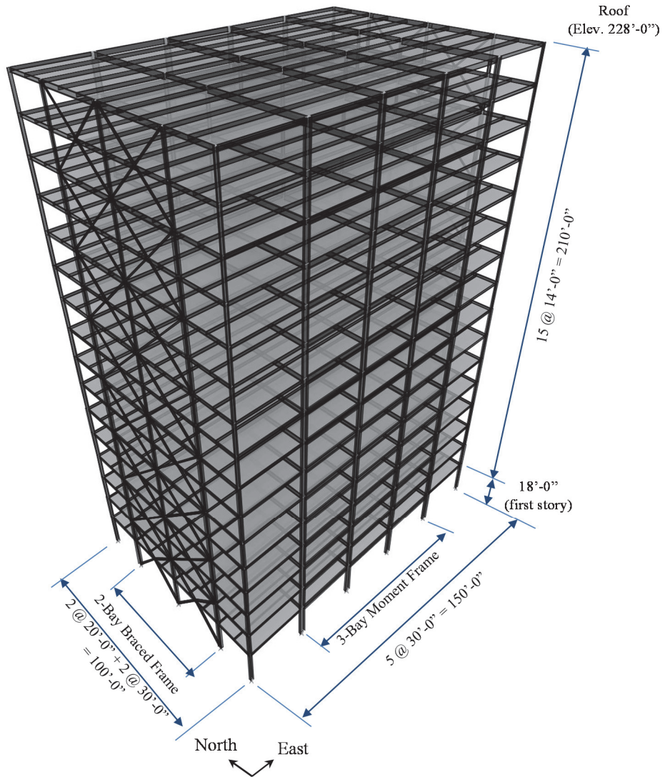
Figure 2-3. Isometric View of MC16 Archetype Building
