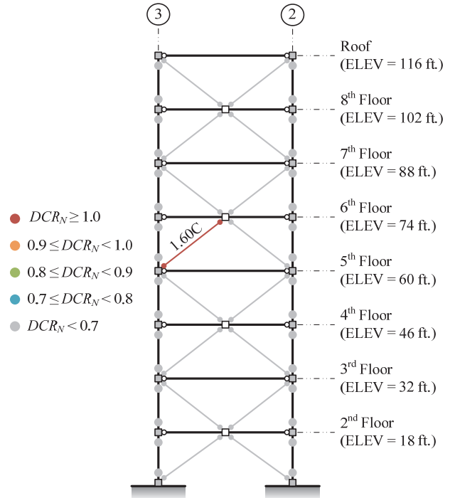
Figure 3-71. NSP Assessment Results, 8-Story SCBF RSA, BSE-1 LS (+push to left)
