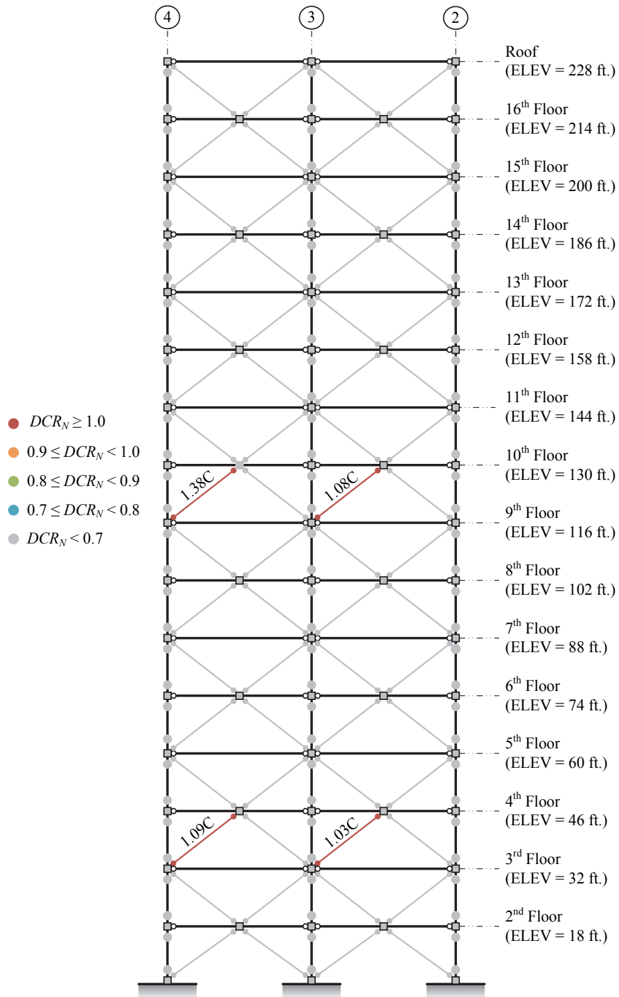
Figure 3-99. NSP Assessment Results, 16-Story SCBF ELF, BSE-1 LS (+push to left)
