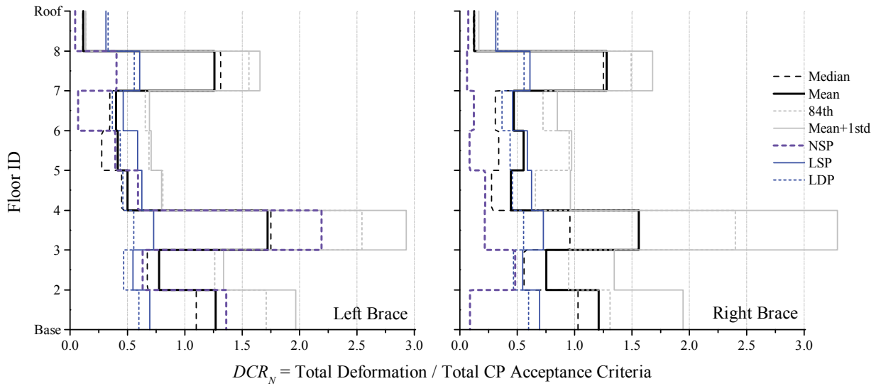
Figure 3-76. NDP Assessment Results, Brace Struts, 8-Story SCBF ELF, BSE-2 CP
