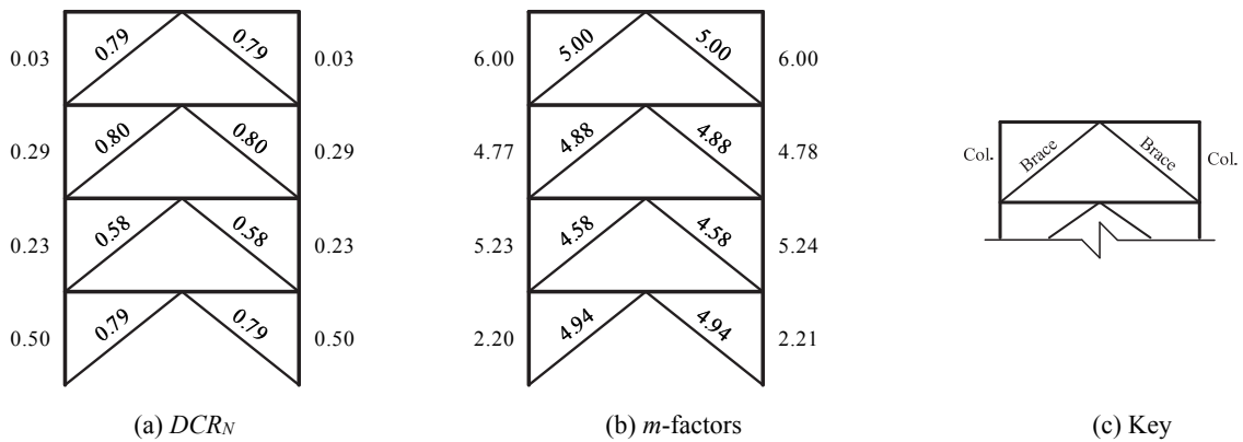
Figure 3-24. LSP Assessment Results, 4-Story SCBF ELF, BSE-1 LS
