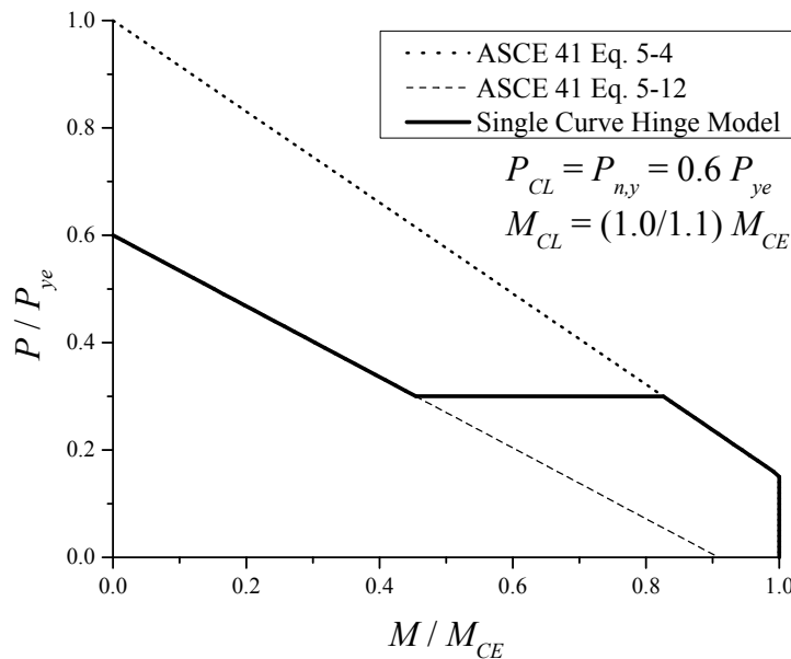
Figure 3-15. In-plane Flexural Hinge Yield Surface Model (Including Force-Controlled Response)
