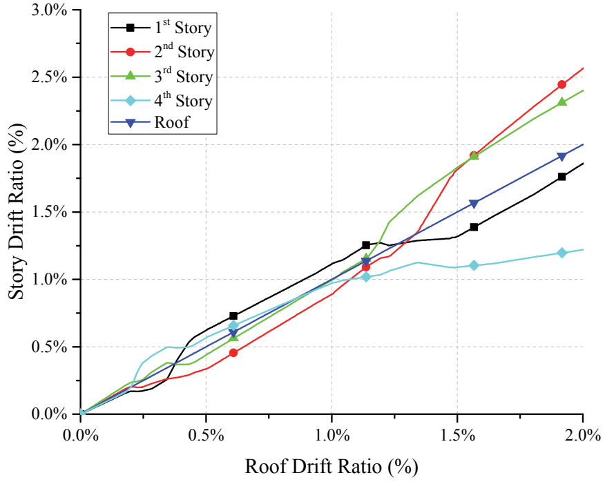
Figure 3-38. 4-Story SCBF ELF Pushover – Story Drift Ratios – BSE-2
