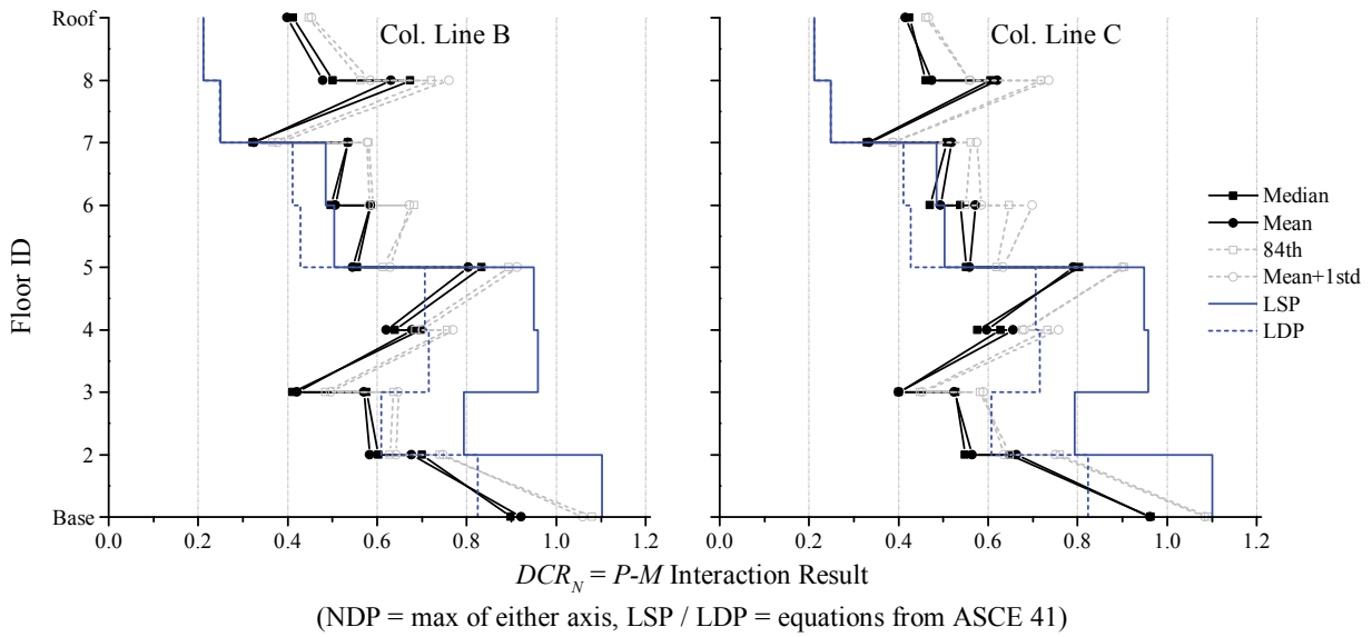
Figure 3-81. NDP Assessment Results, Column Members, 8-Story SCBF RSA, BSE-2
