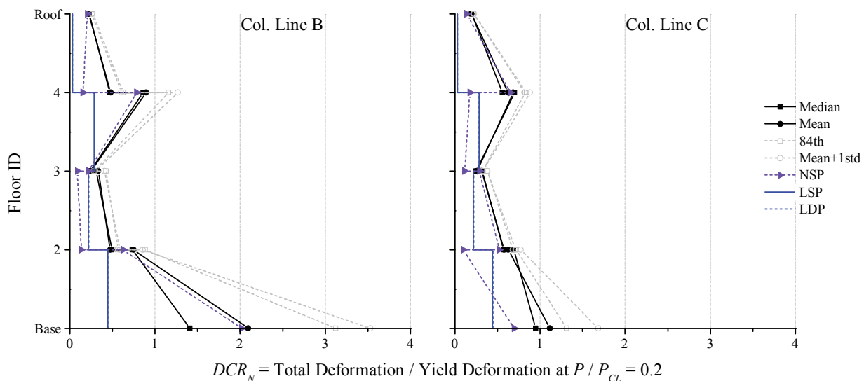
Figure 3-49. NDP Assessment Results, Column Hinges, 4-Story SCBF ELF, BSE-2 Yield
