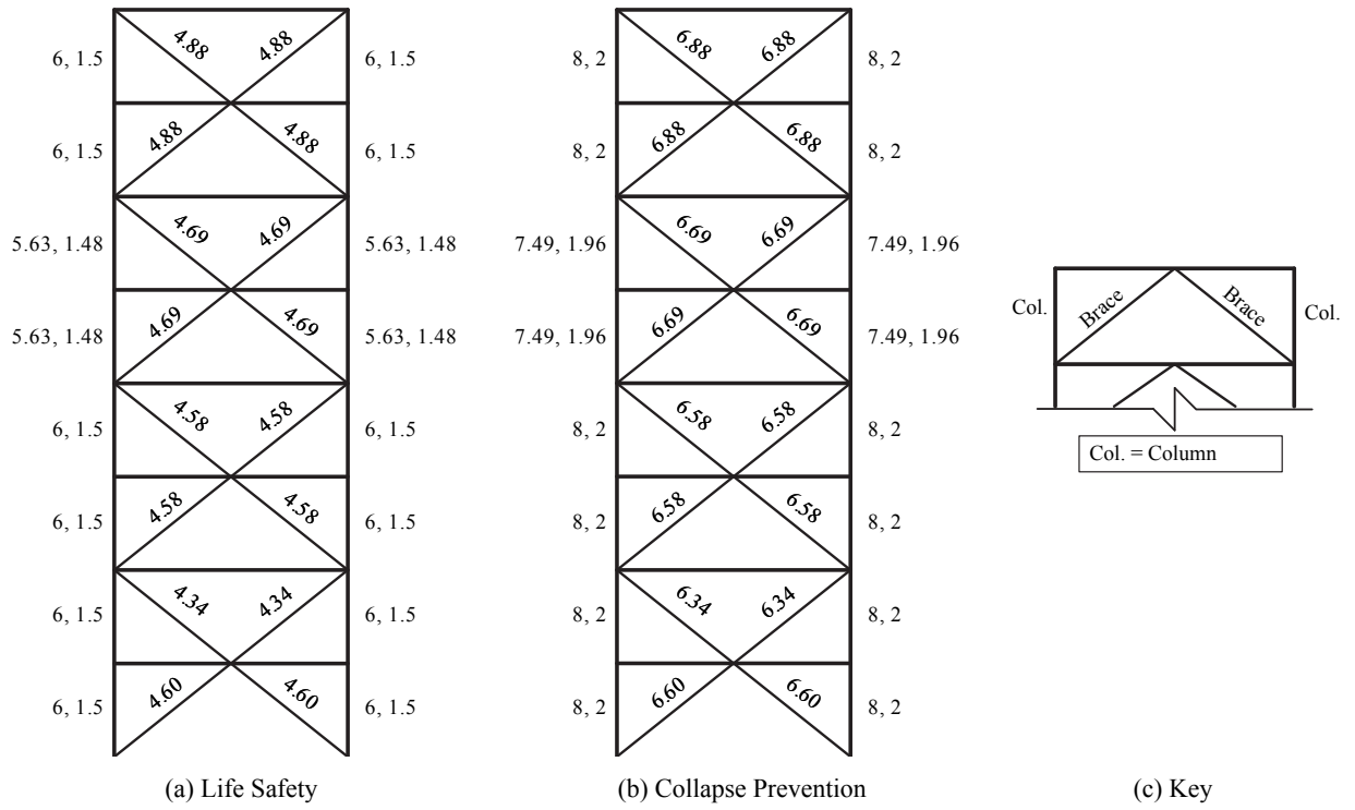
Figure 3-9. Frame Capacity Schematic ( m -factor), LS and CP, 8-Story SCBF ELF
