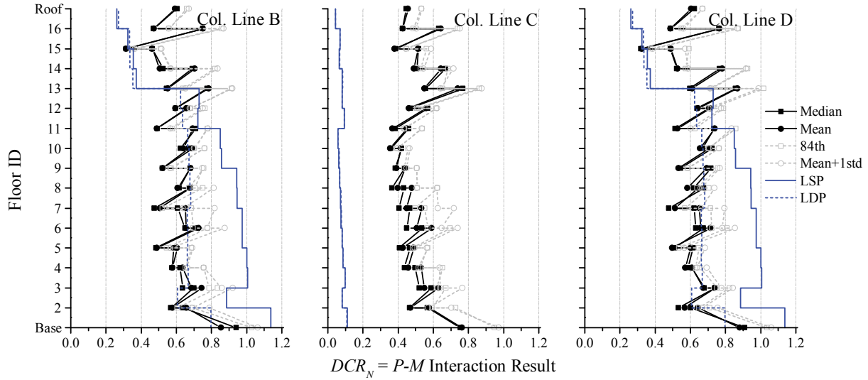
Figure 3-109. NDP Assessment Results, Column Members, 16-Story SCBF ELF, BSE-2
