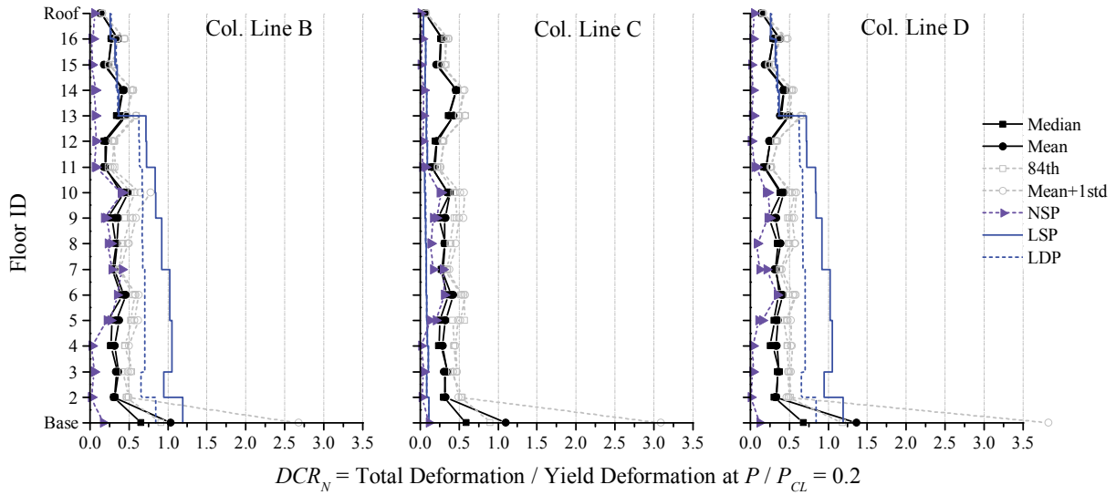
Figure 3-108. NDP Assessment Results, Column Hinges, 16-Story SCBF RSA, BSE-2 Yield
