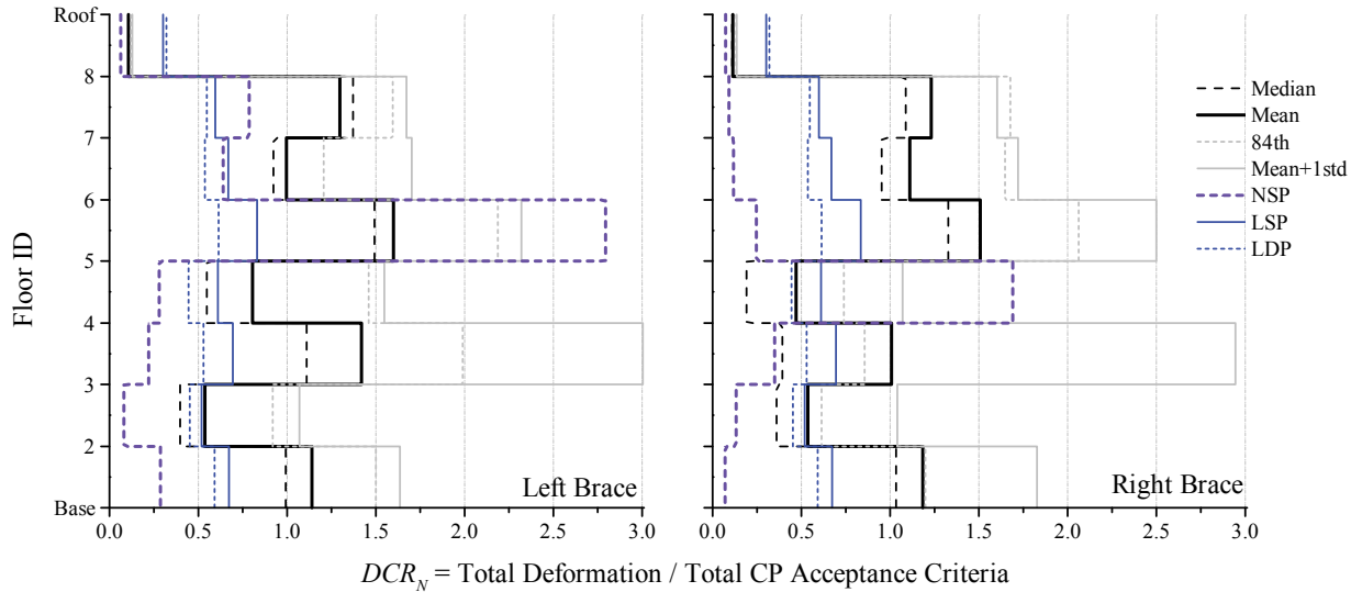
Figure 3-77. NDP Assessment Results, Brace Struts, 8-Story SCBF RSA, BSE-2 CP
