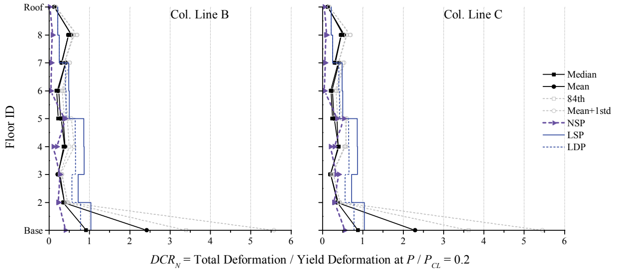
Figure 3-78. NDP Assessment Results, Column Hinges, 8-Story SCBF ELF, BSE-2 Yield
