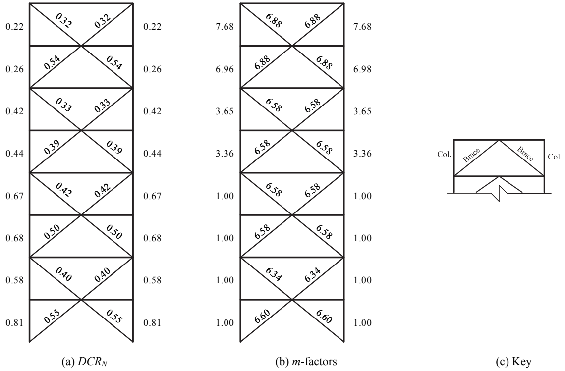
Figure 3-62. LDP Assessment Results, 8-Story SCBF ELF, BSE-2 CP
