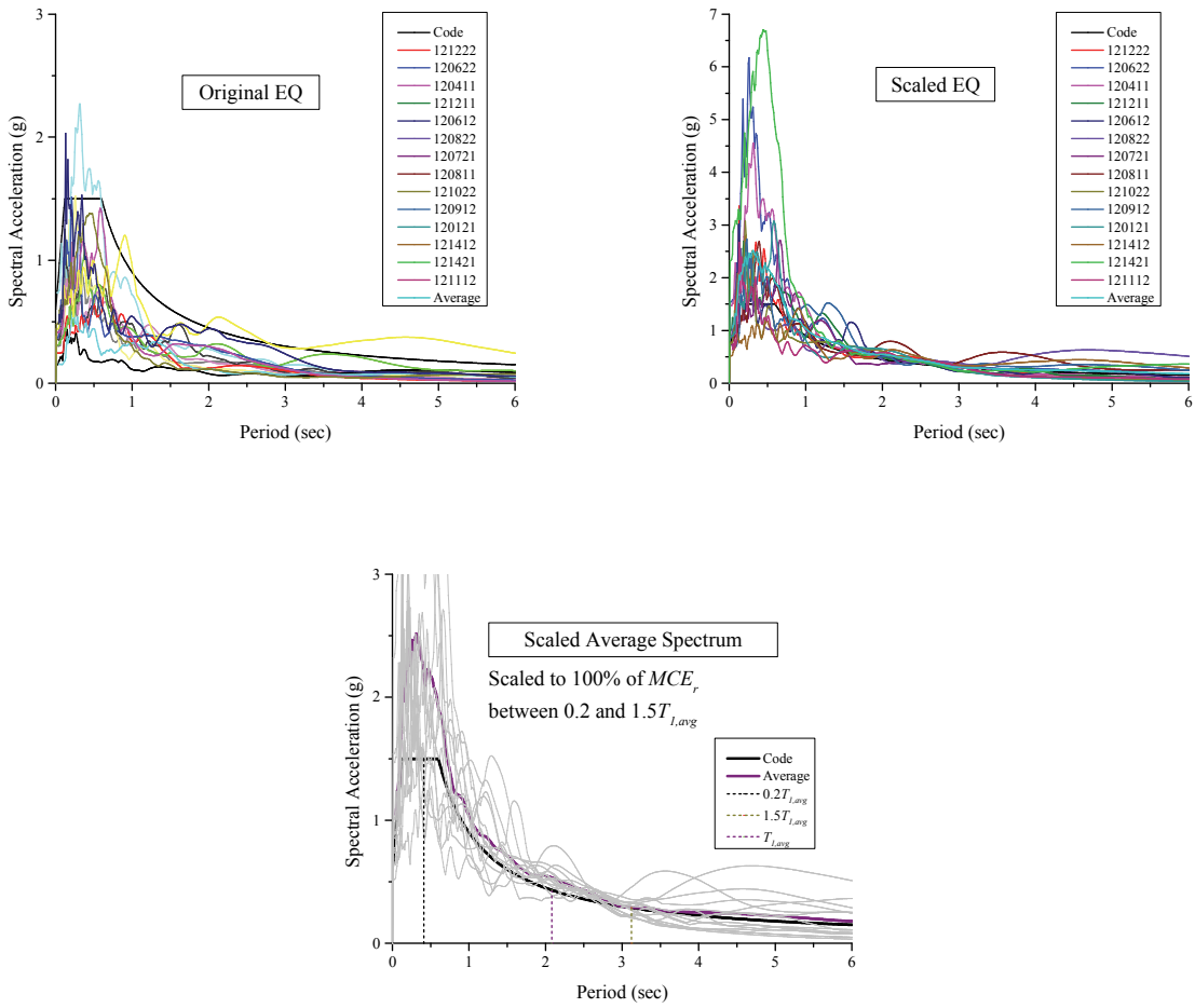
Figure A-5. Acceleration Response Spectra: Original, Scaled, and Scaled Average Spectrum for N-S Direction of MC16
