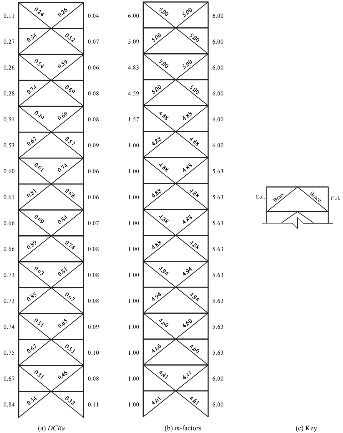
Figure 3-83. LSP Assessment Results, 16-Story SCBF RSA, BSE-1 LS
