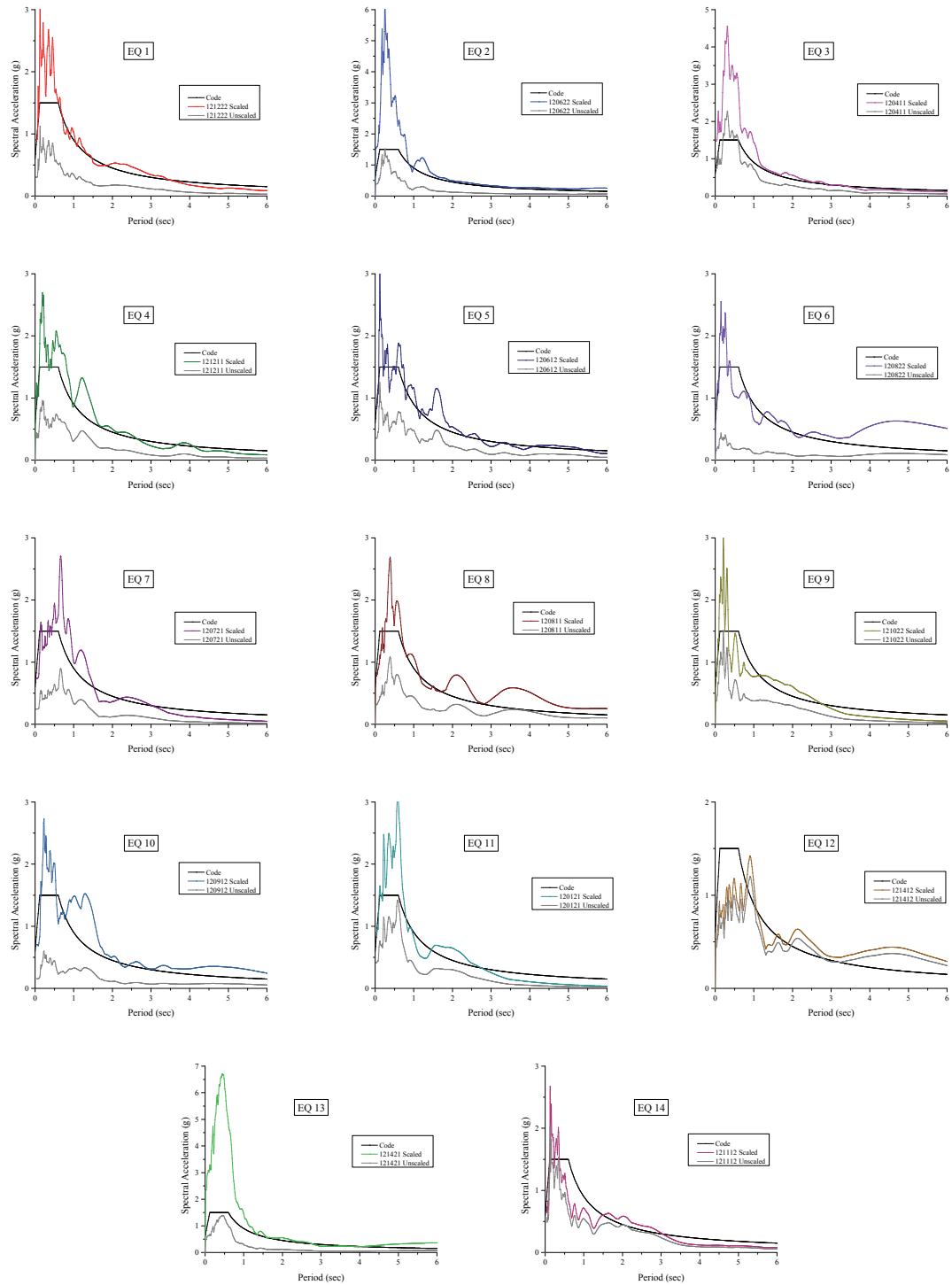
Figure A-6. Acceleration Response Spectra: Original and Scaled for Each Selected Record for N-S Direction of MC16
