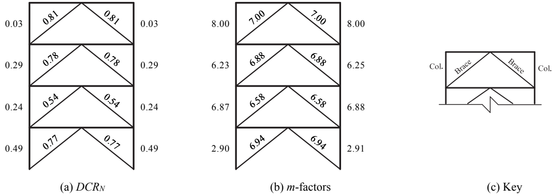
Figure 3-33. LDP Assessment Results, 4-Story SCBF ELF, BSE-2 CP
