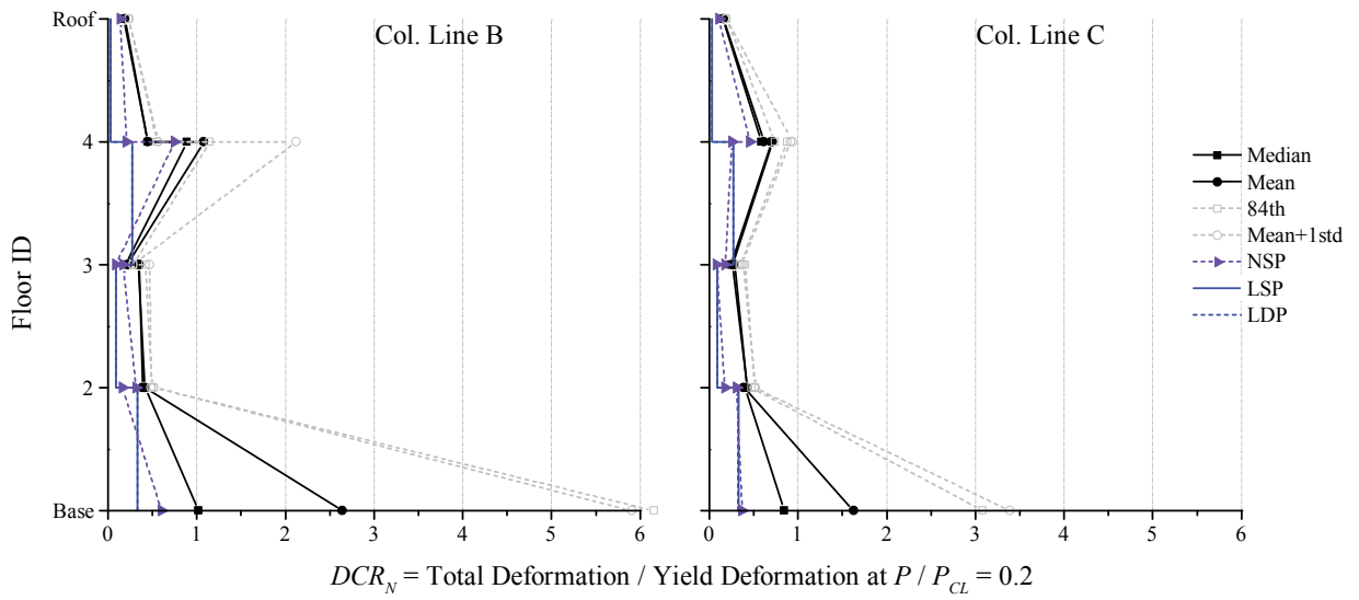
Figure 3-50. NDP Assessment Results, Column Hinges, 4-Story SCBF RSA, BSE-2 Yield
