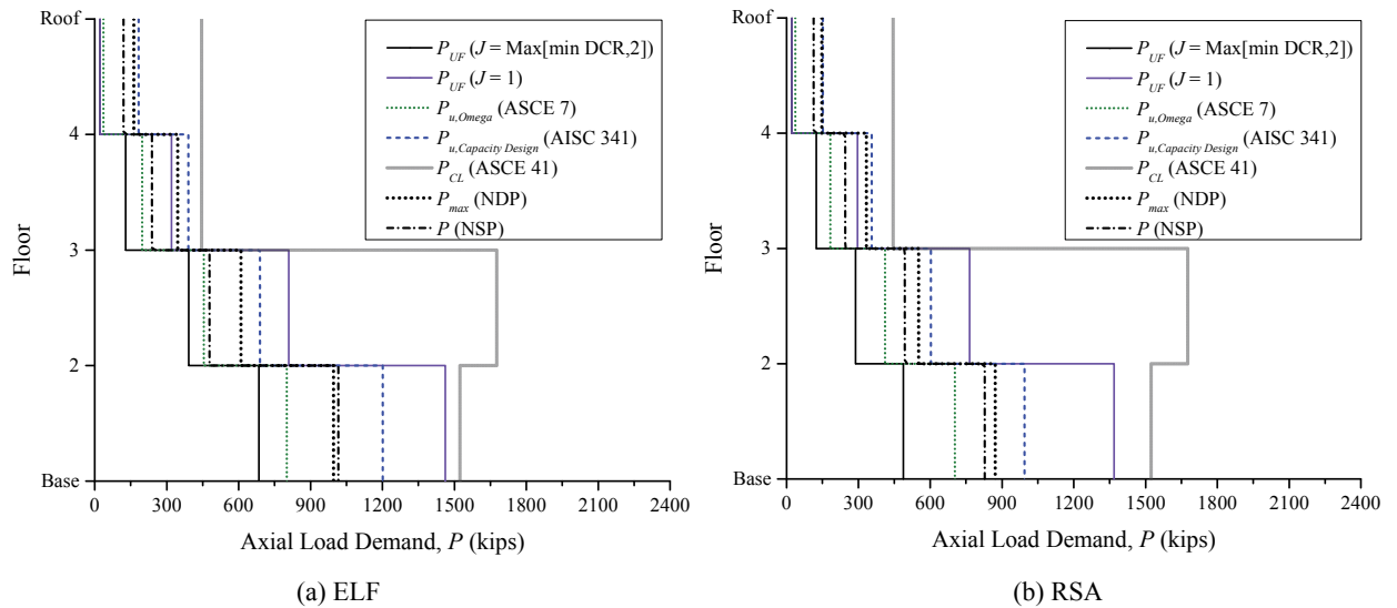
Figure 3-32. LDP Assessment Results, Compression in Ext. Columns, 4-Story SCBF, BSE-1
