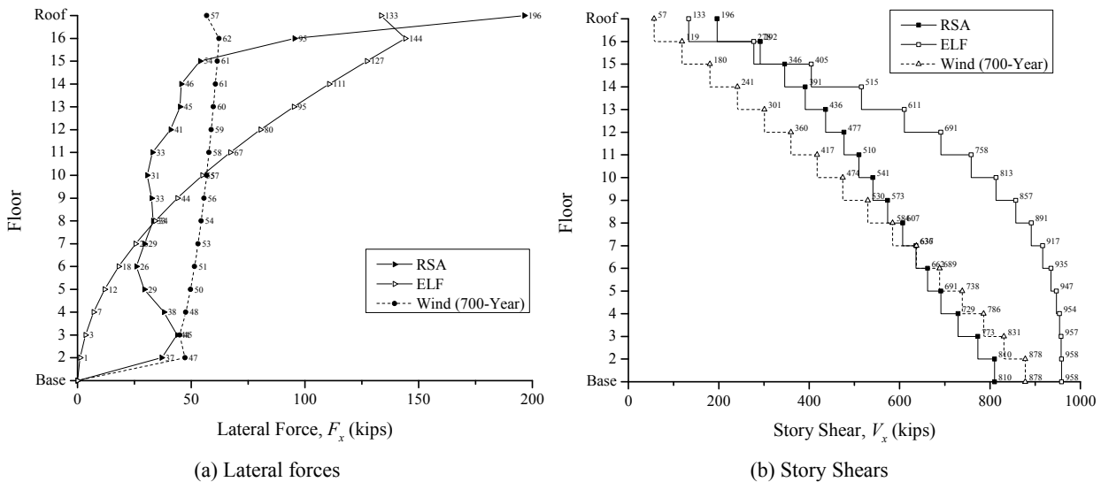
Figure B-7. Strength Design Lateral Forces and Story Shears
