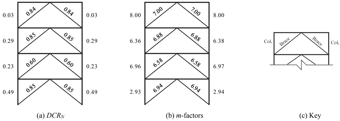
Figure 3-27. LSP Assessment Results, 4-Story SCBF ELF, BSE-2 CP
