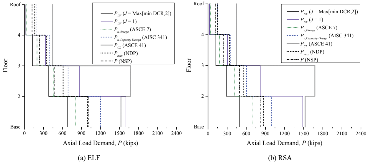
Figure 3-26. LSP Assessment Results, Compression in Ext. Columns, 4-Story SCBF, BSE-1
