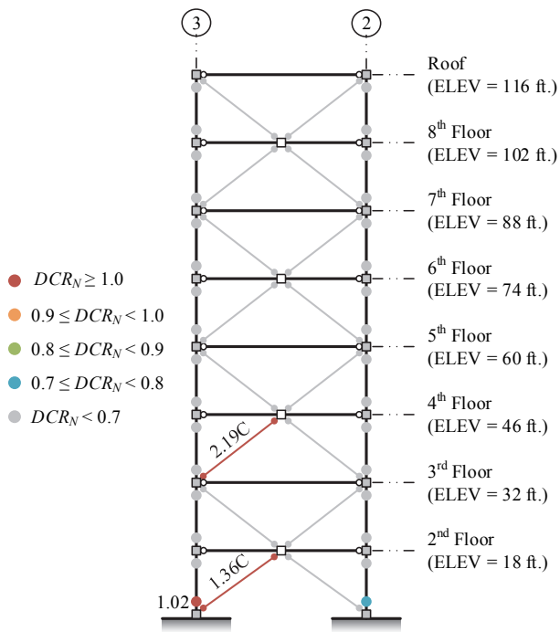
Figure 3-72. NSP Assessment Results, 8-Story SCBF ELF, BSE-2 CP (+push to left)
