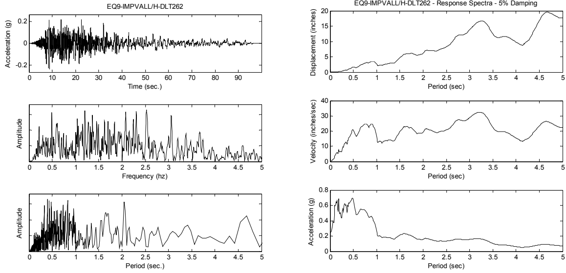
Figure A-15. 1979 Imperial Valley Earthquake at Delta Station, Comp. 262
