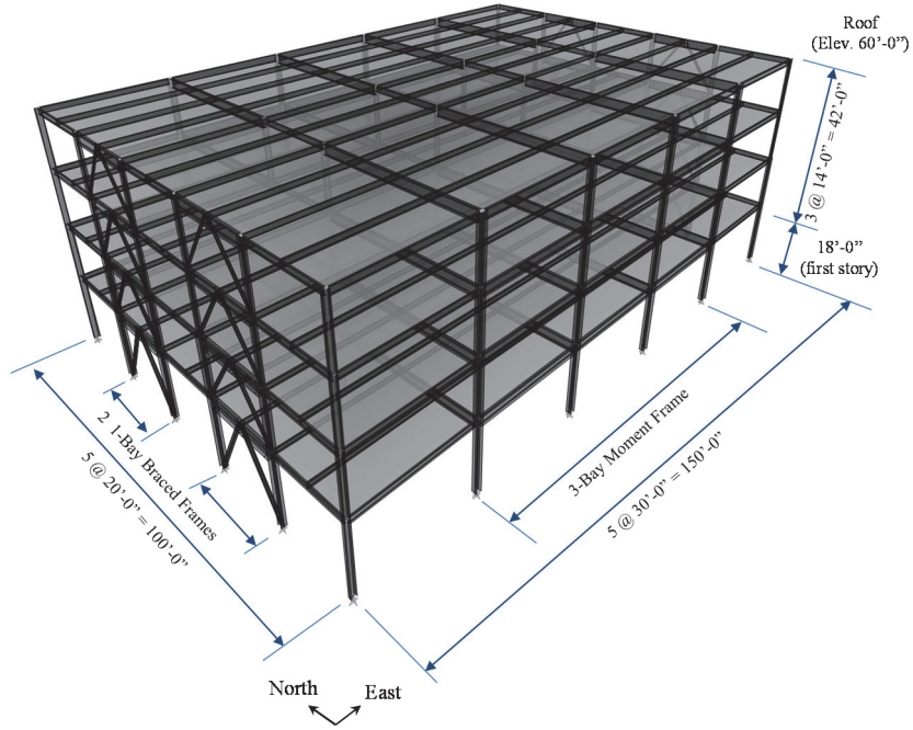
Figure 2-1. Isometric View of MC4 Archetype Building
