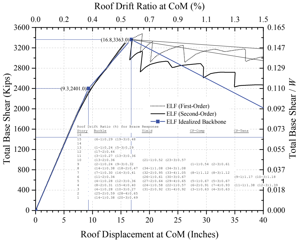
Figure 3-94. 16-Story SCBF ELF Pushover, BSE-2
