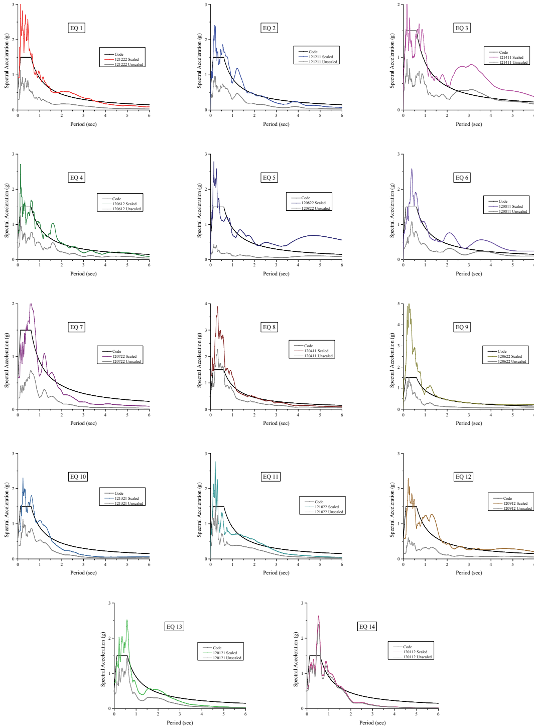
Figure A-4. Acceleration Response Spectra: Original and Scaled for Each Selected Record for N-S Direction of MC8
