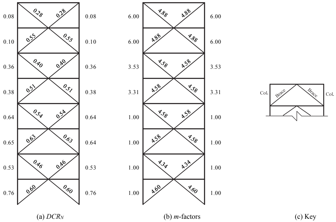
Figure 3-53. LSP Assessment Results – 8-Story SCBF ELF – BSE-1 – LS
