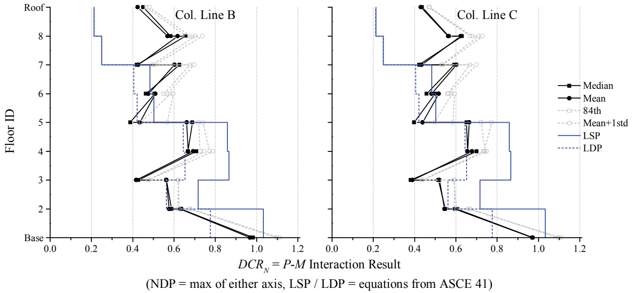
Figure 3-80. NDP Assessment Results, Column Members, 8-Story SCBF ELF, BSE-2
