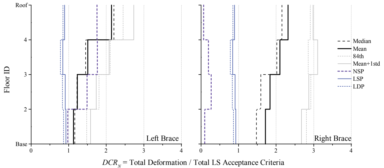
Figure 3-48. NDP Assessment Results, Brace Struts, 4-Story SCBF RSA, BSE-2 CP
