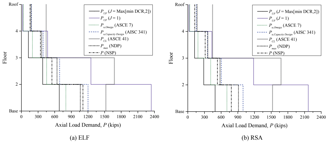
Figure 3-29. LSP Assessment Results, Compression in Ext. Columns, 4-Story SCBF, BSE-2
