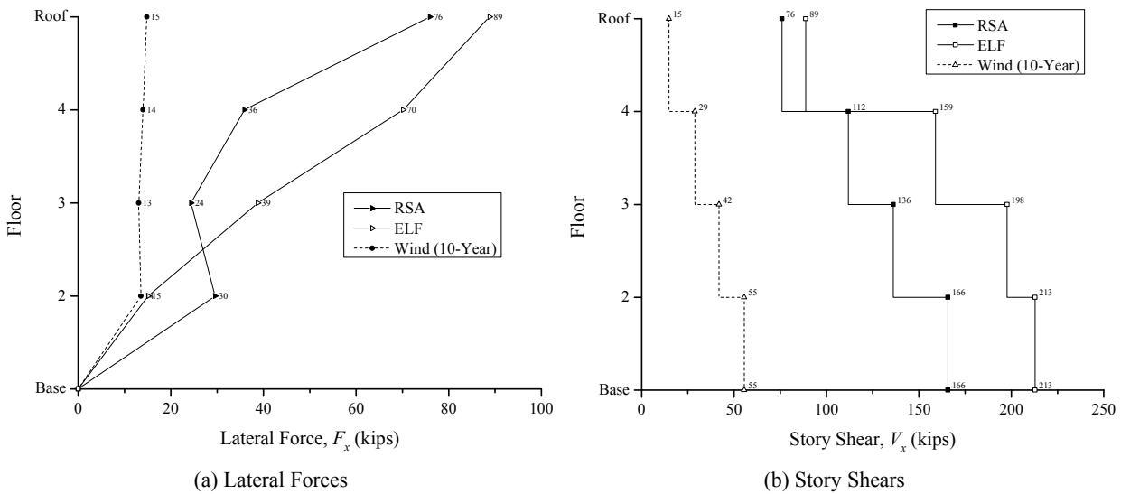
Figure B-2. Drift Design Lateral Forces and Story Shears
