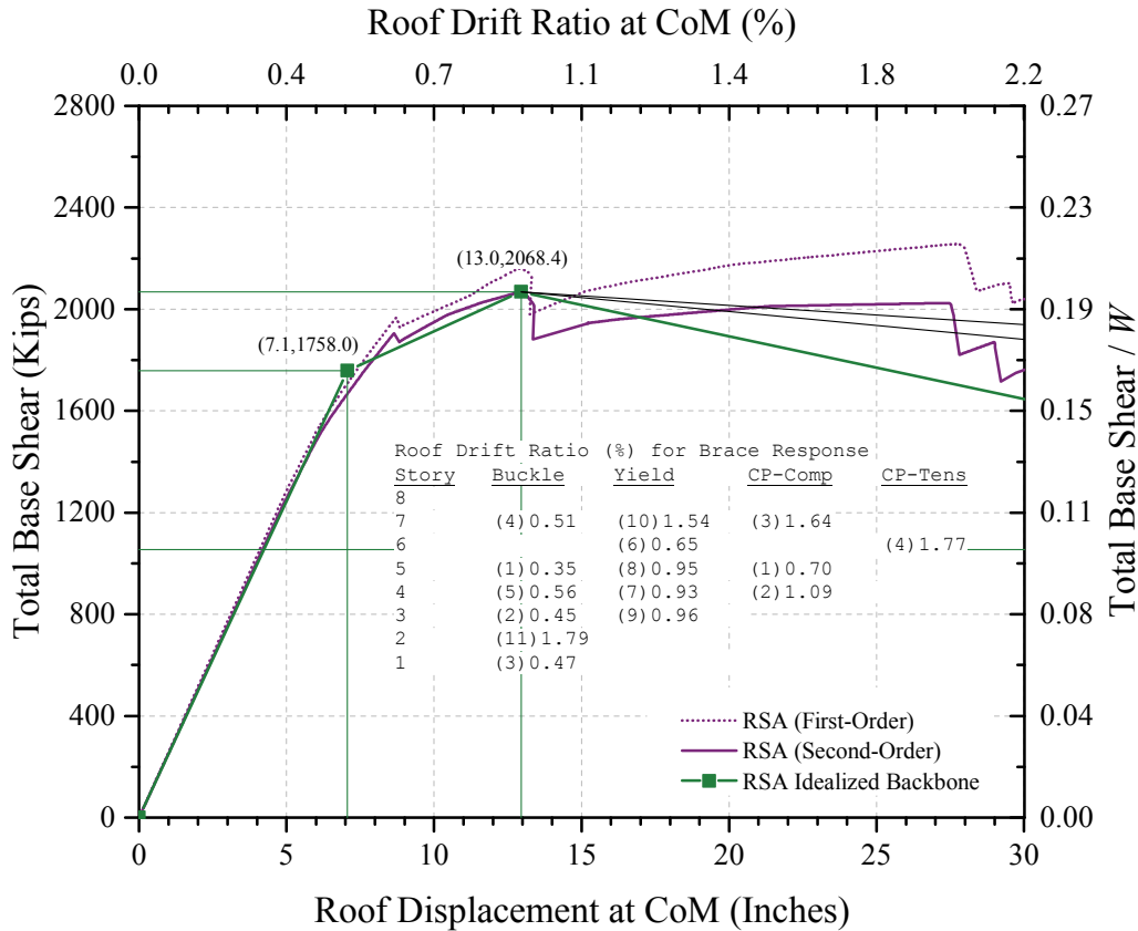
Figure 3-66. 8-Story SCBF RSA Pushover, BSE-2
