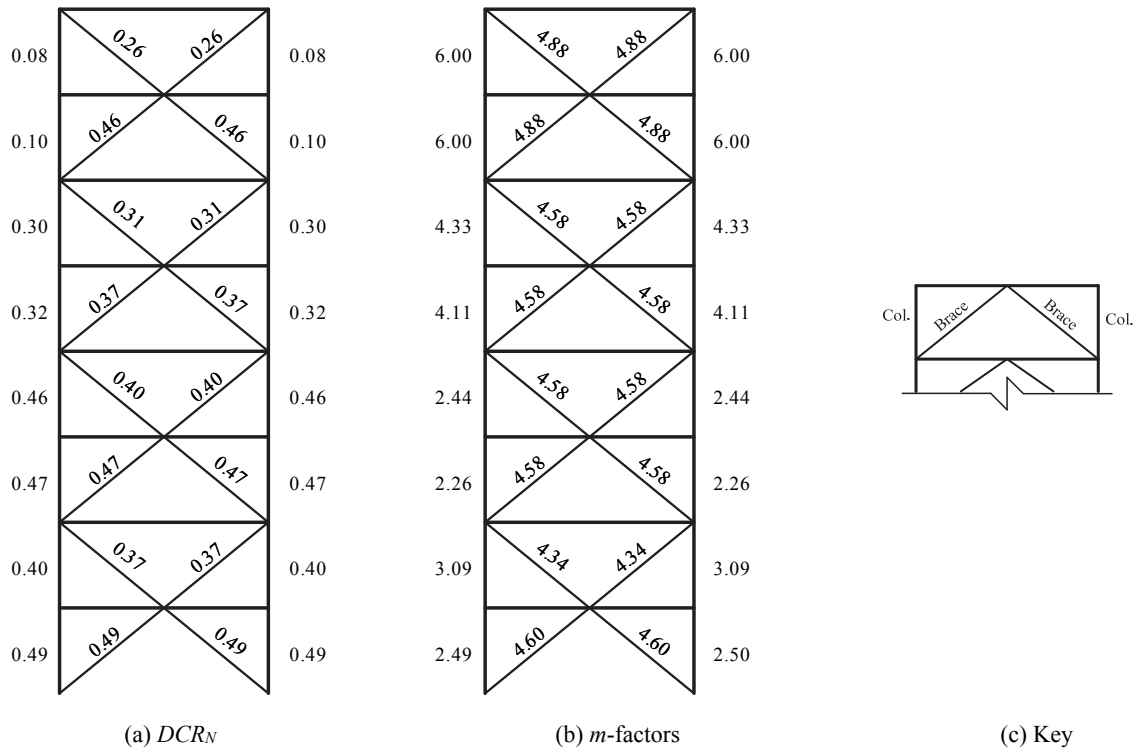
Figure 3-59. LDP Assessment Results, 8-Story SCBF ELF, BSE-1 LS
