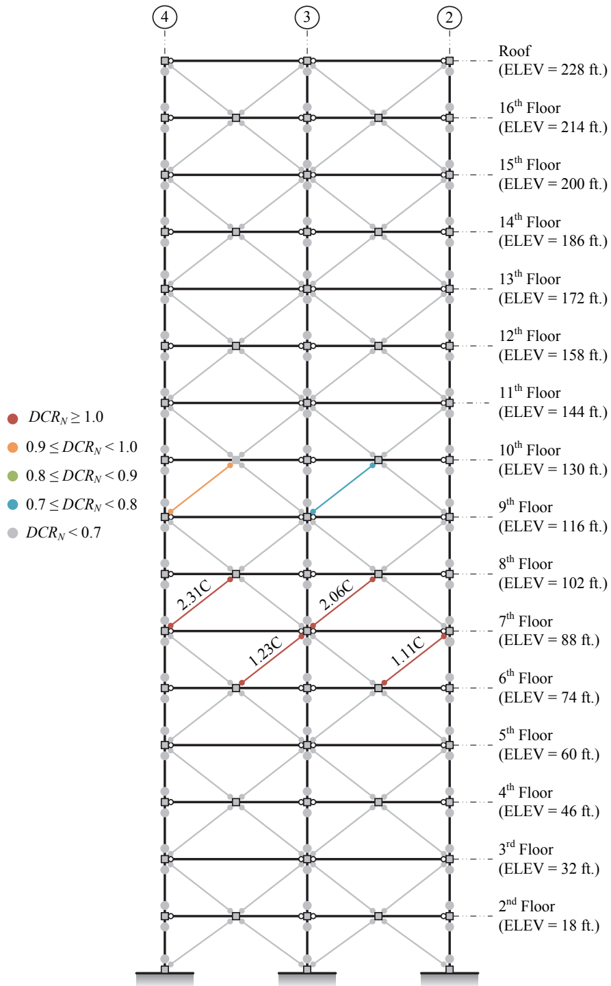
Figure 3-100. NSP Assessment Results, 16-Story SCBF RSA, BSE-1 LS (+push to left)
