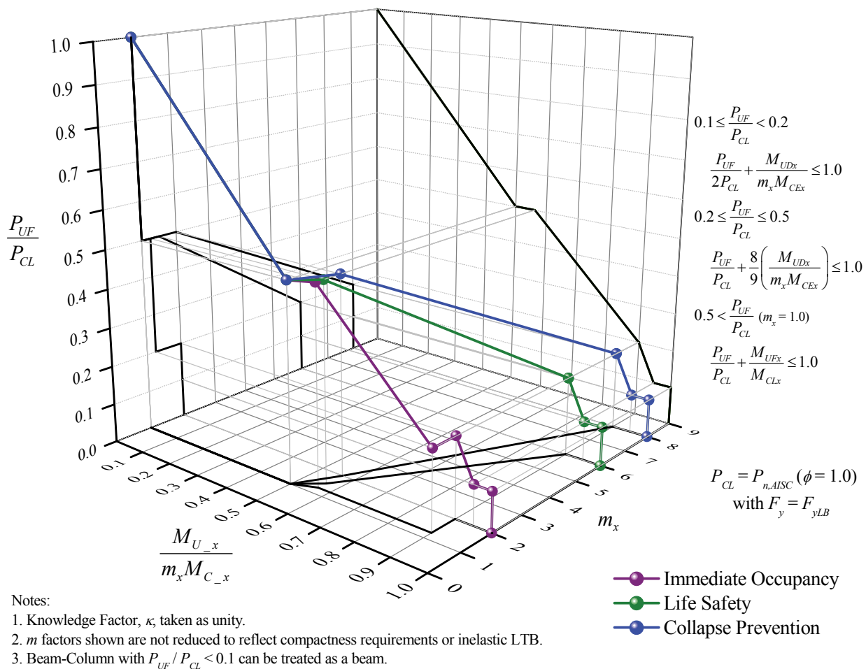
Figure 3-4. P - M Interaction on Section m -factor (in-plane) and Member Instability (Primary Component)
