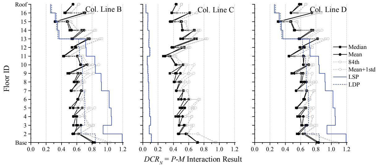
Figure 3-110. NDP Assessment Results, Column Members, 16-Story SCBF RSA, BSE-2
