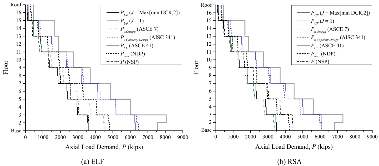
Figure 3-90. LDP Assessment Results, Compression in Ext. Columns, 16-Story SCBF, BSE-1
