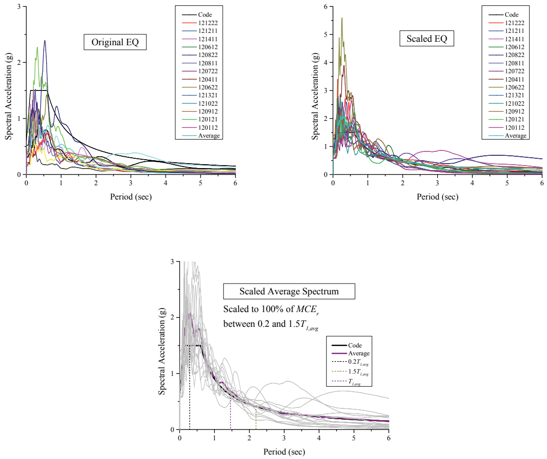
Figure A-3. Acceleration Response Spectra: Original, Scaled, and Scaled Average Spectrum for N-S Direction of MC8
