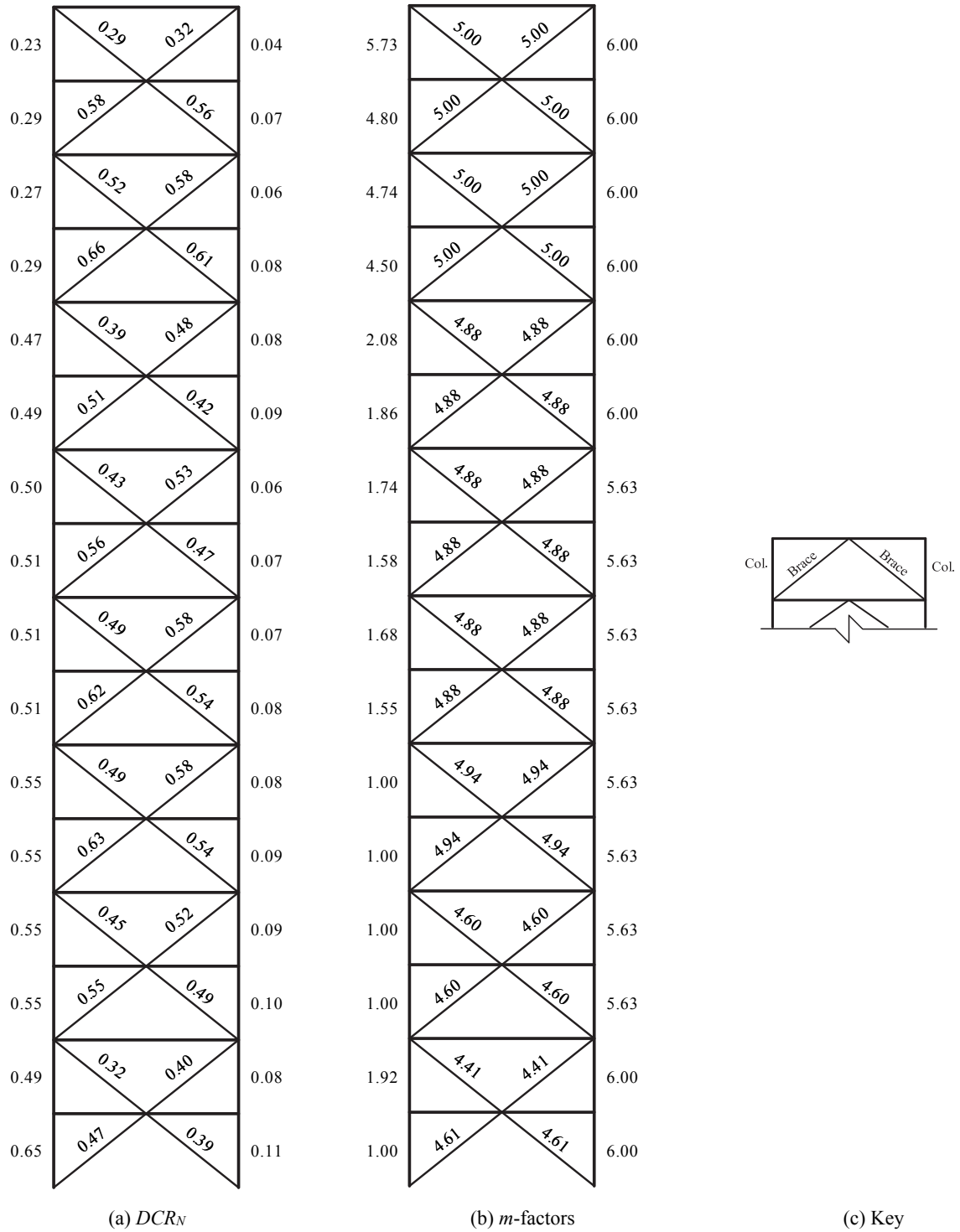
Figure 3-89. LDP Assessment Results, 16-Story SCBF RSA, BSE-1 LS
