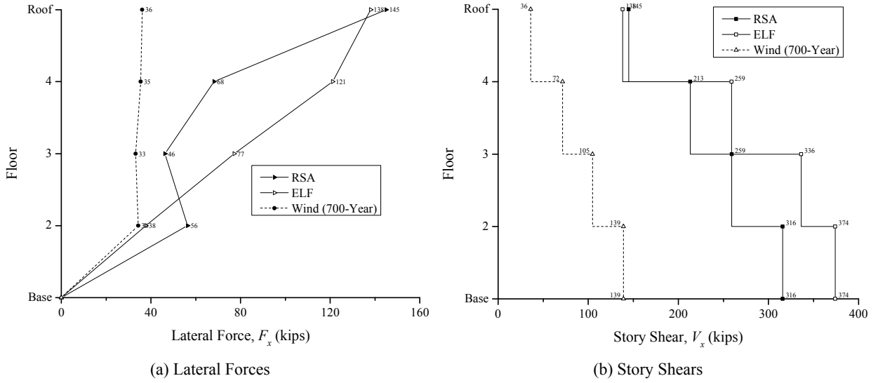
Figure B-1. Strength Design Lateral Forces and Story Shears
