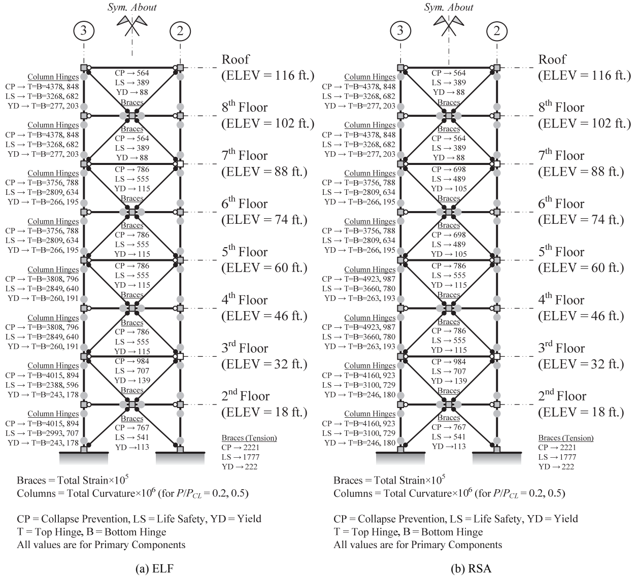
Figure 3-21. Frame Capacity Schematic (Inelastic), LS and CP, 8-Story SCBF ELF and RSA
