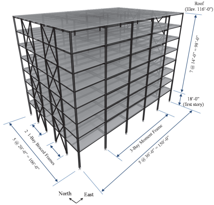
Figure 2-2. Isometric View of MC8 Archetype Building
