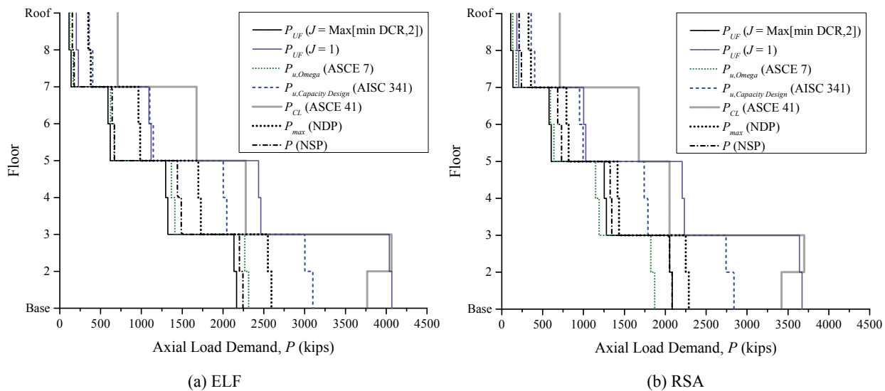
Figure 3-55. LSP Assessment Results, Compression in Ext. Columns, 8-Story SCBF, BSE-1
