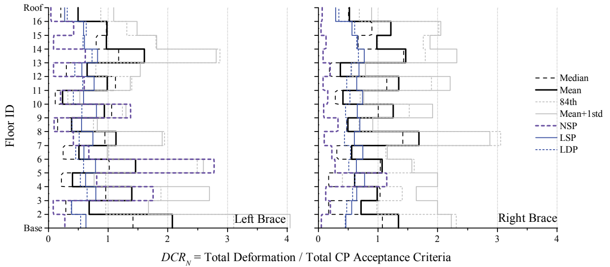
Figure 3-105. NDP Assessment Results, Brace Struts, 16-Story SCBF ELF, BSE-2 CP
