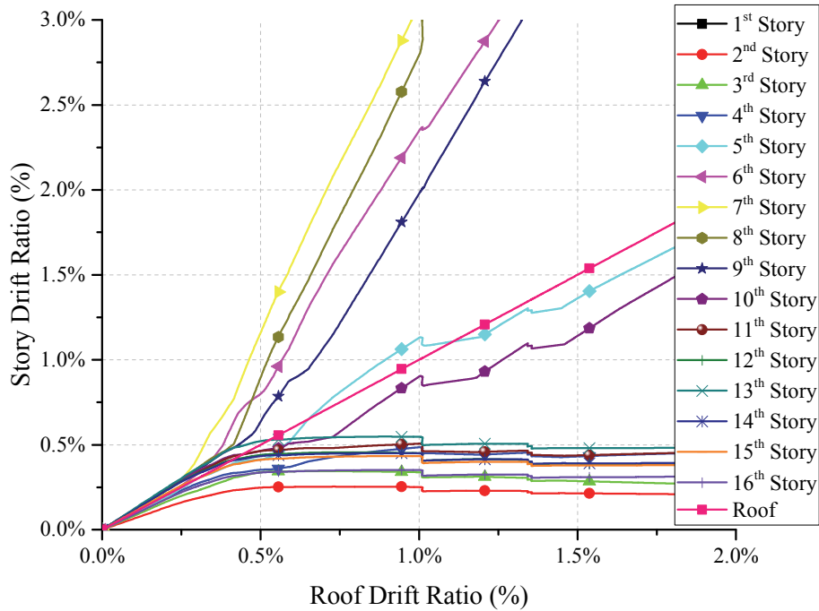
Figure 3-97. 16-Story SCBF RSA Pushover – Story Drift Ratios – BSE-2
