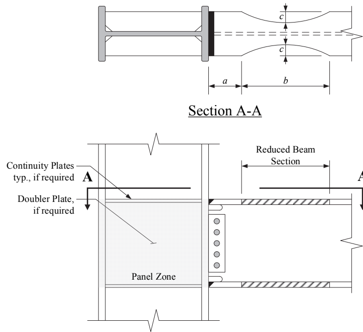
Figure 2-6. Typical FR RBS Beam-to-Column Connection Assembly
