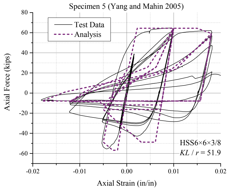
Figure 3-14. PERFORM-3D Brace Calibration
