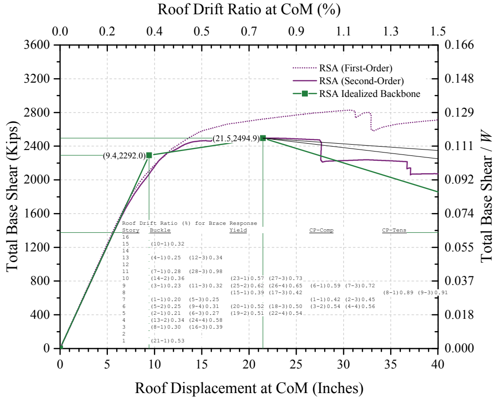
Figure 3-95. 16-Story SCBF RSA Pushover, BSE-2
