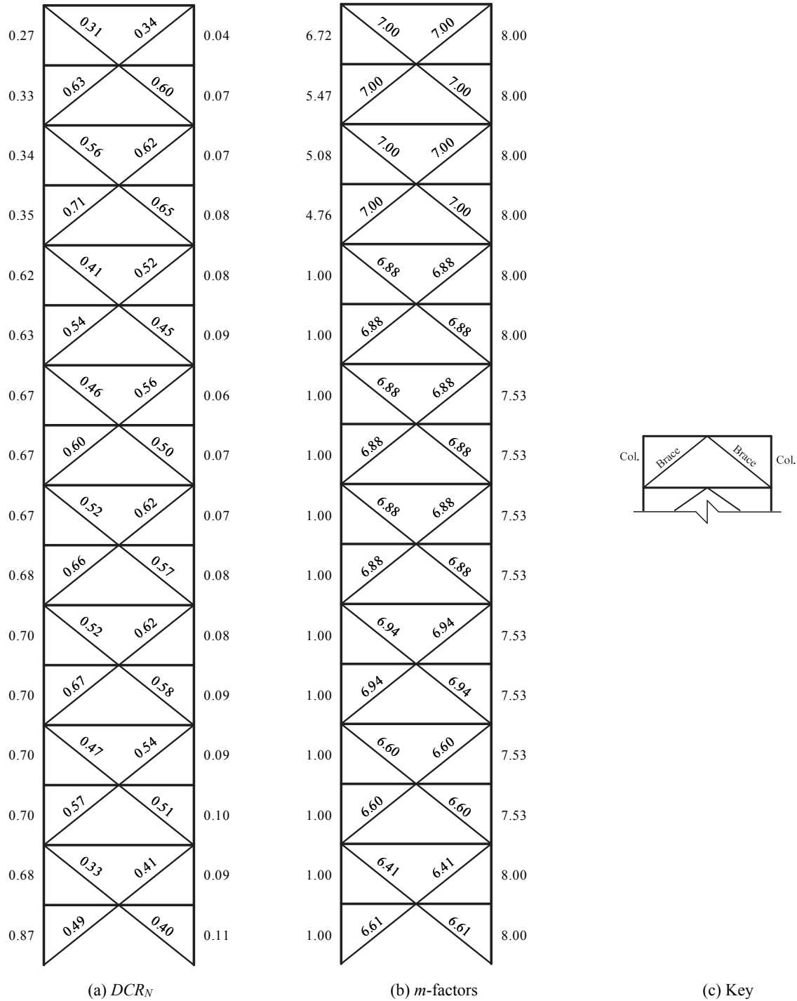
Figure 3-92. LDP Assessment Results, 16-Story SCBF RSA, BSE-2 CP
