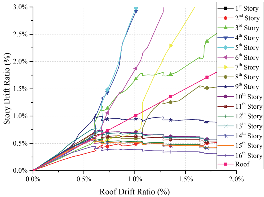
Figure 3-96. 16-Story SCBF ELF Pushover – Story Drift Ratios – BSE-2
