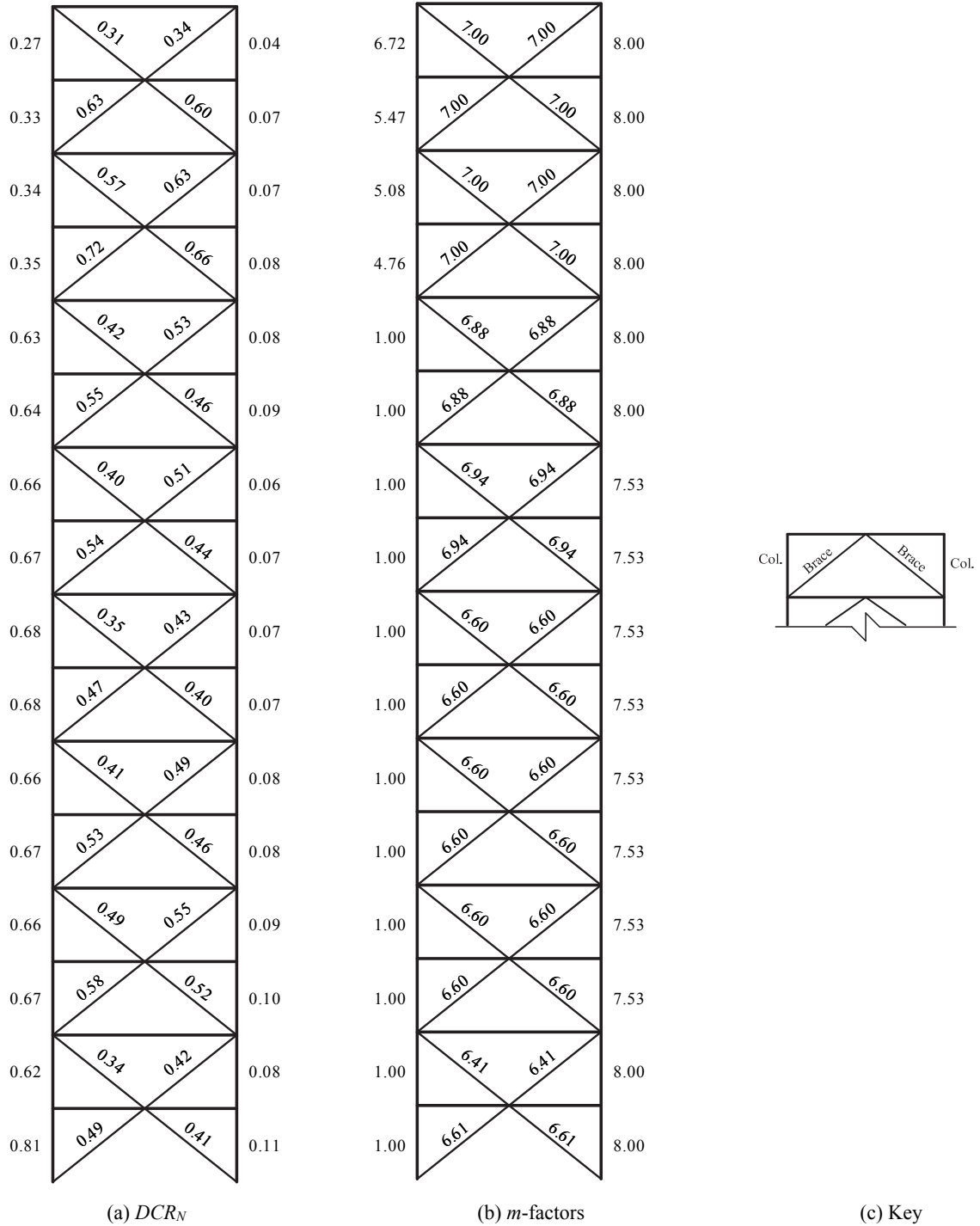
Figure 3-91. LDP Assessment Results, 16-Story SCBF ELF, BSE-2 CP
