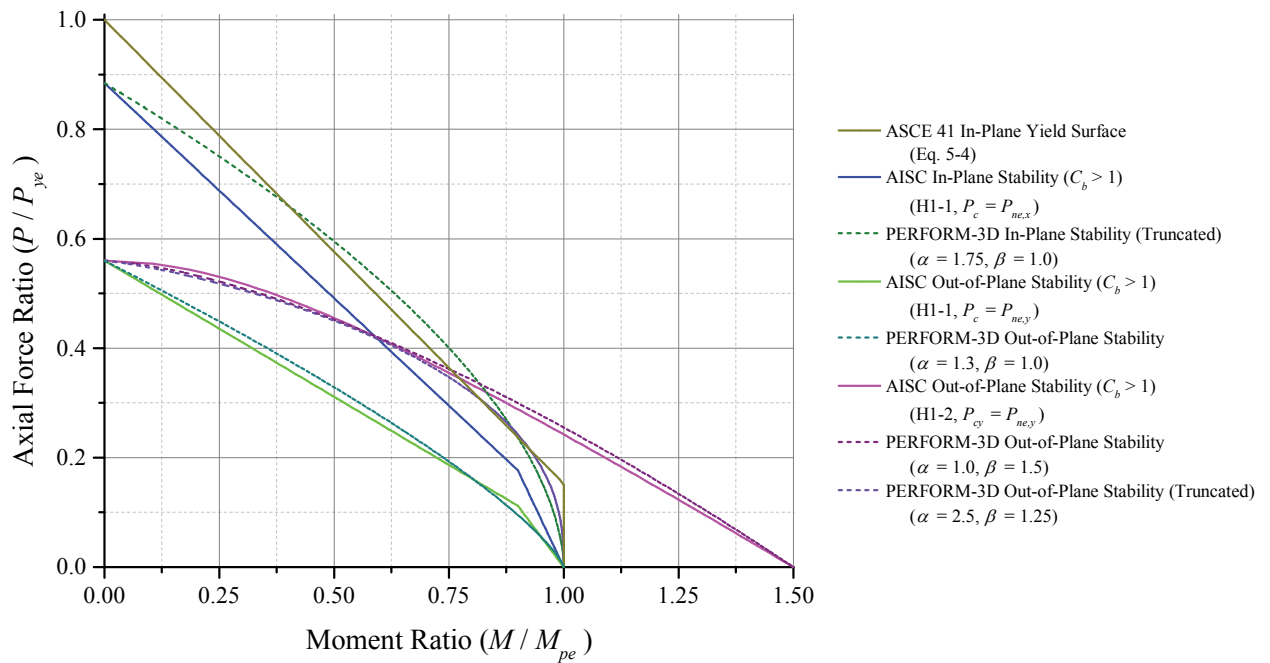
Figure 3-19. P-M Interaction Curve (Member Instability)
