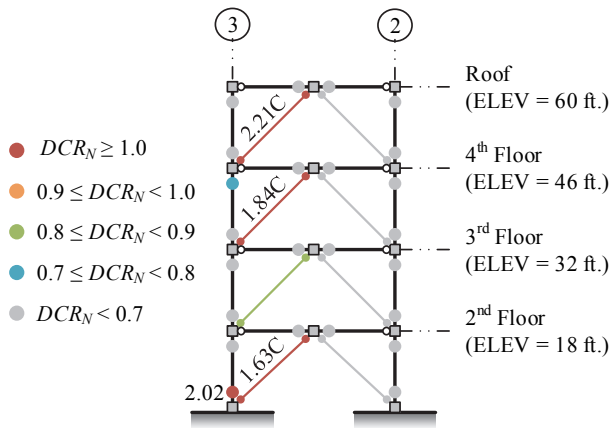
Figure 3-43. NSP Assessment Results, 4-Story SCBF ELF, BSE-2 CP (+push to left)
