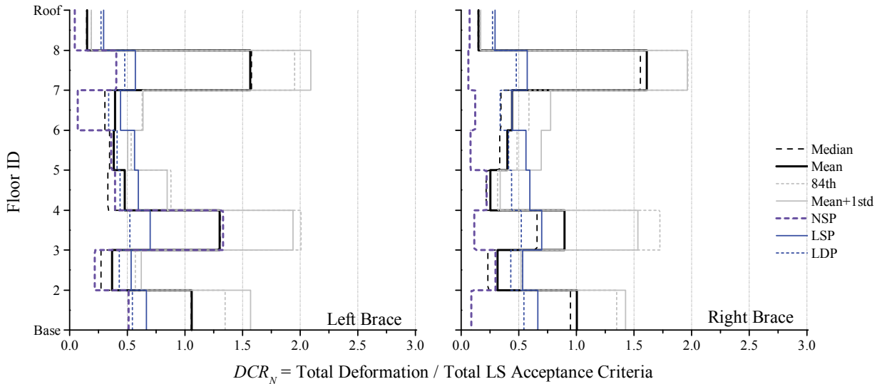
Figure 3-74. NDP Assessment Results, Brace Struts, 8-Story SCBF ELF, BSE-1 LS
