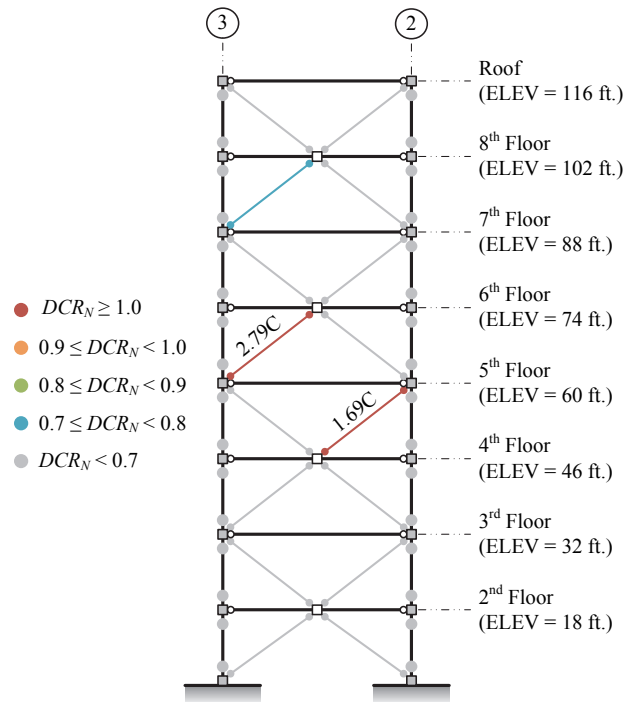
Figure 3-73. NSP Assessment Results, 8-Story SCBF RSA, BSE-2 CP (+push to left)
