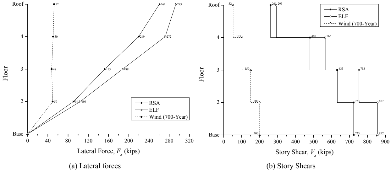
Figure B-10. Strength Design Lateral Forces and Story Shears
