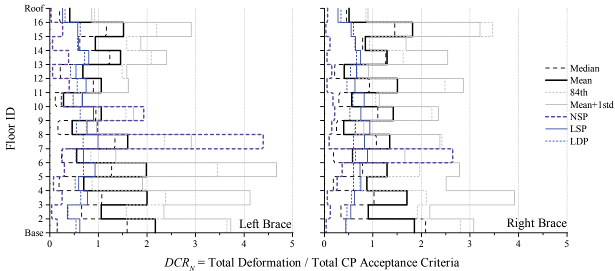
Figure 3-106. NDP Assessment Results, Brace Struts, 16-Story SCBF RSA, BSE-2 CP
