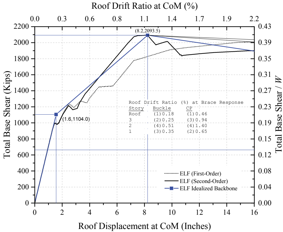
Figure 3-36. 4-Story SCBF ELF Pushover, BSE-2
