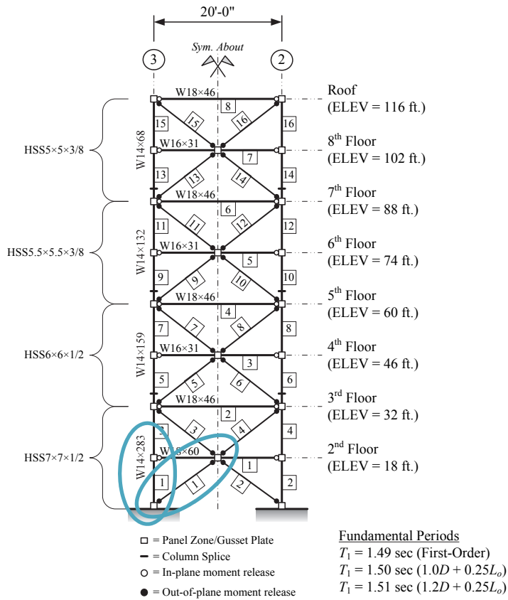
Figure B-19. SCBF Member Sizes, 8-Story RSA
