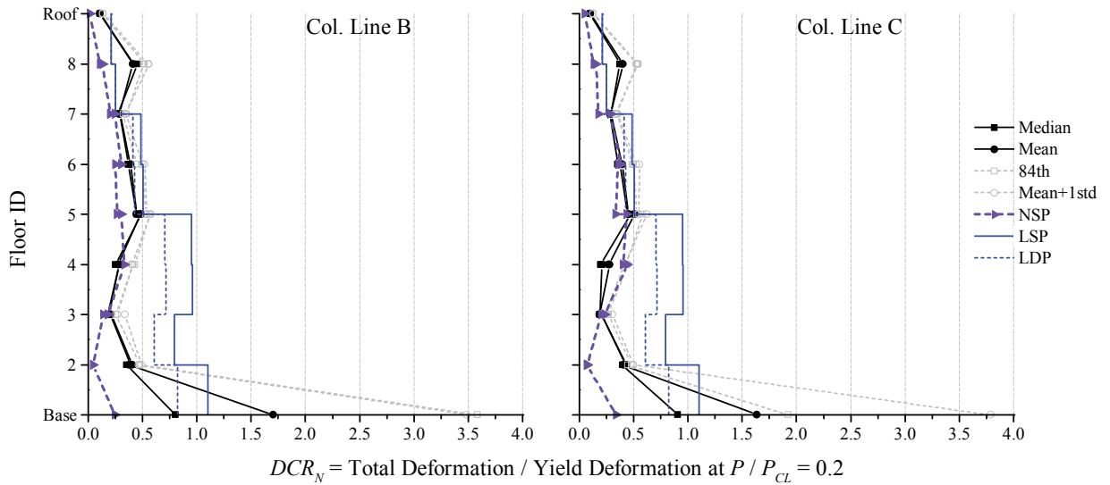
Figure 3-79. NDP Assessment Results, Column Hinges, 8-Story SCBF RSA, BSE-2 Yield
