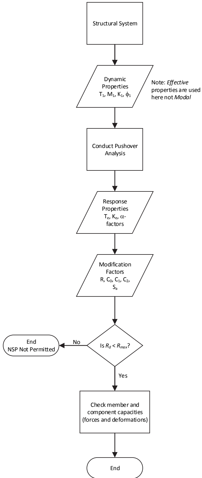
Figure 3-3. NSP Process
