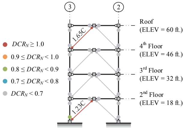
Figure 3-41. NSP Assessment Results, 4-Story SCBF ELF, BSE-1 LS (+push to left)
