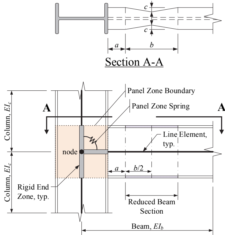
Figure 2-7. FR RBS Beam-To-Column Connection Subassembly Model for Linear Analysis
