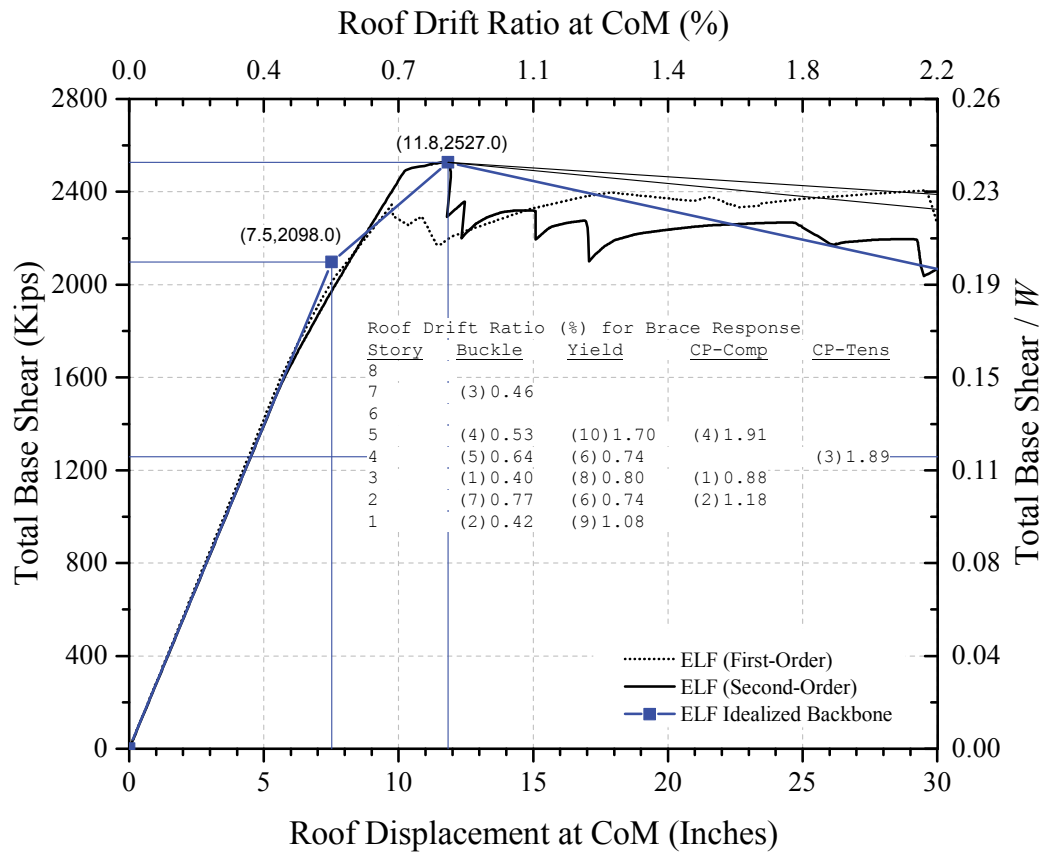
Figure 3-65. 8-Story SCBF ELF Pushover, BSE-2
