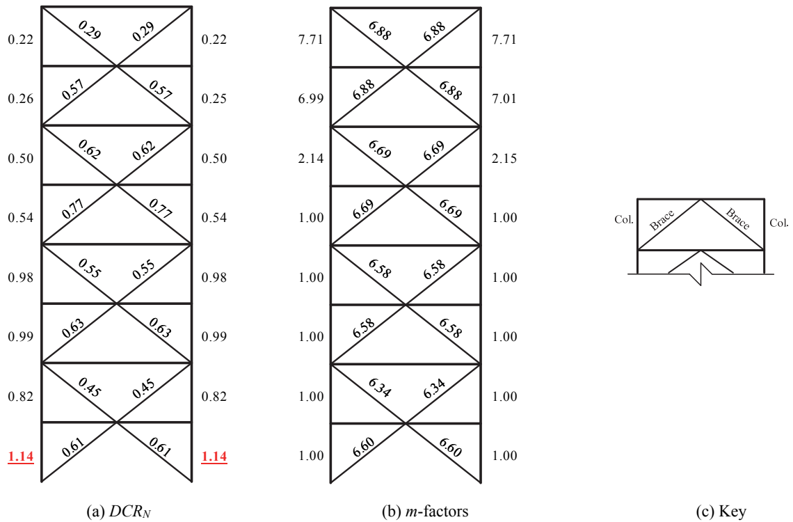
Figure 3-57. LSP Assessment Results, 8-Story SCBF RSA, BSE-2 CP
