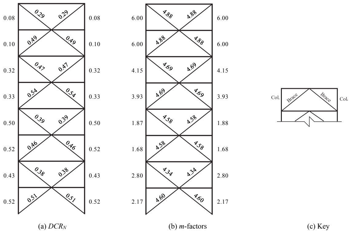
Figure 3-60. LDP Assessment Results, 8-Story SCBF RSA, BSE-1 LS
