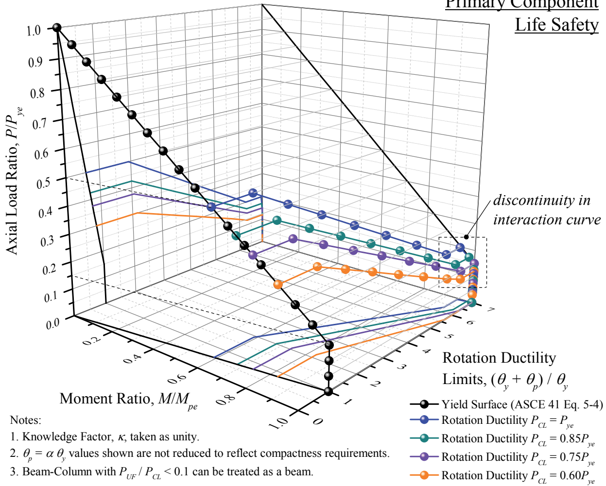
Figure 3-17. P-M Interaction on Plastic Rotation, LS Acceptance Criteria (Primary Component)
