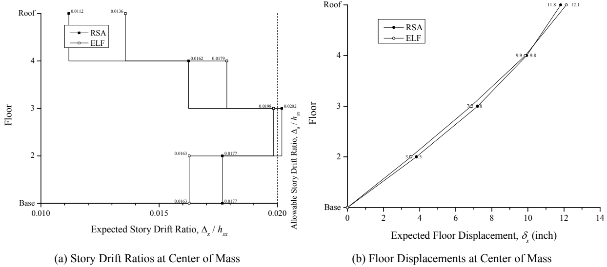
Figure B-3. Story Drift Ratios and Deflected Shape
