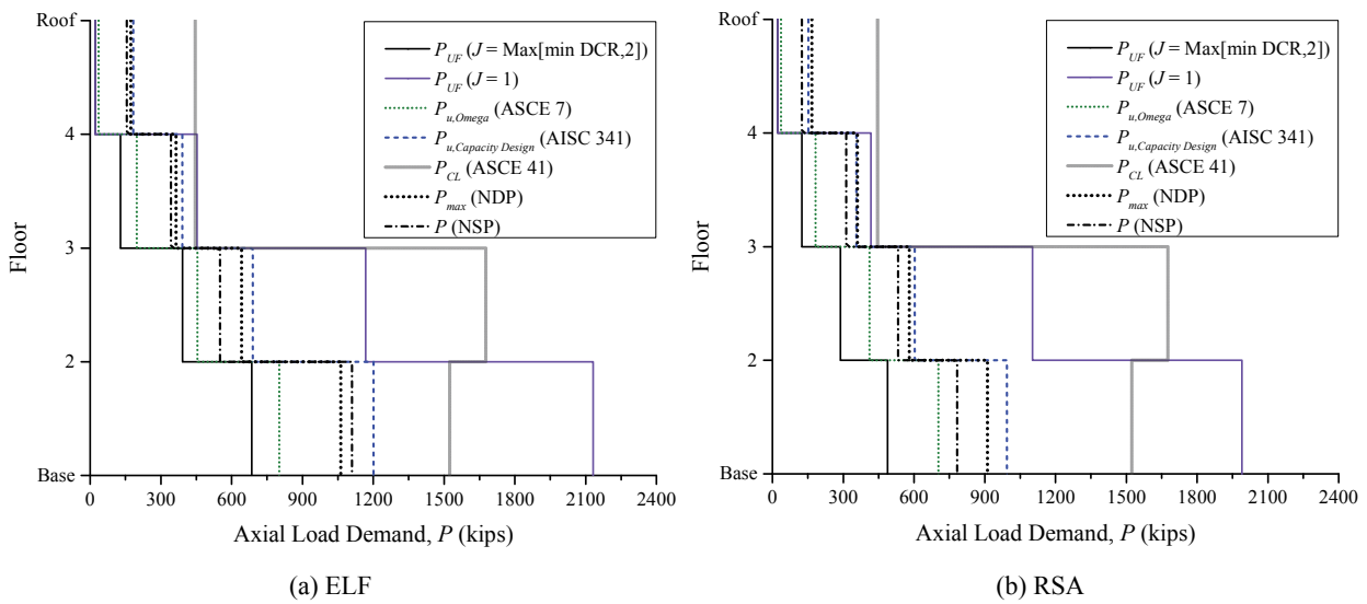
Figure 3-35. LDP Assessment Results, Compression in Ext. Columns, 4-Story SCBF, BSE-2
