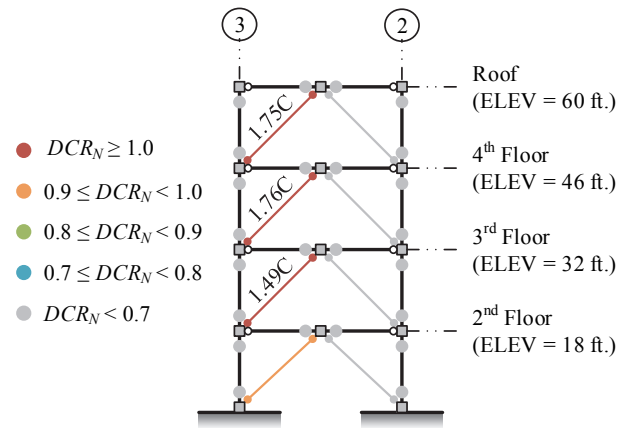
Figure 3-44. NSP Assessment Results, 4-Story SCBF RSA, BSE-2 CP (+push to left)
