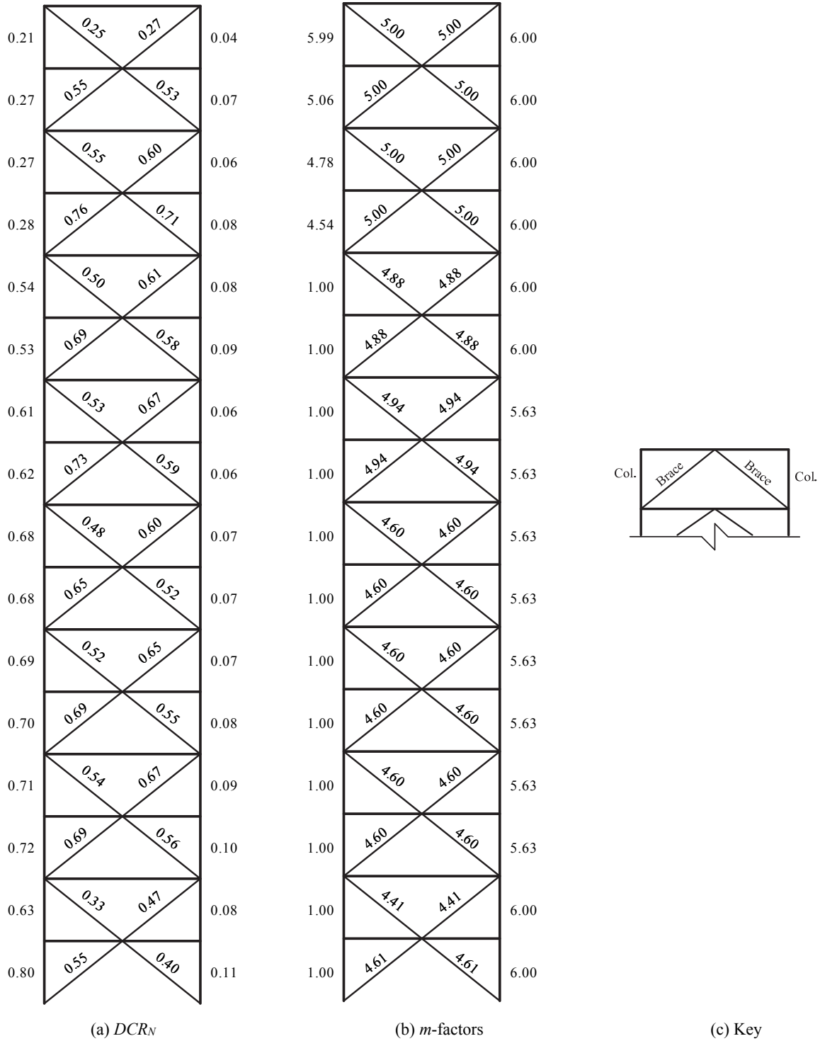
Figure 3-82. LSP Assessment Results, 16-Story SCBF ELF, BSE-1 LS
