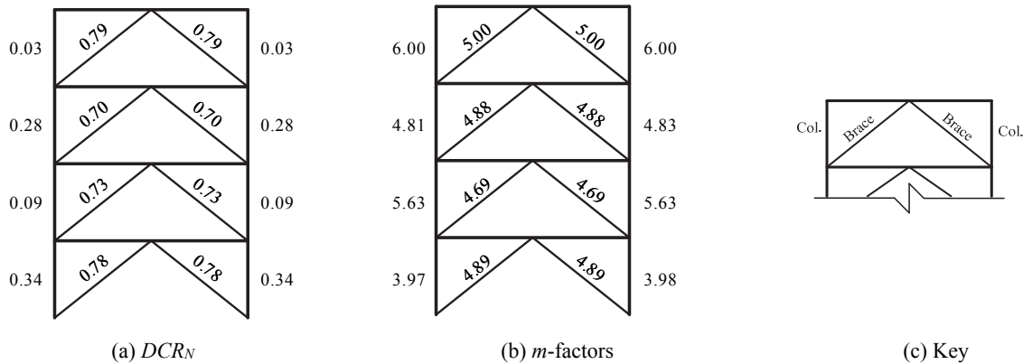
Figure 3-31. LDP Assessment Results, 4-Story SCBF RSA, BSE-1 LS
