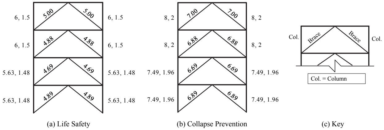
Figure 3-8. Frame Capacity Schematic ( m -factor), LS and CP, 4-Story SCBF RSA
