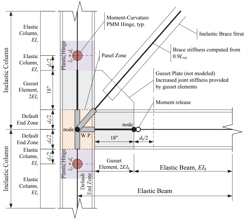
Figure 3-13. SCBF Brace-to-Beam / Column Subassembly Analytical Schematic
