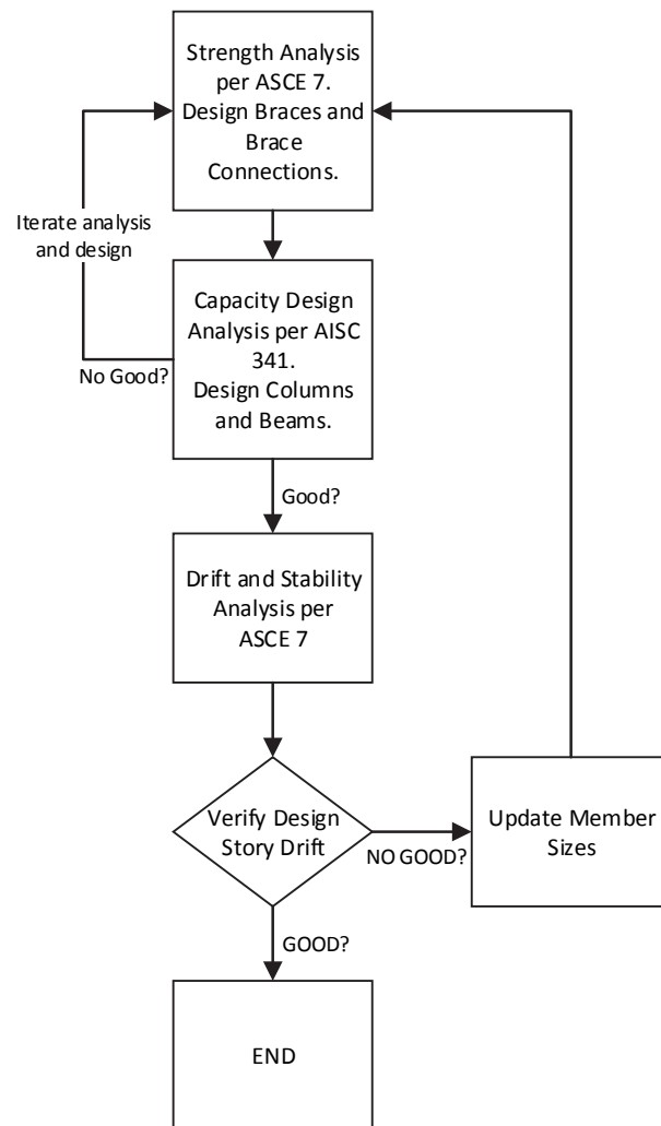
Figure 2-14. Flow Chart of SCBF Design Process
