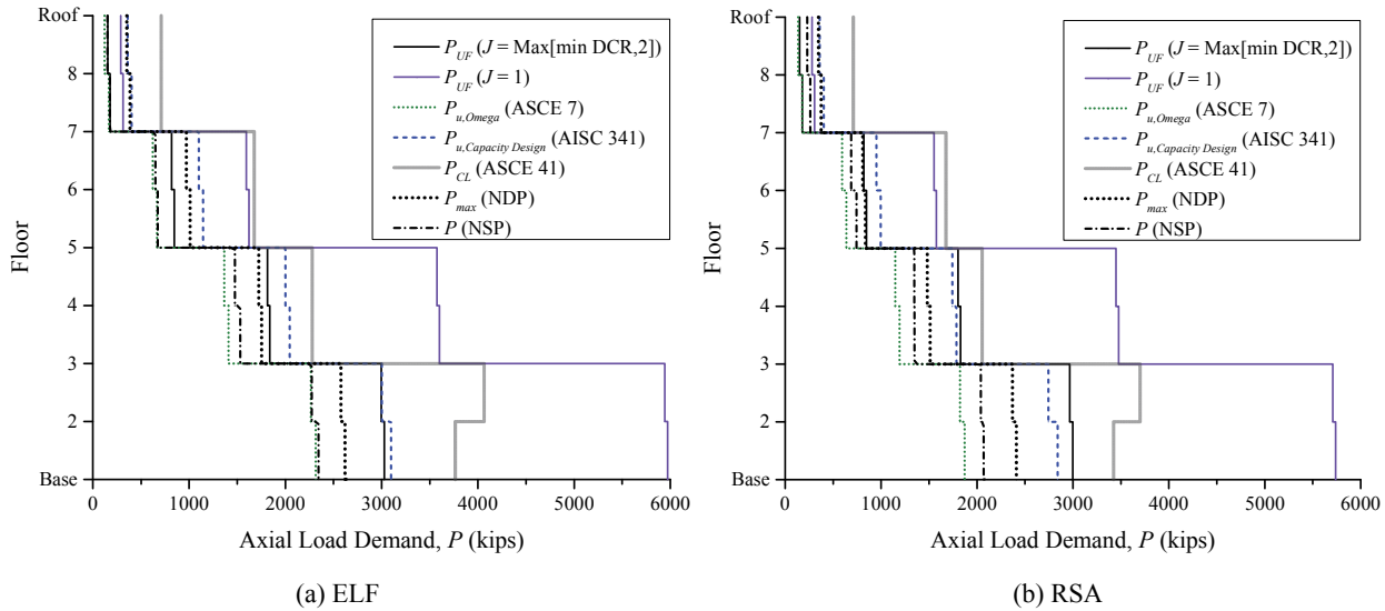
Figure 3-58. LSP Assessment Results, Compression in Ext. Columns, 8-Story SCBF, BSE-2
