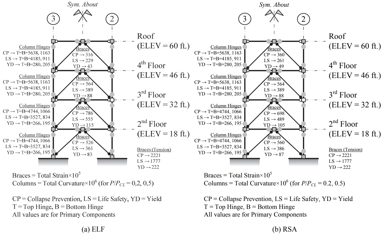
Figure 3-20. Frame Capacity Schematic (Inelastic), LS and CP, 4-Story SCBF ELF and RSA
