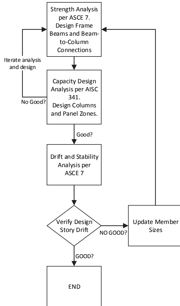
Figure 2-10. Flow Chart of SMF Design Process
