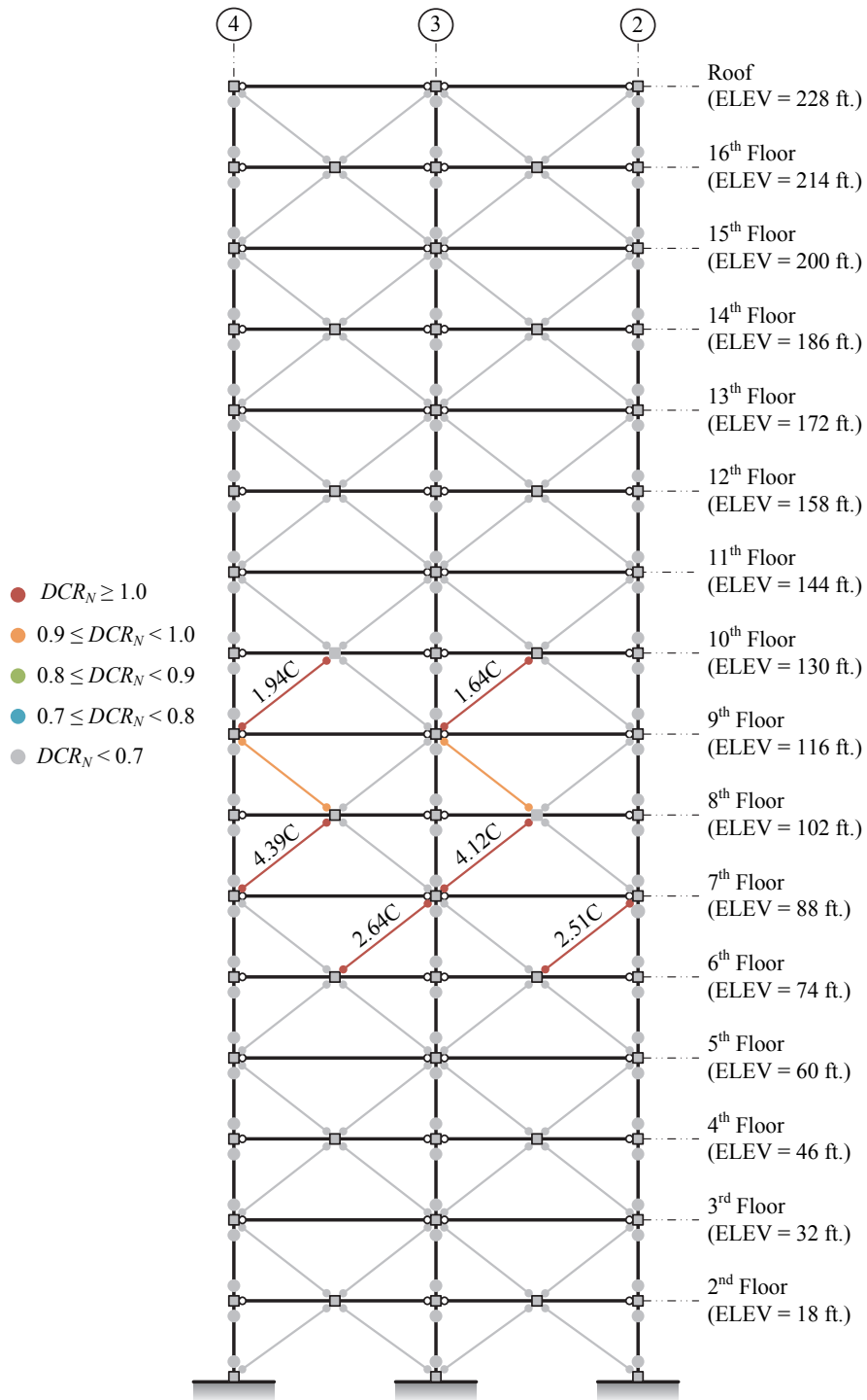
Figure 3-102. NSP Assessment Results, 16-Story SCBF RSA, BSE-2 CP (+push to left)
