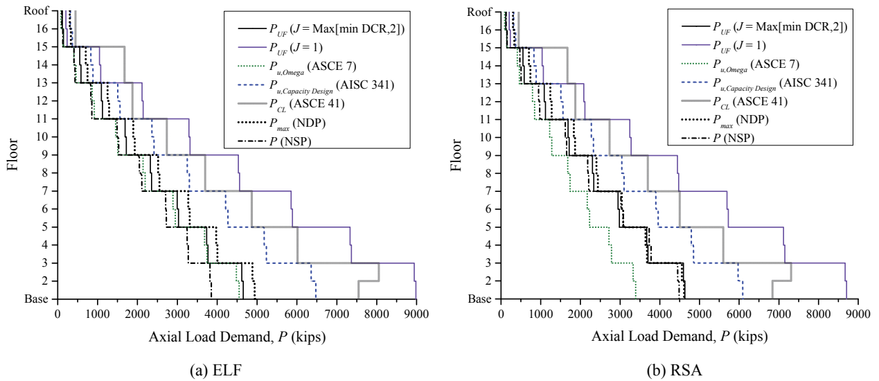
Figure 3-93. LDP Assessment Results, Compression in Ext. Columns, 16-Story SCBF, BSE-2
