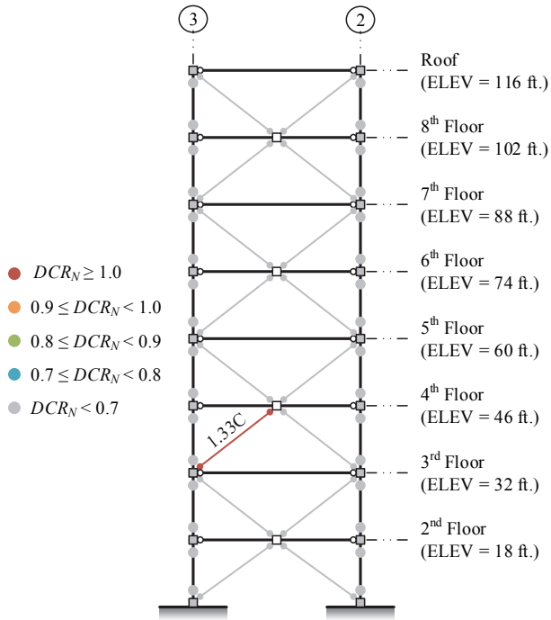
Figure 3-70. NSP Assessment Results, 8-Story SCBF ELF, BSE-1 LS (+push to left)
