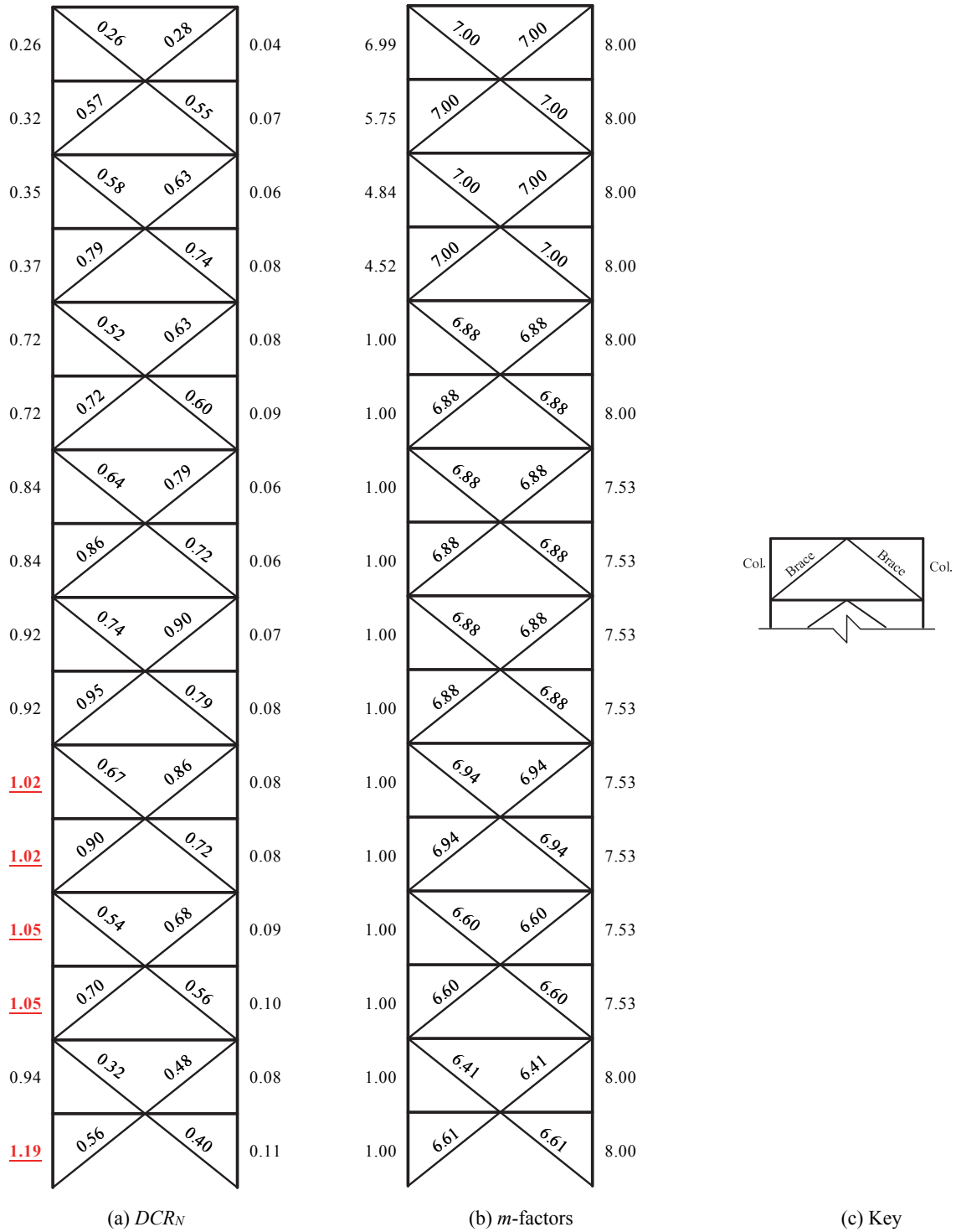
Figure 3-86. LSP Assessment Results, 16-Story SCBF RSA, BSE-2 CP
