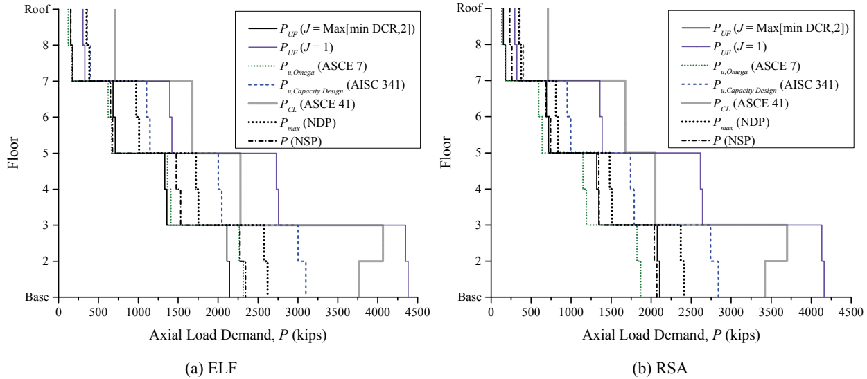
Figure 3-64. LDP Assessment Results, Compression in Ext. Columns, 8-Story SCBF, BSE-2
