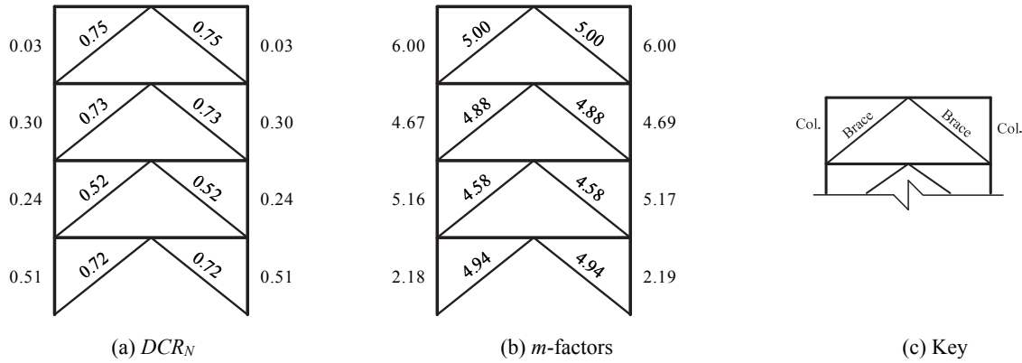
Figure 3-30. LDP Assessment Results, 4-Story SCBF ELF, BSE-1 LS
