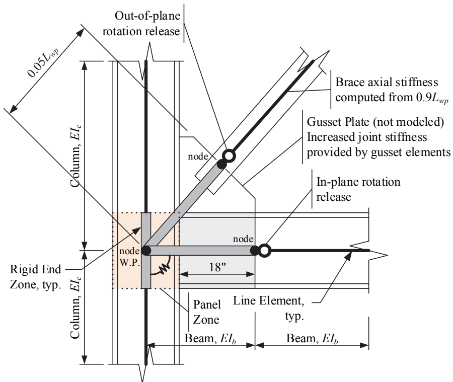
Figure 2-9. Brace-to-Beam / Column Connection Subassembly Model for Linear Analysis
