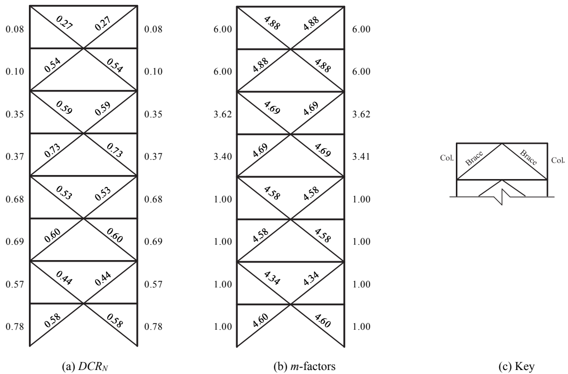
Figure 3-54. LSP Assessment Results, 8-Story SCBF RSA, BSE-1 LS
