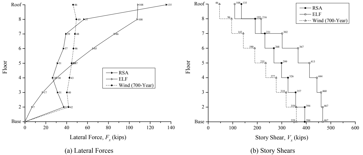
Figure B-4. Strength Design Lateral Forces and Story Shears
