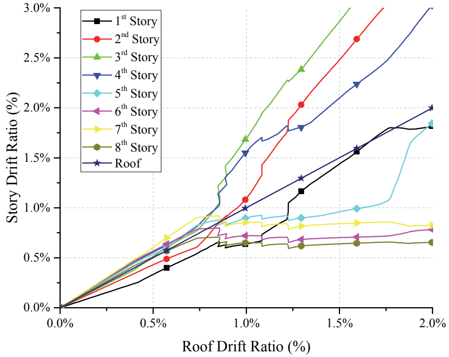
Figure 3-67. 8-Story SCBF ELF Pushover – Story Drift Ratios – BSE-2
