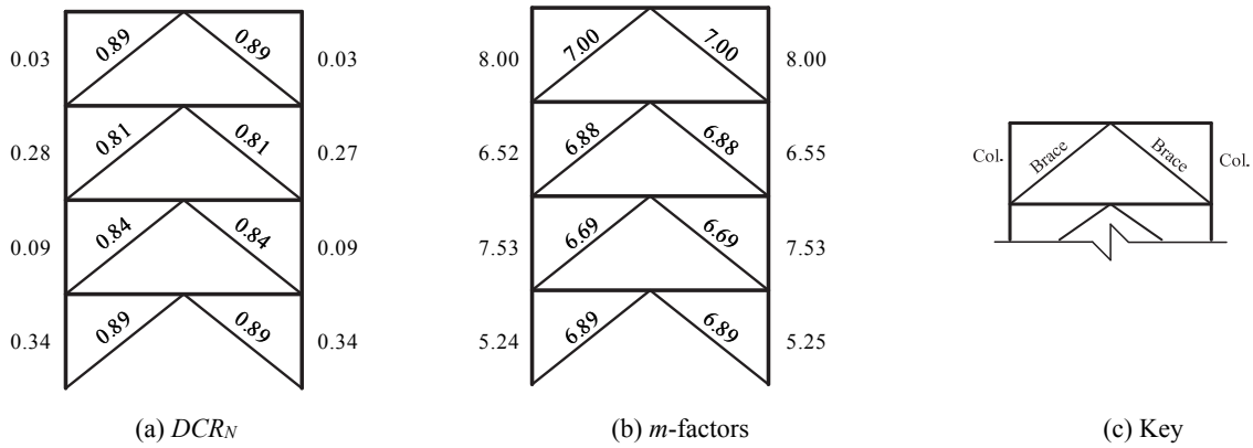
Figure 3-28. LSP Assessment Results, 4-Story SCBF RSA, BSE-2 CP
