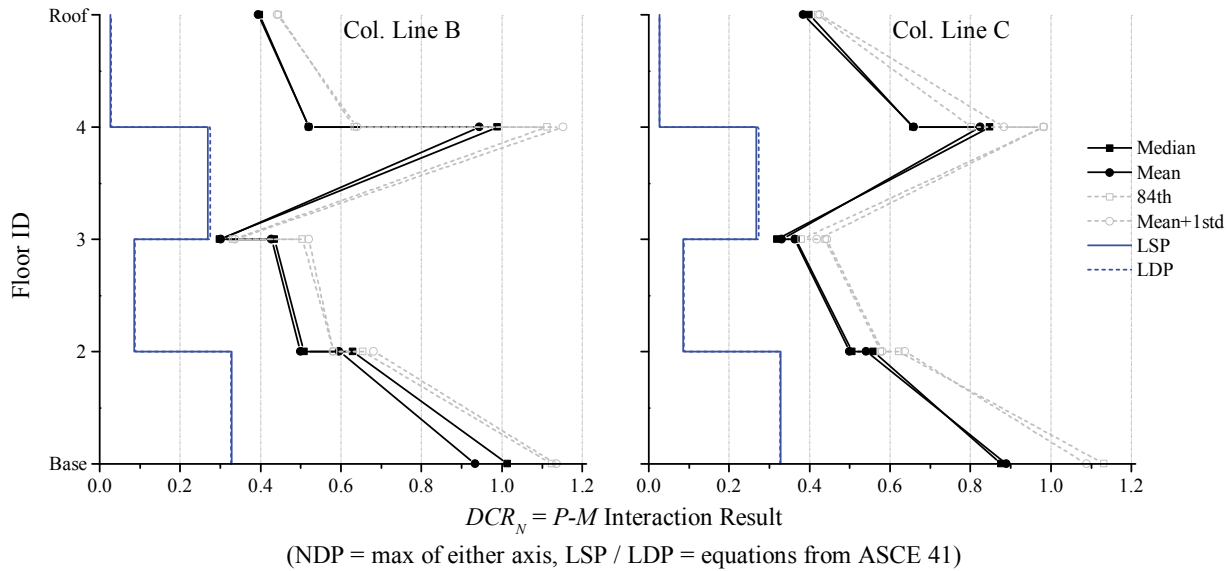
Figure 3-52. NDP Assessment Results, Column Members, 4-Story SCBF RSA, BSE-2
