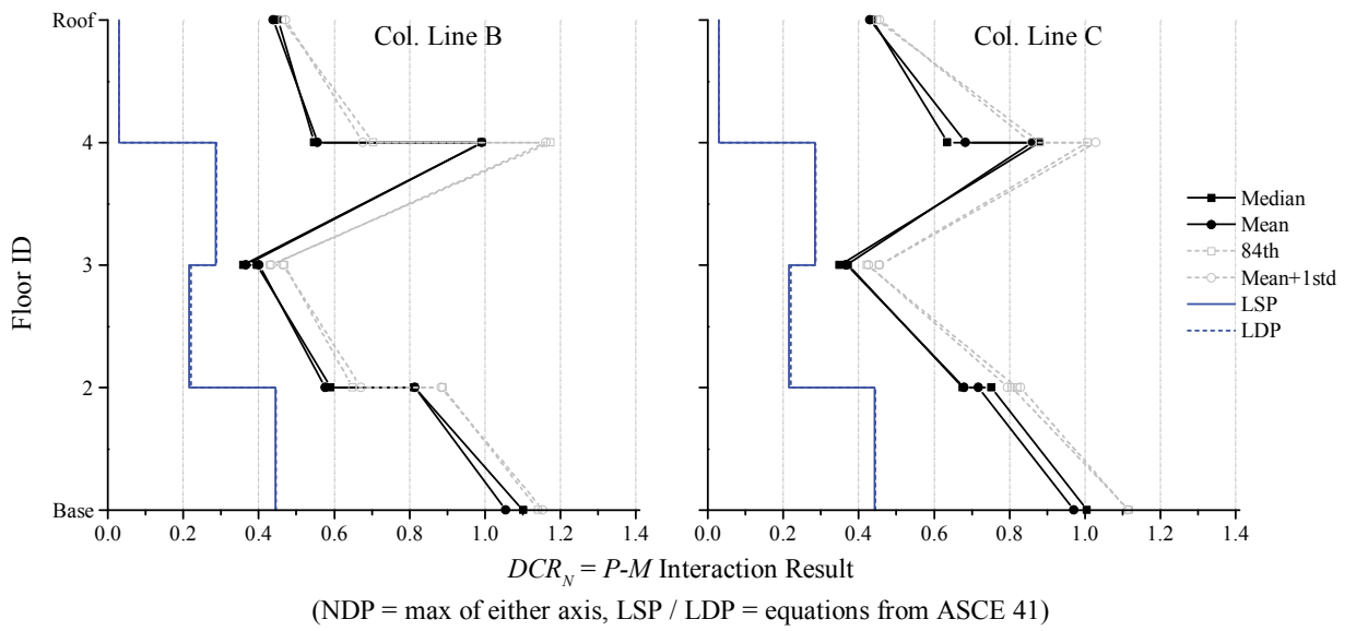
Figure 3-51. NDP Assessment Results, Column Members, 4-Story SCBF ELF, BSE-2
