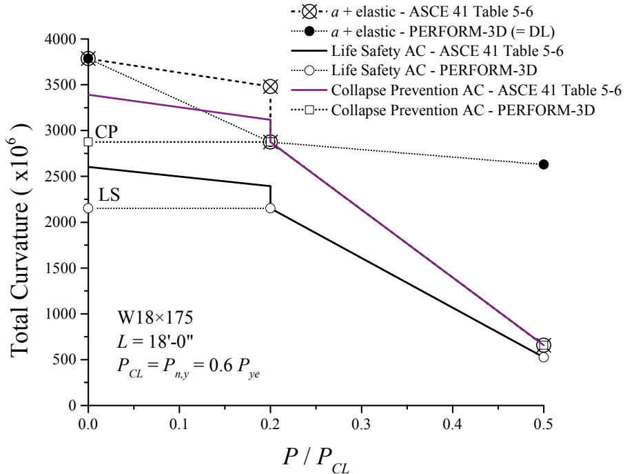
Figure 3-16. Variation in Acceptance Criteria and Hinge Model for Axial Force
