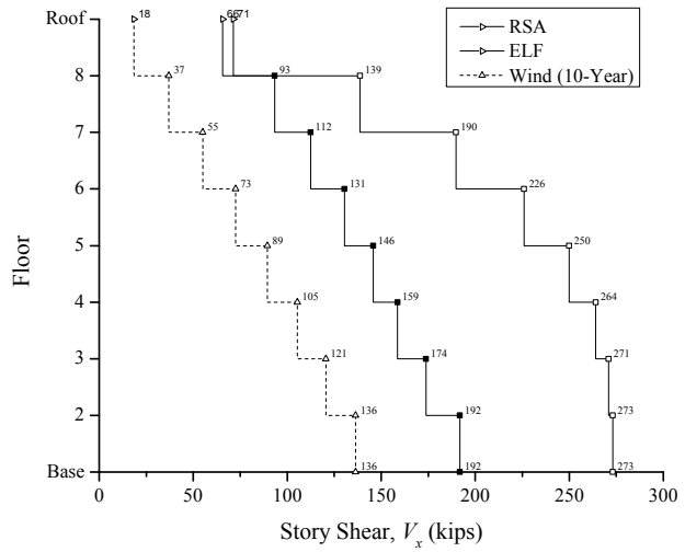
(b) Story Shears
