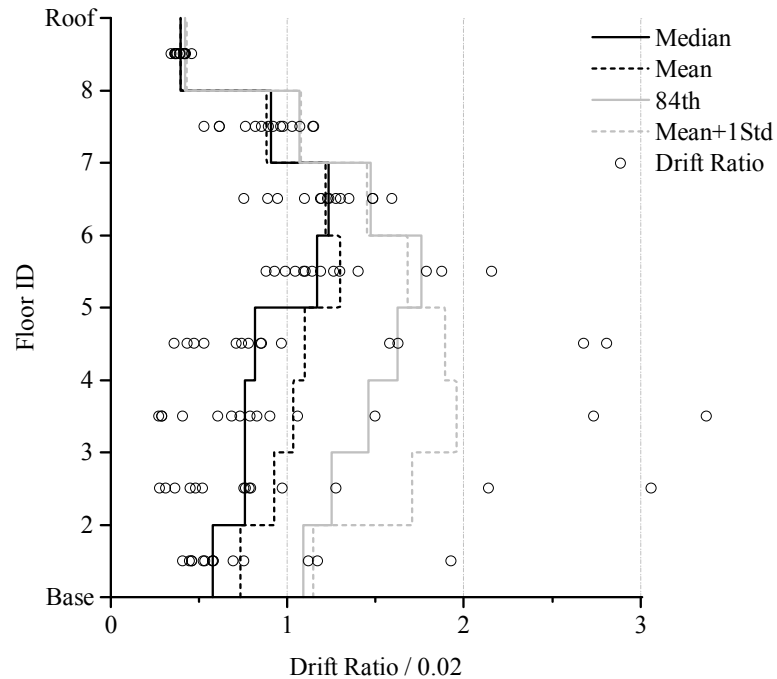
Figure 3-112. NDP Assessment Results, Story Drift Ratios, 8-Story SCBF RSA, BSE-2 CP
