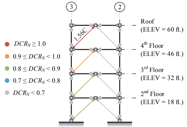
Figure 3-42. NSP Assessment Results, 4-Story SCBF RSA, BSE-1 LS (+push to left)
