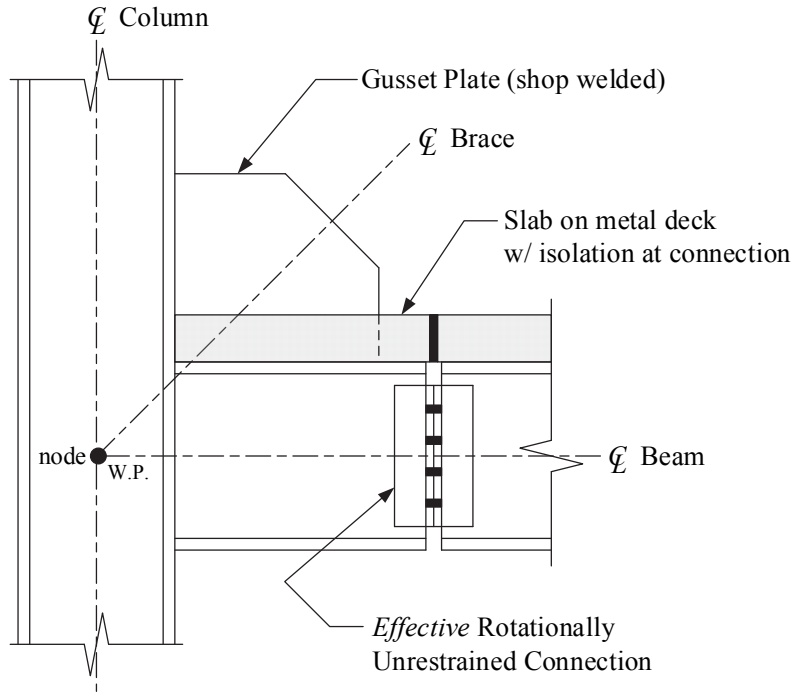
Figure 2-8. Typical Brace-to-Beam / Column Connection Assembly
