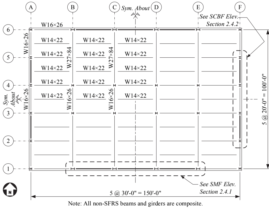
Figure 2-4. Typical Floor Framing Plan, MC4 and MC8
