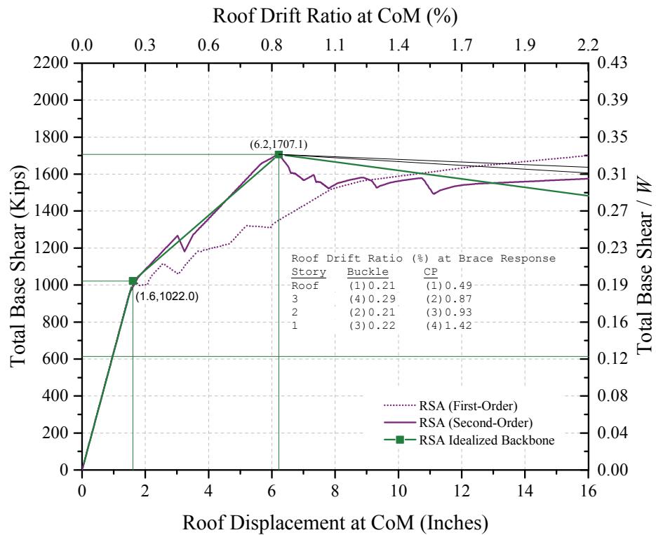
Figure 3-37. 4-Story SCBF RSA Pushover, BSE-2
