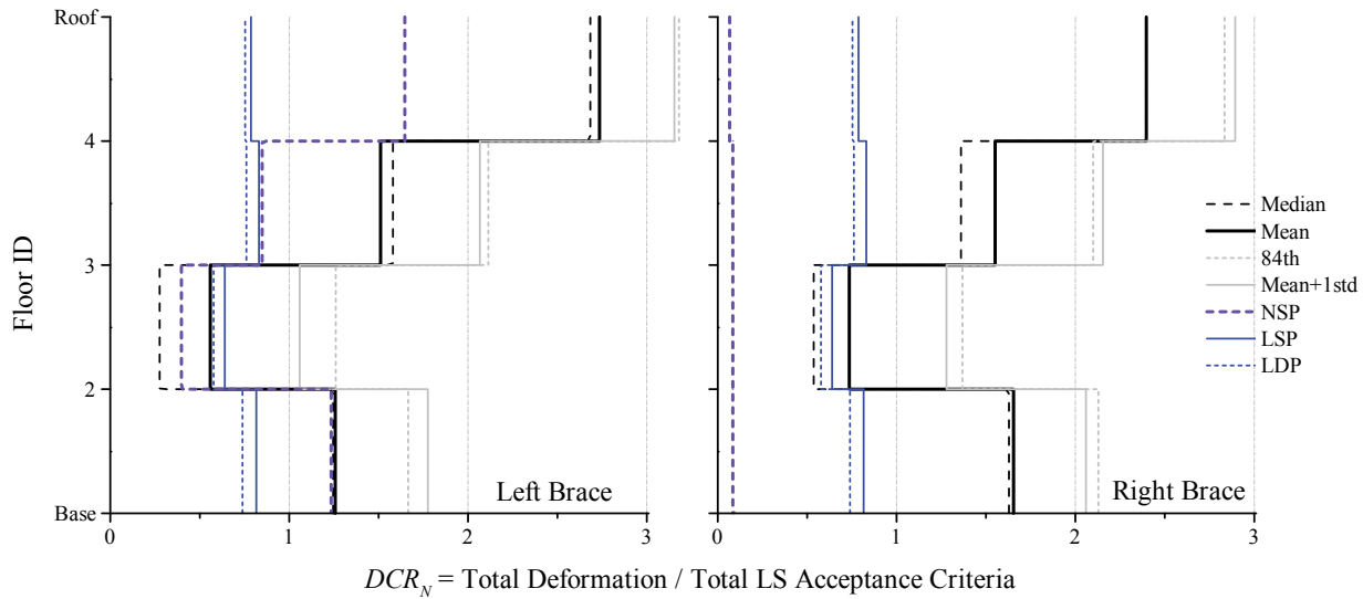
Figure 3-45. NDP Assessment Results, Brace Struts, 4-Story SCBF ELF, BSE-1 LS
