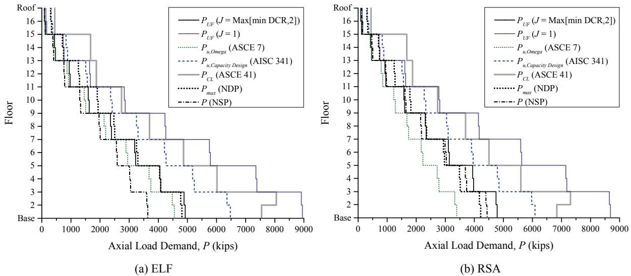
Figure 3-84. LSP Assessment Results, Compression in Ext. Columns, 16-Story SCBF, BSE-1
