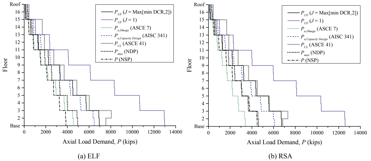
Figure 3-87. LSP Assessment Results, Compression in Ext. Columns, 16-Story SCBF, BSE-2
