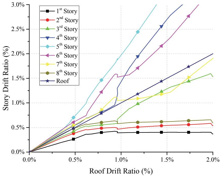
Figure 3-68. 8-Story SCBF RSA Pushover – Story Drift Ratios – BSE-2
