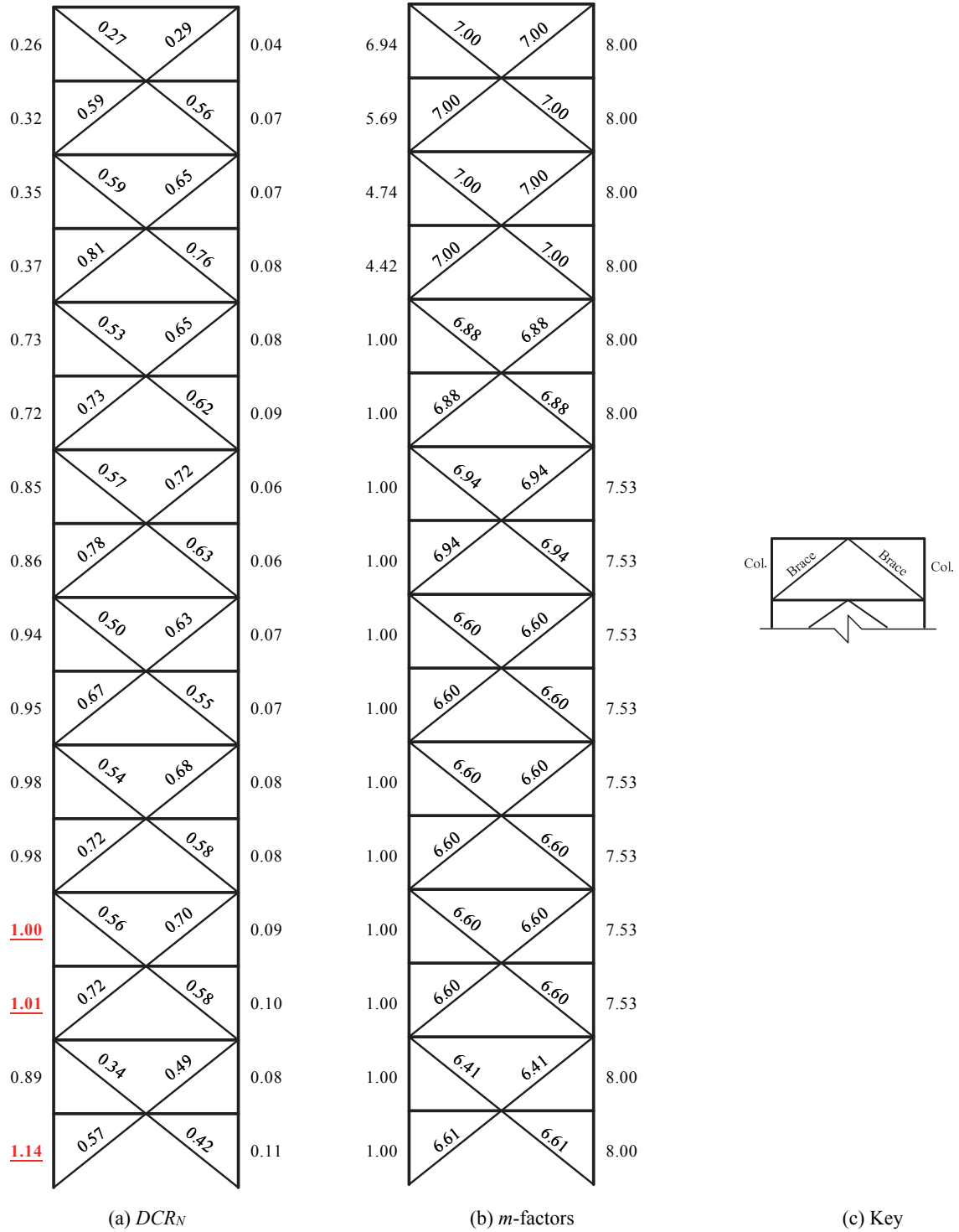
Figure 3-85. LSP Assessment Results, 16-Story SCBF ELF, BSE-2 CP
