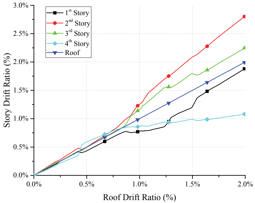
Figure 3-39. 4-Story SCBF RSA Pushover – Story Drift Ratios – BSE-2
