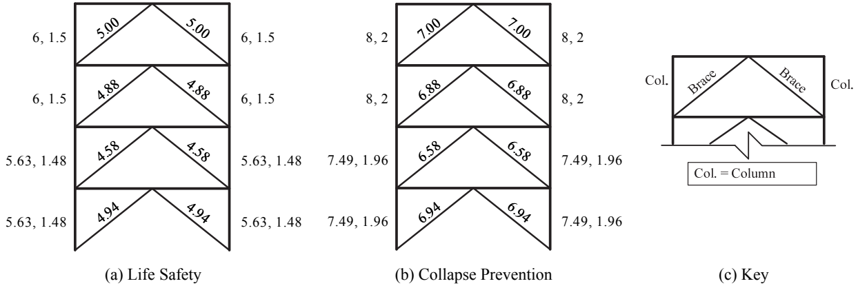
Figure 3-7. Frame Capacity Schematic ( m -factor), LS and CP, 4-Story SCBF ELF
