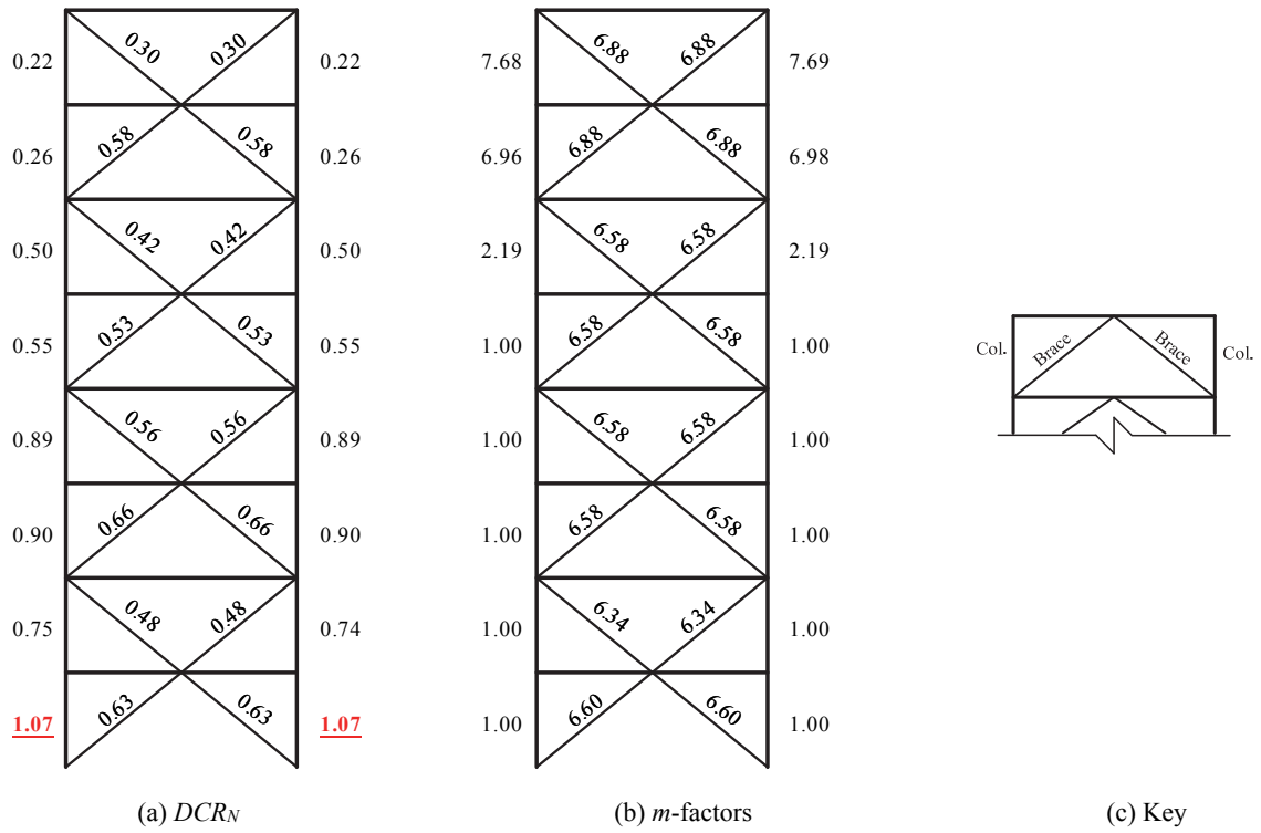
Figure 3-56. LSP Assessment Results, 8-Story SCBF ELF, BSE-2 CP
