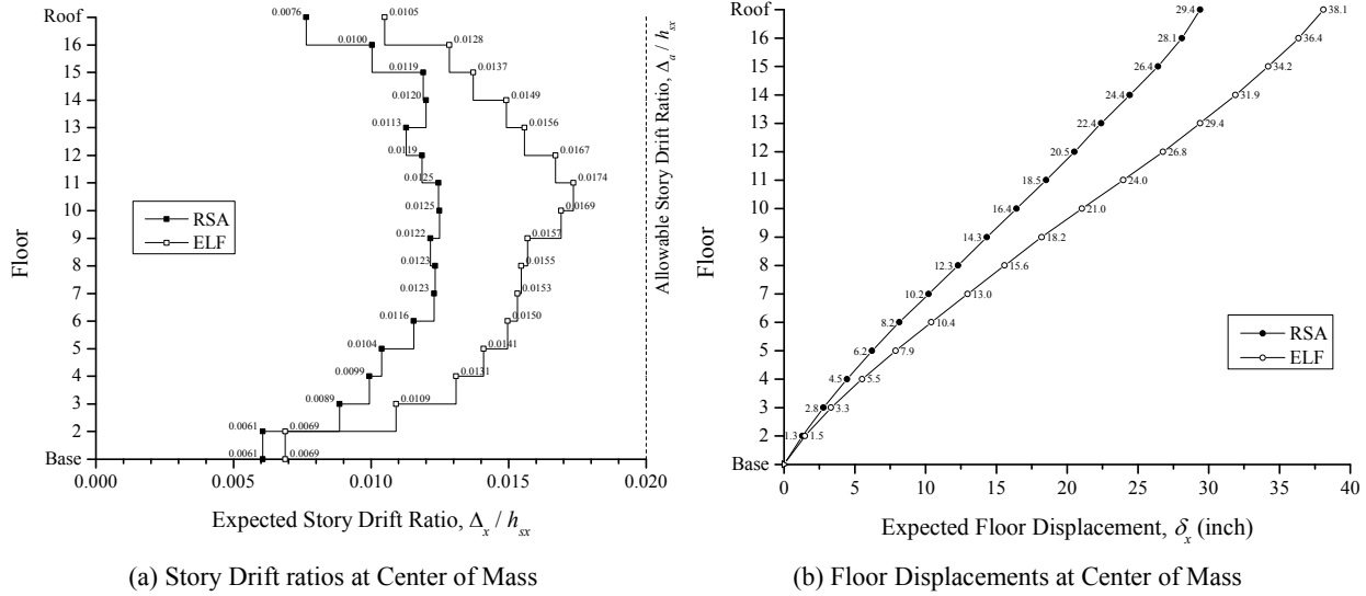
Figure B-9. Story Drift Ratios and Deflected Shape
