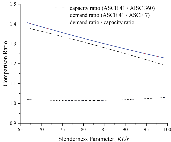
Figure 3-111. Effect of Design and Assessment Provisions on the DCR_N
