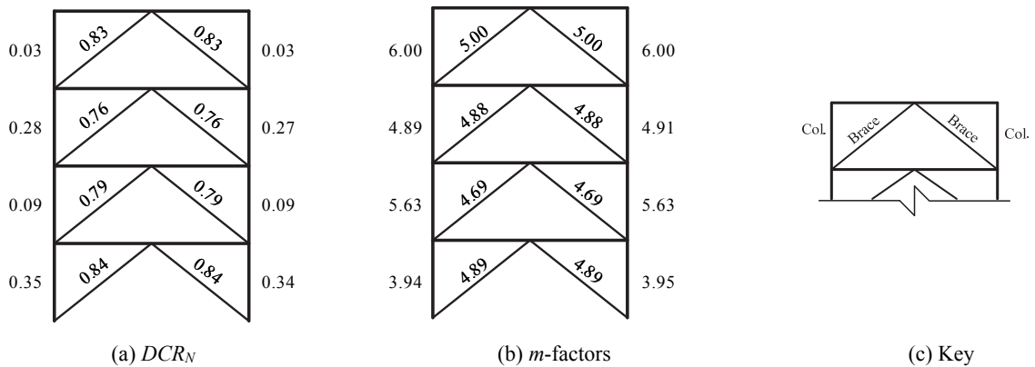
Figure 3-25. LSP Assessment Results, 4-Story SCBF RSA, BSE-1 LS
