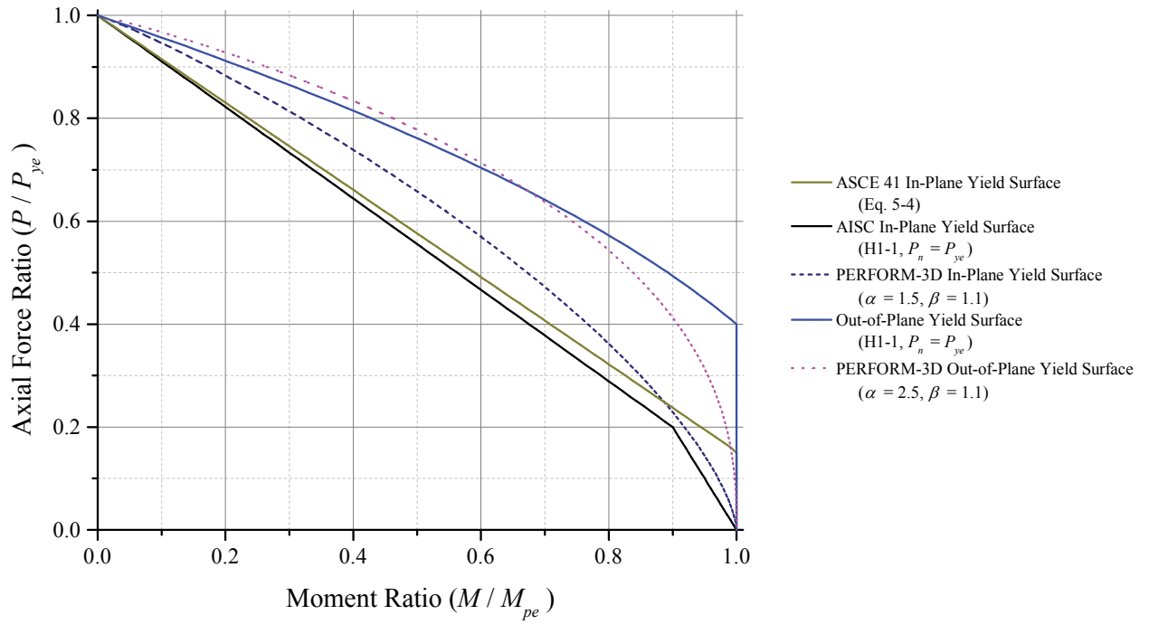
Figure 3-18. P-M Interaction Curve (Section Yield Surface)
