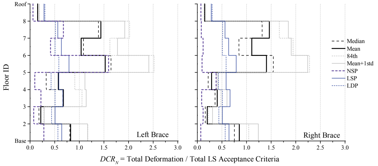
Figure 3-75. NDP Assessment Results, Brace Struts, 8-Story SCBF RSA, BSE-1 LS
