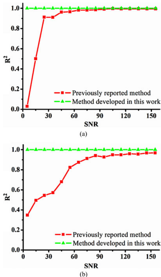
Fig. 8. Comparison of R^2 values as a function of SNR by using two different demodulation schemes (spectrum curve fitting and one peak tracking of the filtered spectrum) for cavity lengths: (a) 60 \mu\text{m} and (b) 300 \mu\text{m} . SNR was calculated as the signal power divided by the noise power.
