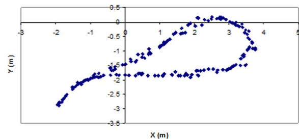
Fig. 4. Operator path through the shared workspace using a LADAR-based tracking system from [5]. Lateral position offsets are due to sensor noise and errors in centroid fitting.
