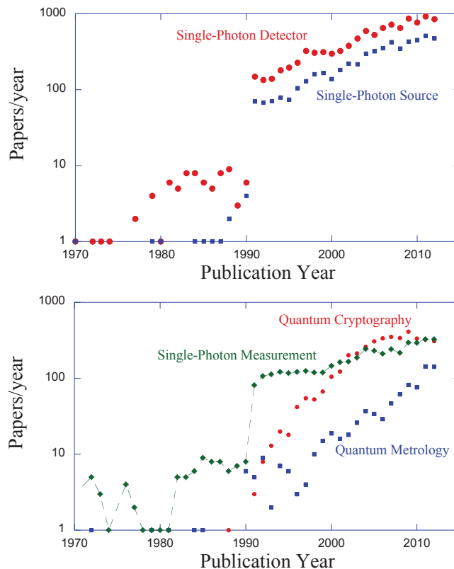
FIG. 1: Growth of the field of single-photon source and detector technology as seen by the number of papers published each year using the indicated search terms in the publication database Web of Science [17]. Search terms: (a) “single-photon source” and “single-photon detector,” (b) “single-photon measurement,” “quantum cryptography,” and “quantum metrology.” Note: The jump in the data at 1990 is an artifact due to the database methodology rather than an indication of a real change in the publication rates.
