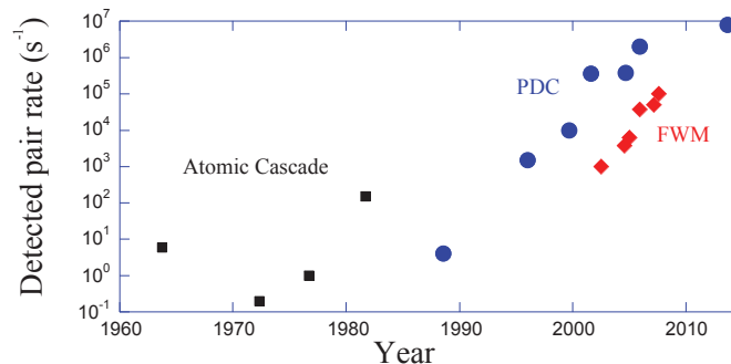
FIG. 2: Detected photon-pair-rate progress. Detected photon pair rates shown for atomic-cascade- (black squares), parametric-down-conversion- (blues dots), and fiber-four-wave-mixing-based sources (red diamonds) [6, 7, 9, 27–35].
