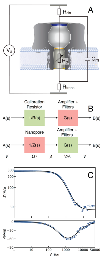
Figure 1. (A) Equivalent circuit model of the nanopore system. The nanopore and membrane are modeled as a resistor ( R_p ) and capacitor ( C_m ) in parallel, together with the total solution and access resistances on either side of the membrane ( R_{cis} and R_{trans} ). (B) The nanopore impedance is measured after removing artifacts from the measurement apparatus. First, the transfer function of the measurement apparatus is determined from the response ( B(s) ) of a 300\text{ M}\Omega calibration resistor to a swept sinusoidal voltage ( A(s) ) stimulus (top). Assuming the resistor frequency response is flat, G(s) = (B(s)/A(s)) R(s) , where G(s) and R(s) are the transfer functions of the measurement apparatus and the calibration resistor respectively. The corrected nanopore impedance was then determined in an identical manner (bottom) to yield Z(s) = G(s)/(B(s)/A(s)) . (C) The equivalent circuit model was validated by measuring the impedance of the nanopore–membrane complex as a function of frequency (blue markers). A least-squares fit (black) of eq 1 to the measured data yielded estimates of R_p = 255\text{ M}\Omega , R_{cis} = R_{trans} = 14\text{ M}\Omega , and C_m = 1.6\text{ pF} .
