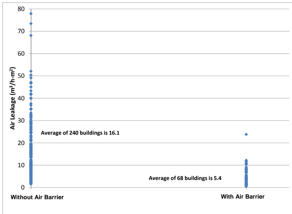
Figure 2 Normalized building air leakage (6-sided enclosure) of buildings with and without air barrier
