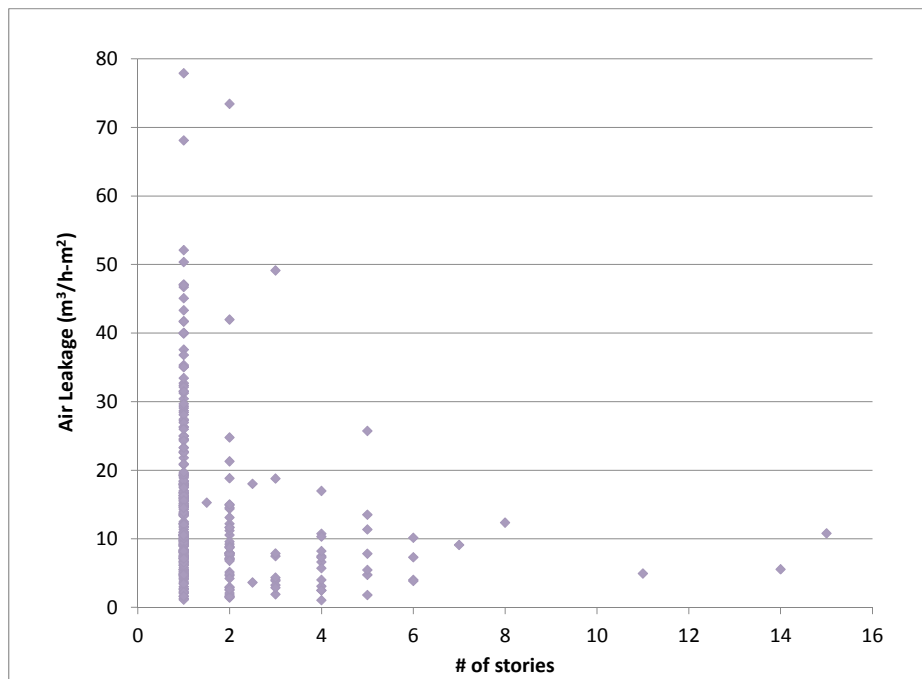
Figure 1: Normalized building air leakage versus height of building (in stories)
