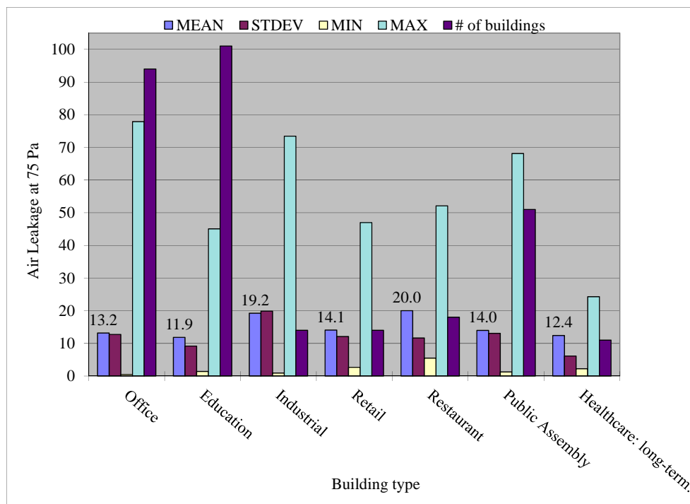
Figure 4: Normalized building air leakage versus Building type
