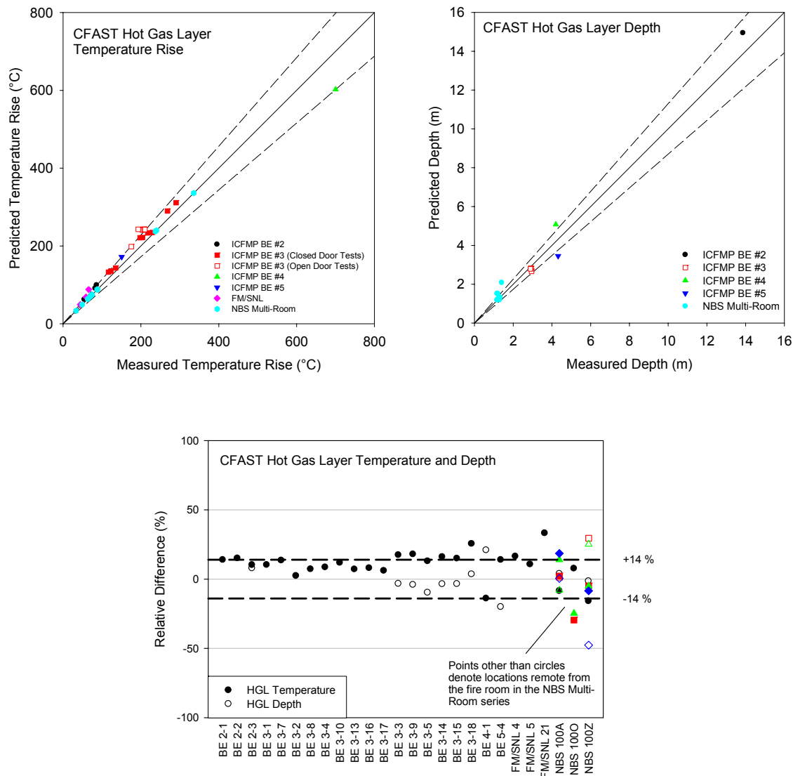
Figure 6-1. Comparisons and Relative Differences for Hot Gas Layer (HGL) Temperature and Height
