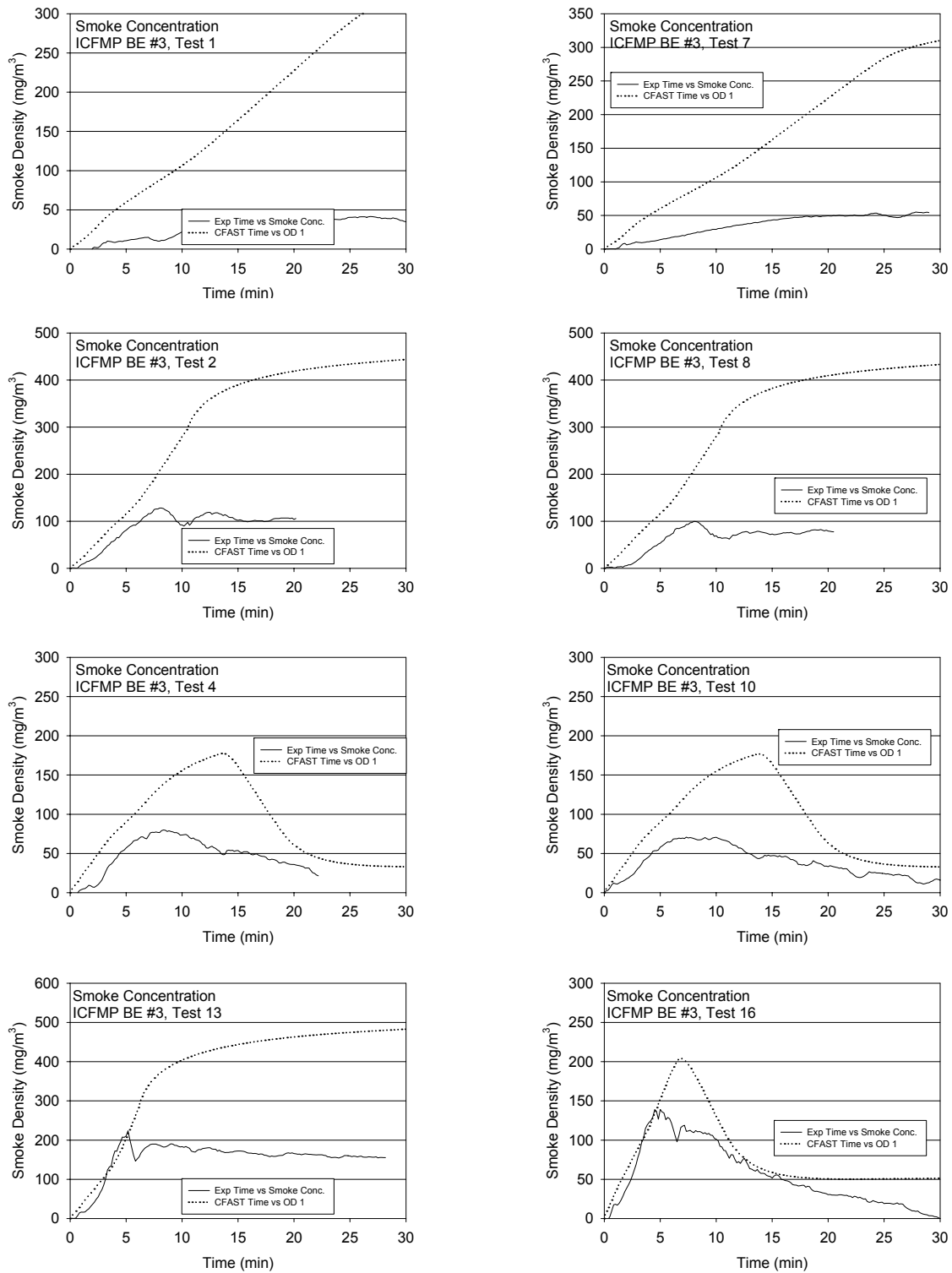
Figure A-26. Smoke Concentration, ICMP BE #3, Closed-Door Tests
