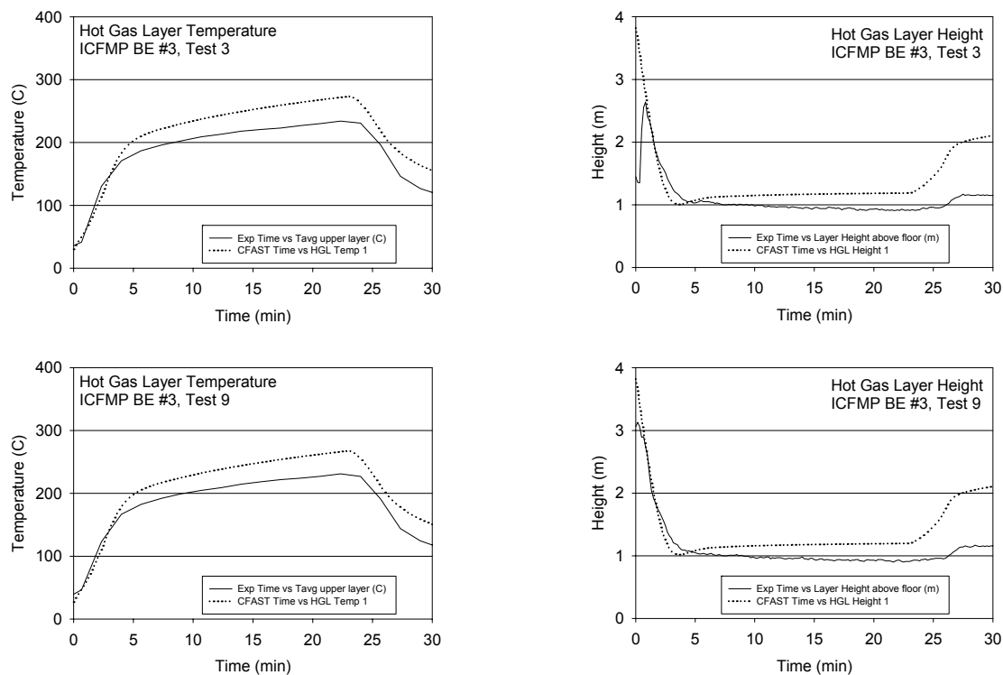
Figure A-6. Hot Gas Layer (HGL) Temperature and Height, ICFMP BE #3, Open-Door Tests
