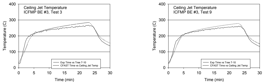
Figure A-19. Ceiling Jet Temperature, ICFMP BE #3, Closed-Door Tests
