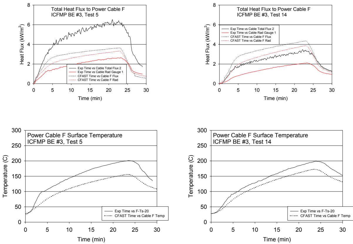
Figure A-49. Thermal Environment near Power Cable F, ICFMP BE #3, Tests 5 and 14
