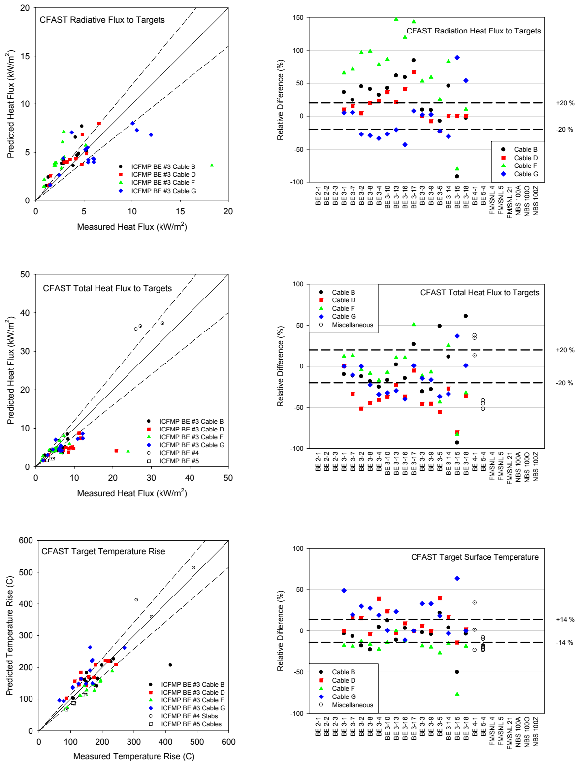
Figure 6-6. Comparisons and Relative Differences for Heat Flux to Targets and Target Temperature
