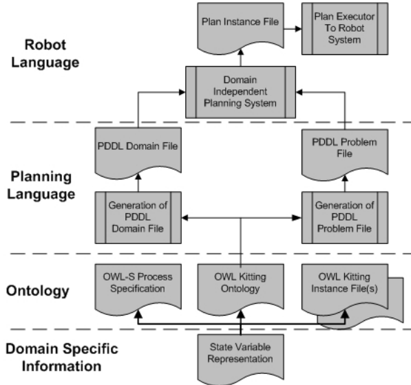
Fig. 1. Kitting data flow abstraction.
