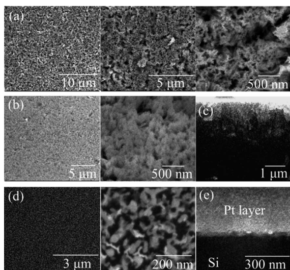
Fig. 7 (a) Top down view and (b) 52° view of strongly corrugated silicon (referred to as 1.6 μm MaCE in the paper), (c) side-view of cleaved strongly corrugated silicon, and (d) top down and (e) 52° view of Focus Ion Beam cross-section of lightly corrugated silicon (referred to as 100 nm MaCE in the paper).
