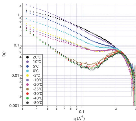
Fig. 2 SANS from lysozyme in 0.4\text{ M NaCl } D_2O solution as a function of temperature. Error bars represent plus and minus the combined standard uncertainty of the data collection.
