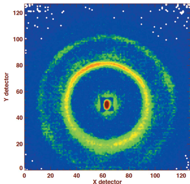
Figure 1 The two-dimensional neutron scattering pattern from opal taken at a wavelength of 10 Å, showing the variation in the resolution of the 111 peak. The weak second diffraction peak at a scattering vector that is (8/3)^{1/2} \approx 1.61 times that of the first-order peak is consistent with a system of close-packed lattice of noncrystalline silica spheres (Sosnowska & Shiojiri, 1999). (The incident beam without the sample is superimposed on the beam stop.)
