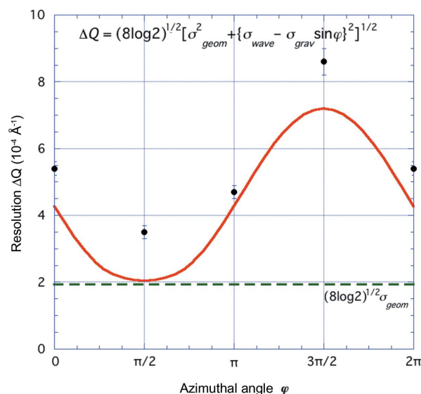
Figure 2 The variation of the FWHM of the diffraction peak for opal using \lambda = 10 Å neutrons as a function of azimuthal angle \varphi . The line is the calculation and the points are the measured data. Both are averaged over 20^\circ . The statistical error bars correspond to one standard deviation.
