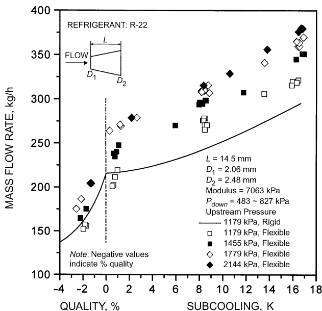
Figure 4. Comparison of Flow Rate of Flexible Short Tube to that of Rigid Short Tube
