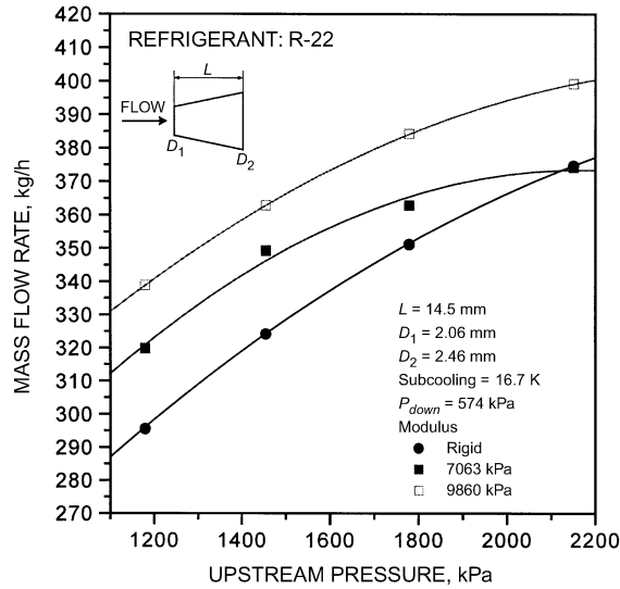
Figure 3. Effect of Upstream (Condensing) Pressure and Modulus of Elasticity at Subcooling of 16.7 K
