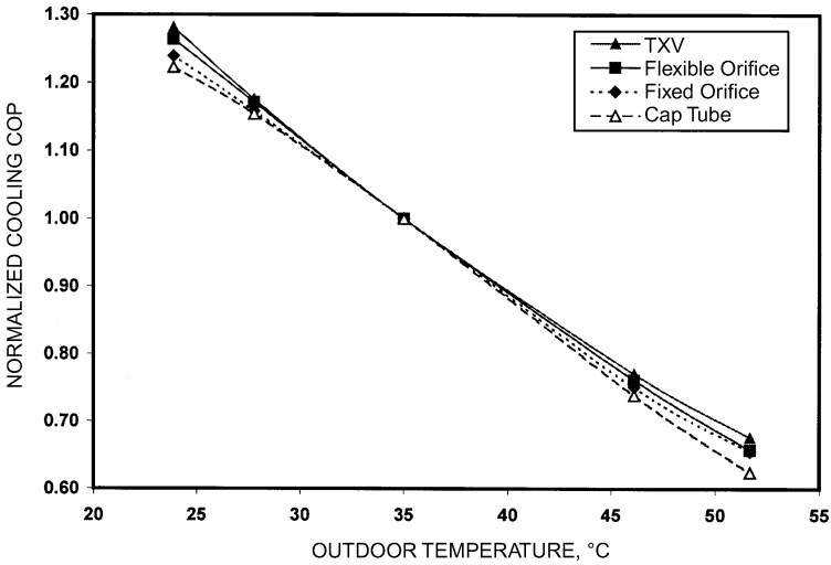
Figure 6. Normalized Cooling COP for Window Air Conditioner as Function of Outdoor Temperature for Four Expansion Devices
