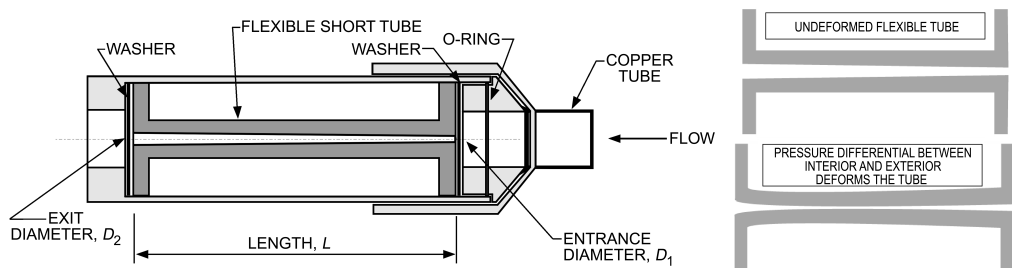
Figure 2. Schematic of Flexible Short-Tube Test Section
