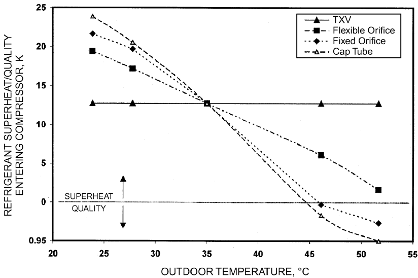
Figure 7. Refrigerant Superheat/Quality Entering Compressor
