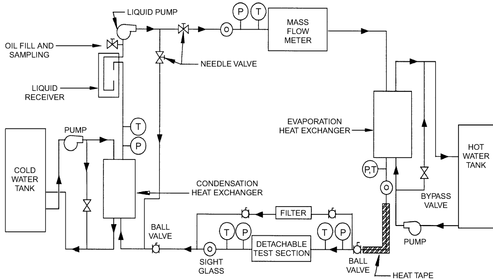
Figure 1. Schematic Diagram of Flexible Short-Tube Test Setup
