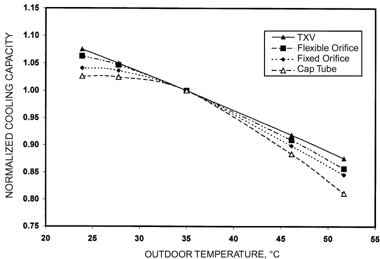
Figure 8. Estimated Normalized Cooling Capacity for Window Air Conditioner as Function of Outdoor Temperature for Four Expansion Devices
