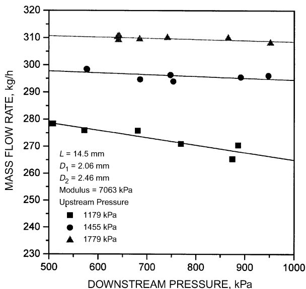
Figure 5. Effect of Downstream (Evaporating) Pressure on Flow Rate for Flexible Short Tube with Modulus of 7063 kPa
