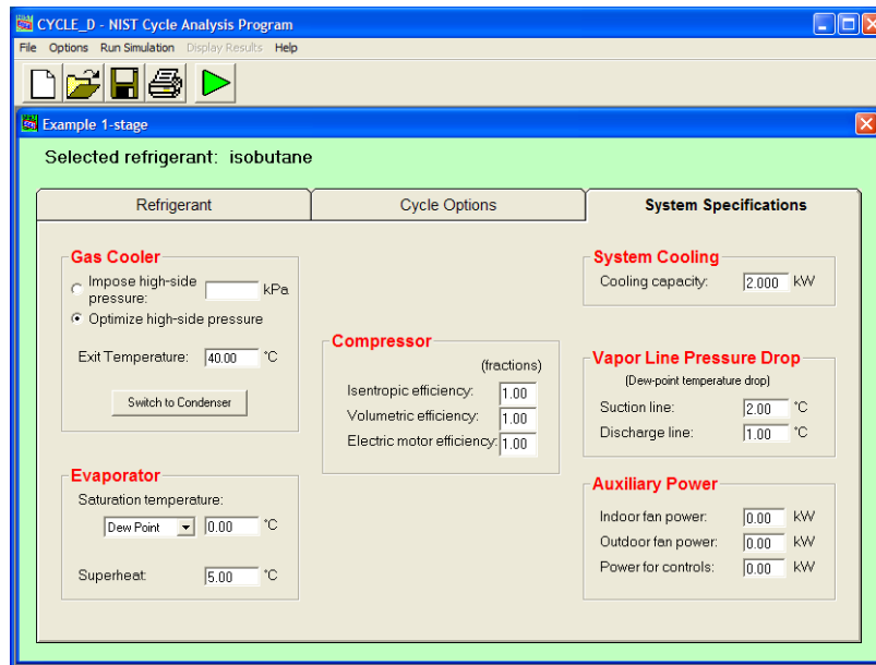
Figure 13. System Specifications tab for a single-stage, transcritical cycle and optimization option selected for the gas cooler pressure
