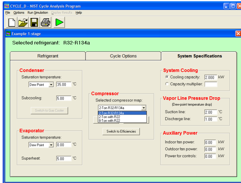
Figure 12. System Specifications tab for a single-stage, subcritical cycle and map-based representation of the compressor
