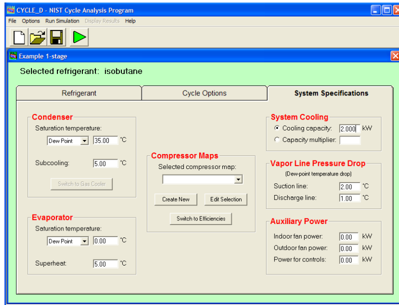
Figure C1. System Specifications tab showing the Create New and Edit Selection compressor map options after a click on the Switch to Maps key
