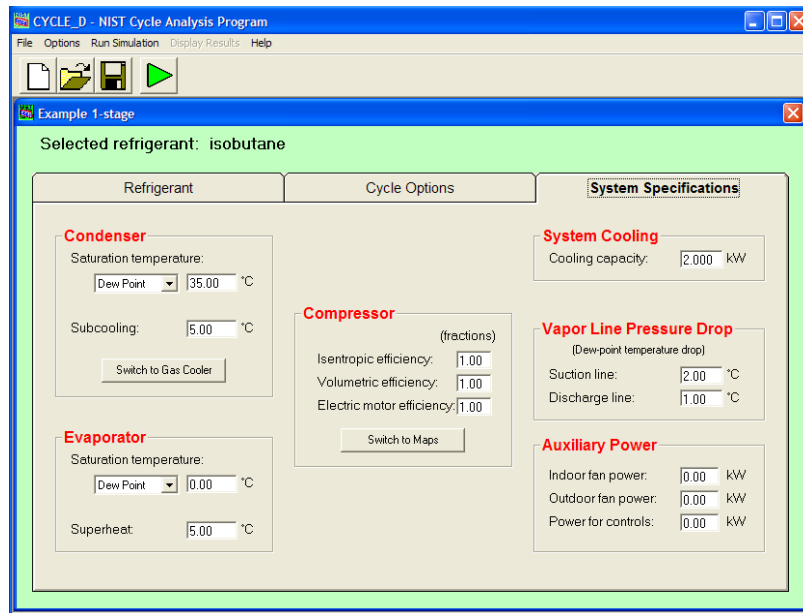
Figure 11. System Specifications tab for a single-stage, subcritical cycle and efficiency-based representation of the compressor
