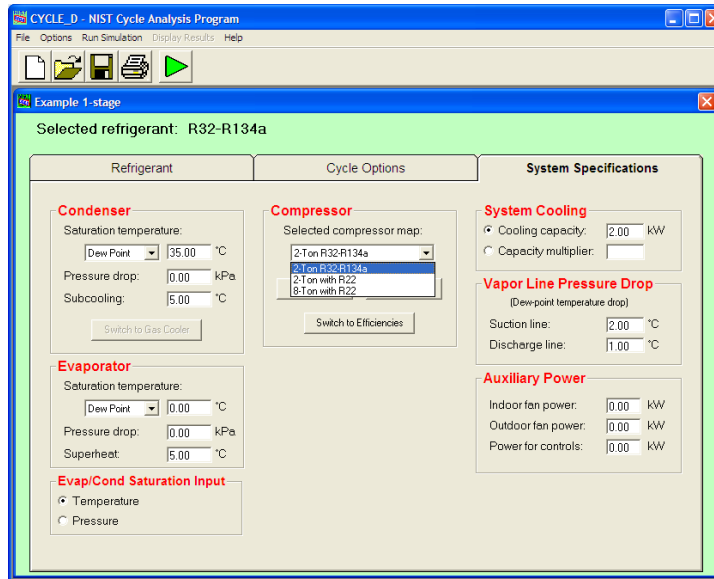
Figure 12. System Specifications tab for a single-stage, subcritical cycle and map-based representation of the compressor
