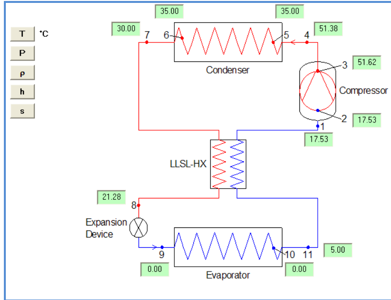
Figure 16. System schematic window
