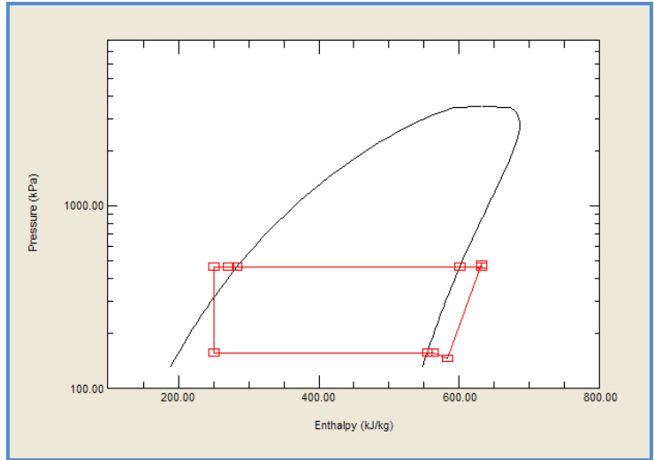
Figure 16. P-h state diagram
