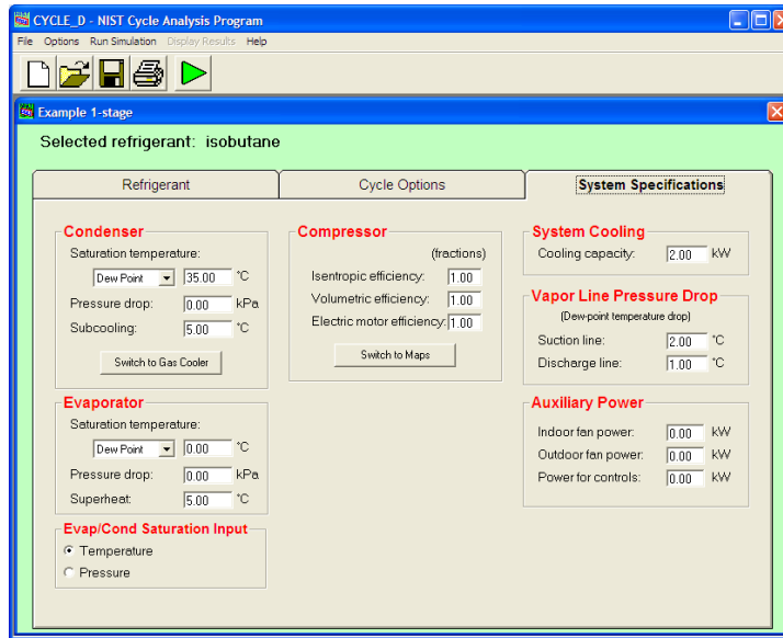
Figure 11. System Specifications tab for a single-stage, subcritical cycle and efficiency-based representation of the compressor
