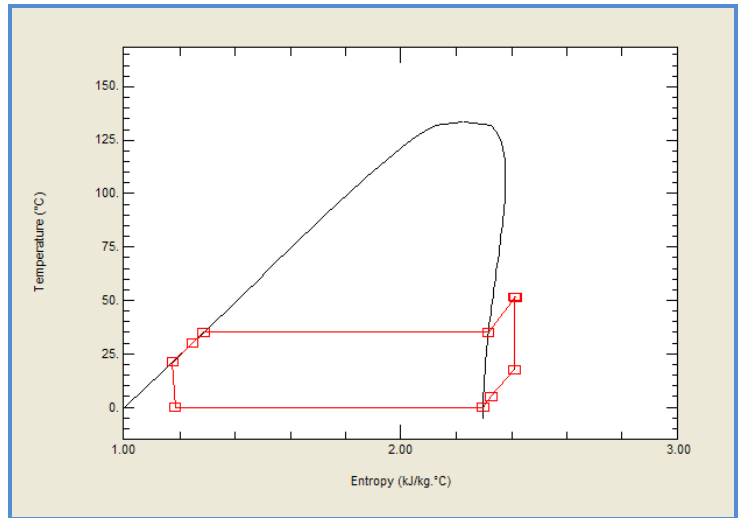
Figure 17. T-s state diagram
