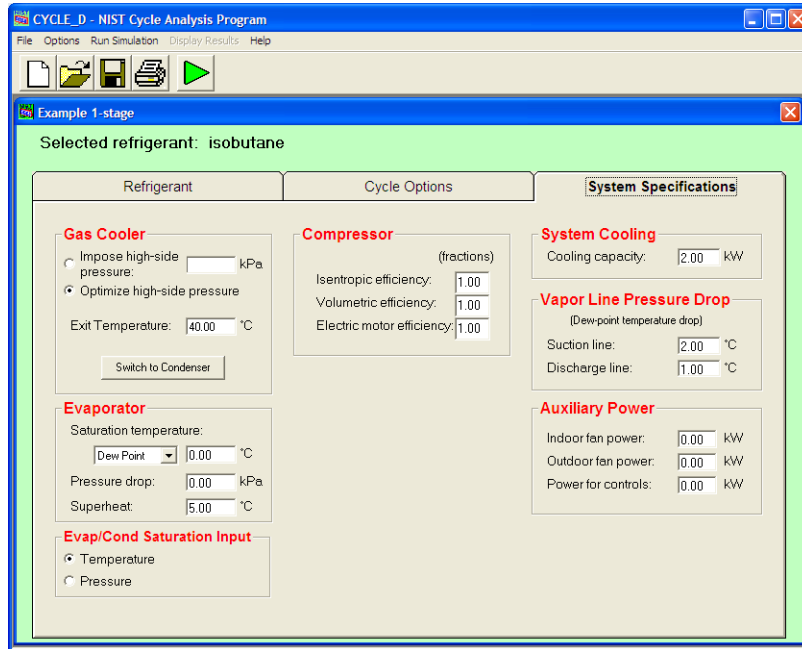
Figure 13. System Specifications tab for a single-stage, transcritical cycle and optimization option selected for the gas cooler pressure
