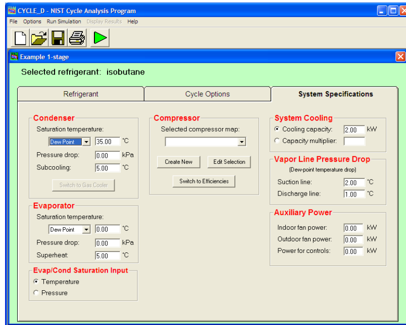
Figure C1. System Specifications tab showing the Create New and Edit Selection compressor map options after a click on the Switch to Maps button
