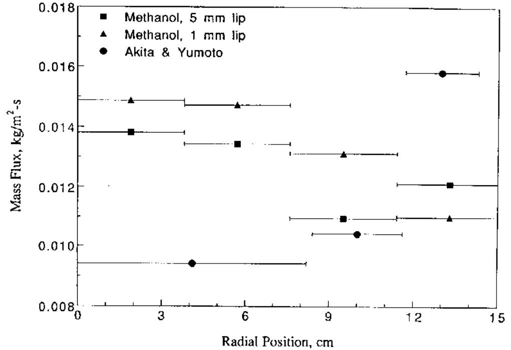
FIGURE 17 Mass burning rates as a function of radial location for methyl alcohol burning in a 0.30 m ring pool with 0.1 and 0.5 cm lip heights. Also shown are results reported by Akita and Yumoto (1965).
