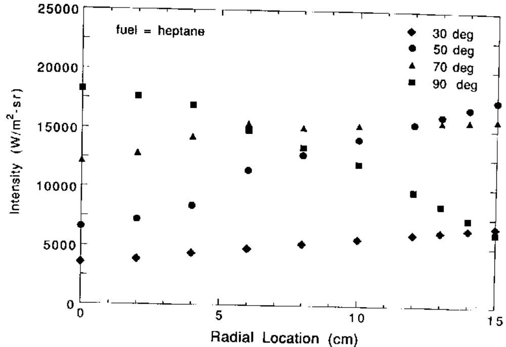
FIGURE 9 The time-averaged radiative intensity as a function of radial location on the surface of the 0.30 m pool burning heptane for directions defined by \phi = 90^\circ and \Theta = 30^\circ, 50^\circ, 70^\circ , and 90^\circ . The center of the pool is indicated by the 0 cm position.
