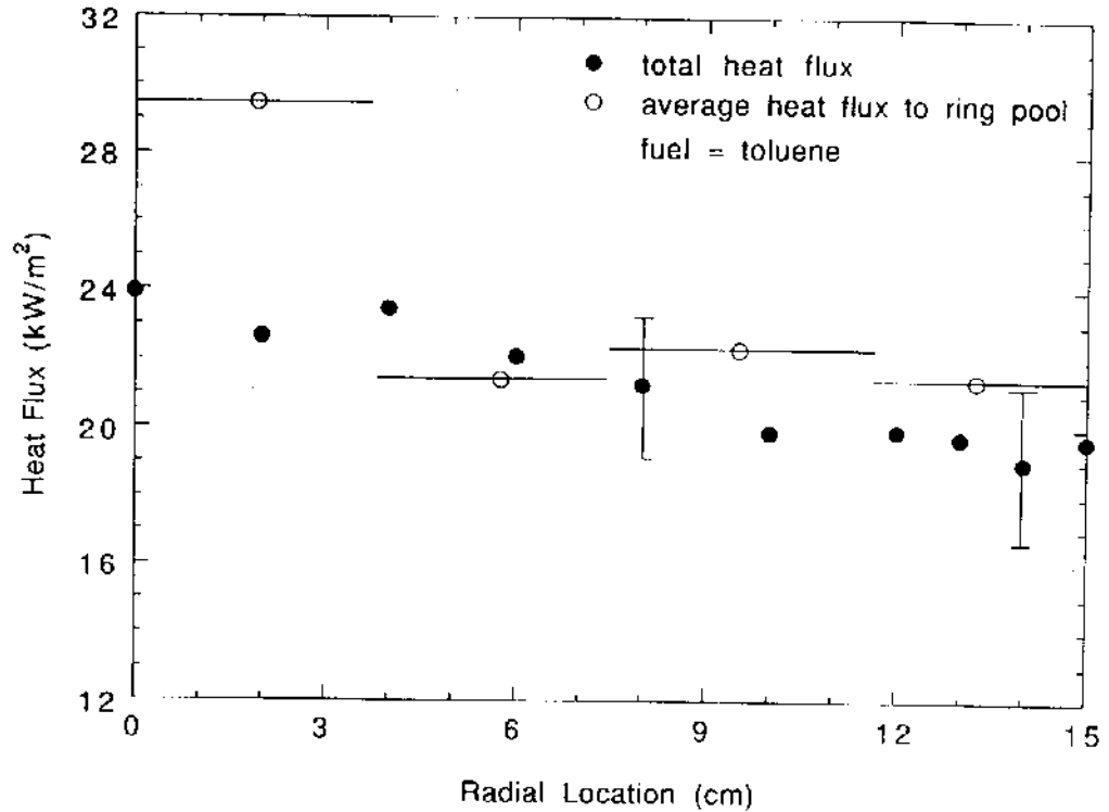
FIGURE 15 Local heat feedback measurement as a function of radial location for a 0.30 m pool fire burning toluene. Also shown are the net heat feedback calculated from mass burning rates in annular rings (see Fig. 13). The lateral extent of the rings are denoted by the horizontal bars.
