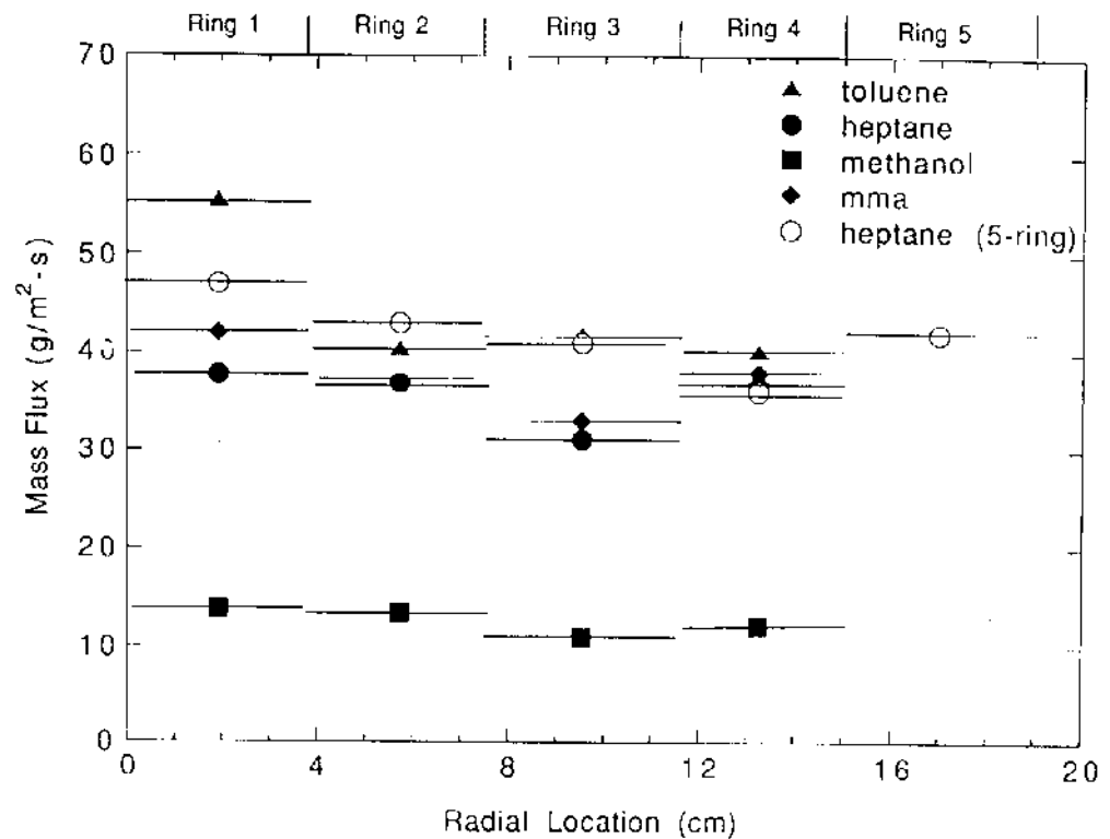
FIGURE 13 Time-averaged mass burning rate as a function of ring location for pool fires burning methyl alcohol, MMA, toluene, and heptane in a four-ring and heptane in a five-ring pool.
