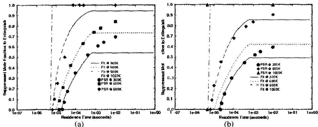
Figure 1. Blowout suppressant mole fraction vs. residence time for stoichiometric H_2/air mixtures with (a) N_2 (in excess of air) and (b) H_2O suppressants at 1 atm pressure. Symbols are from PSR-CHEMKIN calculations and lines are curve fits.
