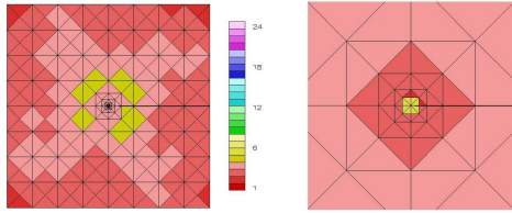
Figure 225: Example grid for the REFSOLN_EDGE strategy with the mode 2 linear elasticity problem, including details at the singularity.
