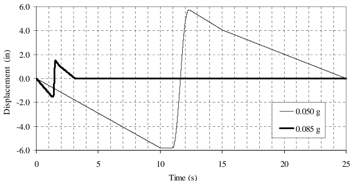
Figure 2–49. Displacement history inputs for tests 4 and 5.
