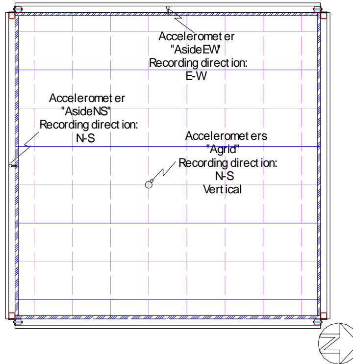
Figure 2-11c. Locations of the accelerometers on the ceiling support grid.
