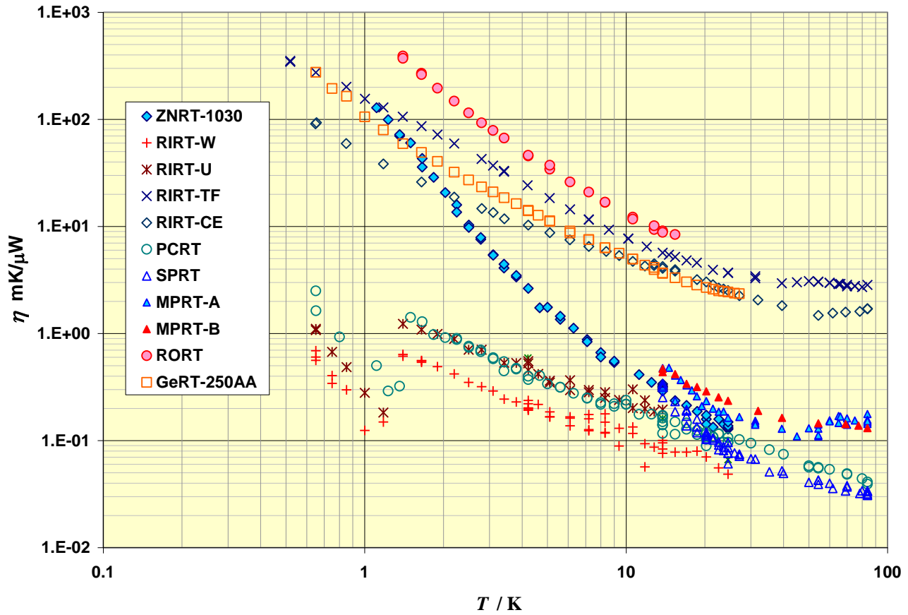
Figure 1.5 . The self-heating coefficient \eta(T) over the range 0.5 K to 84 K for a sample of cryogenic resistance thermometers as measured under vacuum: ZNRT-1030 , Lakeshore model CX-1030-AA; RIRT-W and -U, Tinsley model 5187-W and -U; RIRT-TF, Lakeshore model RF-100-AA; RIRT-CE, Lakeshore model RF-800 ;PCRT, Chino model R-800-4; SPRT, Leeds & Northrup model 8164; MPRT-A and -B, Minco model S1059; RORT, custom 10 k \Omega TFCR bonded to copper strip; GeRT-250AA, Lakeshore model GR-200-A-250.
