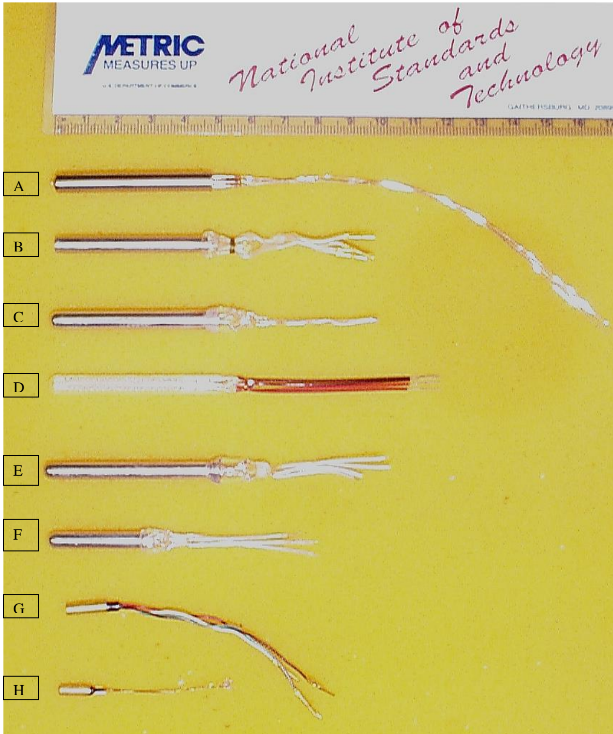
Figure 1.8 Various commercial designs of capsule type SPRTs, RIRTs, PCRTs, and GeRTs: A. 5.7 OD SPRT with inconel outer sheath [39, 53 ]; B. 5 mm OD SPRT or PCRT with platinum sheath [54] ; C. 5.5 mm OD platinum sheath SPRT [55] ; D. 5.7 mm OD glass sheath SPRT [56]; E. 5 mm OD SPRT or 100 \Omega RIRT [57] ; F. 5 mm OD 50 \Omega RIRT with platinum sheath [57] ; G. 3.6 mm OD GeRT ; H. 3 mm OD GeRT, also similar packages are used for MPRTs , thin-film RIRTs, ZNRTs, and other common NTC devices.
