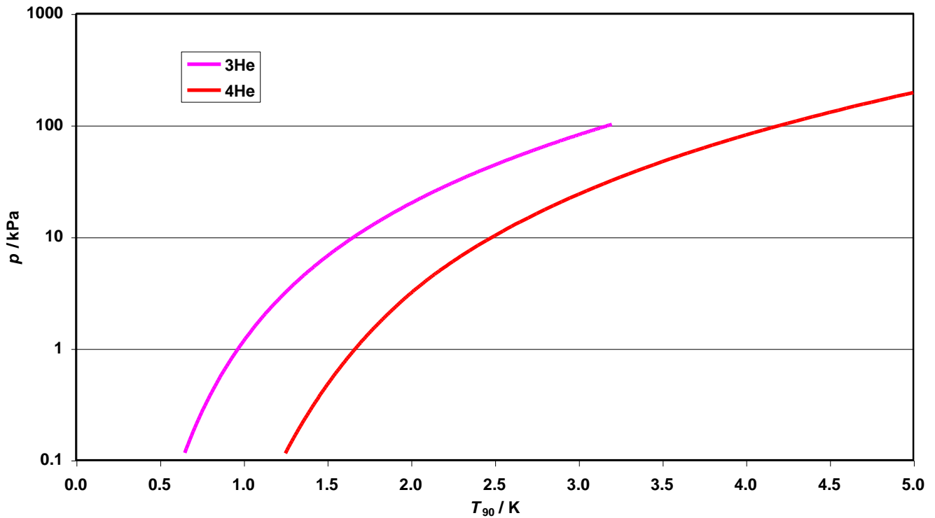
Figure 3.4 The ITS-90 ^3\text{He} and ^4\text{He} vapor pressure curves from 0.65 K to 5.0 K.
