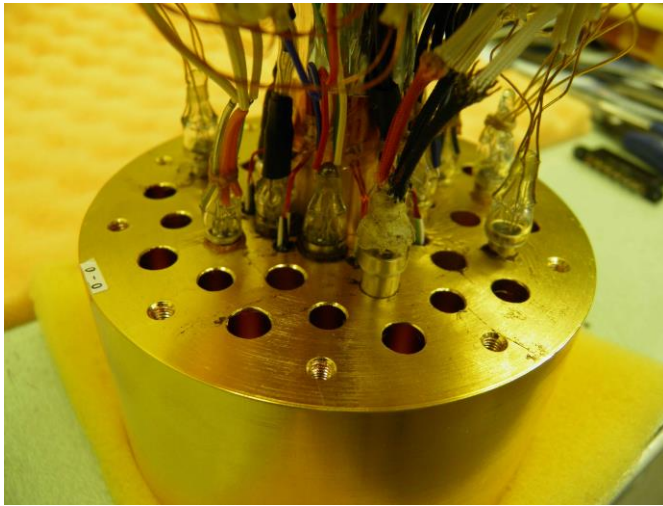
Figure 5.2 A large comparison block with capsule thermometers installed.
