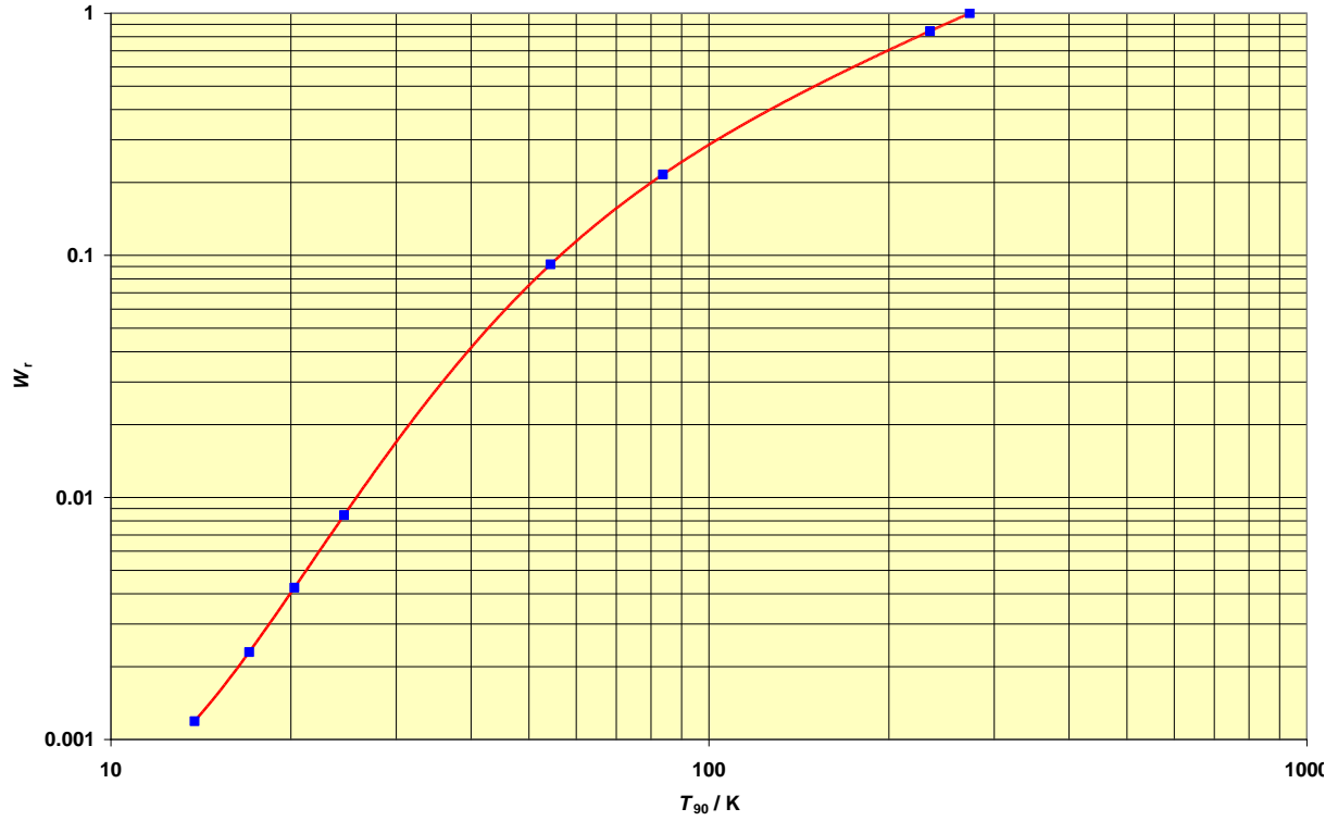
Figure 3.2 The SPRT reference function for T_{90} < 273.16 K. Location of defining fixed points are indicated as square markers on the curve.
