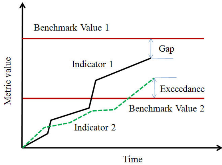
Figure 8. Performance Evaluation
