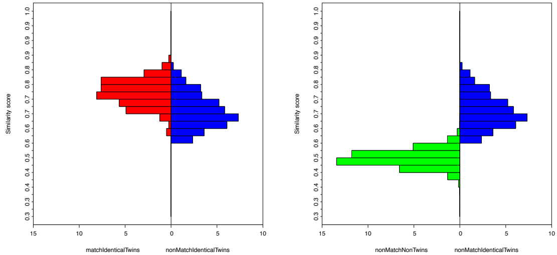
Fig. 8. Back-to-back histograms of the similarity score distributions for Algorithm C for the Ambient-to-ambient lighting and Neutral-to-neutral expression experiment. All three distributions are for face pairs collected on the same day. The distribution for match face pairs is plotted in red in the histogram on the left (labeled 'matchIdenticalTwins' in this Figure). The distribution for non-match pairs for identical twins is plotted in blue in both histograms (labeled 'nonMatchIdenticalTwins'). The distribution for non-match pairs for non-identical twins (standard non-match face pairs) is plotted in green in the histograms on the left (labeled 'nonMatchNonTwins').
