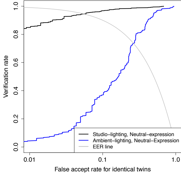
Fig. 3. A ROC showing the extremes in performance for algorithm C for images taken on the same day.
