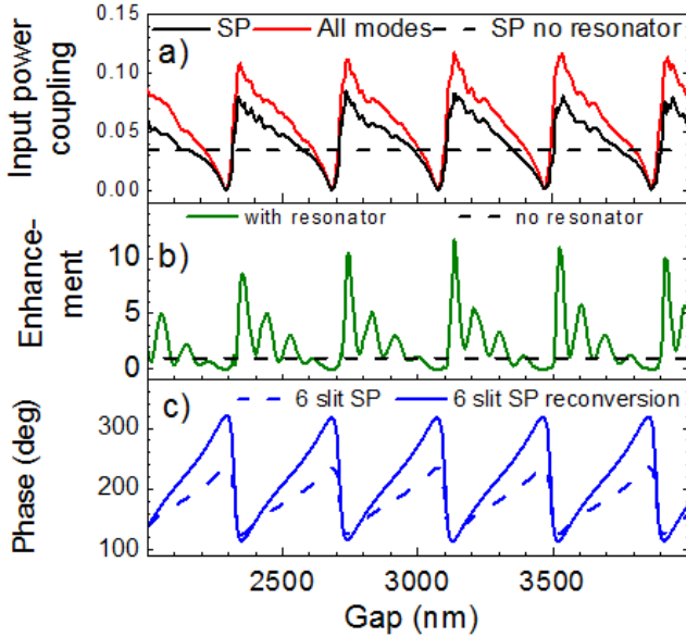
FIG. 3. (a) Optical power coupling through a single grating from a Gaussian incident beam into the SP mode (black) and total lateral power flow from all modes (red) with reflector, as well as coupling into SP mode without a resonator (dashed). (b) Modeled enhancement resulting from two grating couplers with (green) and without (dashed) a resonator and interference between SP and other guided modes. (c) Gap-dependence of the phase variation of SPs produced at a six slit in-coupler and the corresponding phase variation of the reconverted light exiting normal to the film at the out-coupler.
