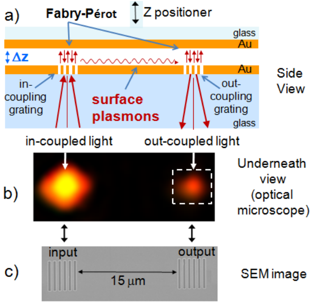
FIG. 1. (a) The top Au reflector moves up and down with respect to the bottom patterned Au film via a piezo positioner. The gratings couple light and SPs. Fabry-Pérot resonance conditions occur above the gratings and are responsible for out-coupled light enhancement. (b) Optical image taken in cross polarization from below (see Fig. 1a) showing input laser (left) and the weaker out-coupled light (dashed box defines integration area). (c) Scanning electron microscope image of Au film gratings.
