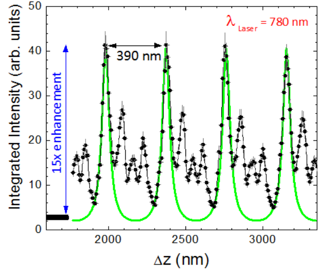
FIG. 2. Integrated intensity of out-coupled light from grating vs. FP resonator separation \Delta z (Fig. 1). Horizontal line (lower left) is the integrated intensity with no resonator ( = 2.8 \pm 0.2 ). The enhancement is the peak intensity ( = 42 \pm 3 ) w/ resonator divided by the intensity w/o resonator and equals 15 \pm 2 . Green curve is a fit to main FP resonance (interference induced side resonances are discussed in text and Fig. 3b) using the function 9 T(\Delta z) = 1/[1 + [4R \sin^2(2\pi\Delta z/\lambda)/(1-R)^2]] for FP transmittance. The fit gives R = 0.63 which is the effective reflectance of the two resonator surfaces. Uncertainty at 95 % confidence level is indicated by error bars and was determined by statistical analysis of both the reproducibility of the z piezo position and stability of the imaging system.
