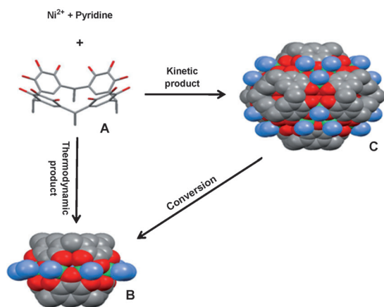
Figure 3. The temperature-dependent synthesis of dimeric (B) and hexameric (C) nickel/copper capsules from pyrogallol[4]arene (A). Addition of Ni/Cu and pyridine to A yields preferentially B or C depending on temperature, metal, and solvent. Propyl groups and pyridine rings are omitted for clarity.
